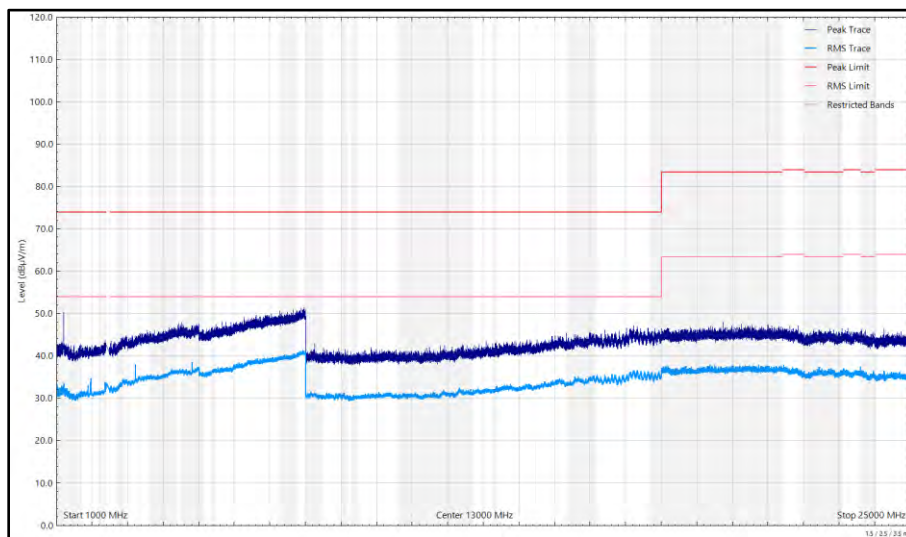
Figure 63 - Ch1_BLE_LE1M - 2404 MHz, 1 GHz to 25 GHz, Horizontal Z Orientation
