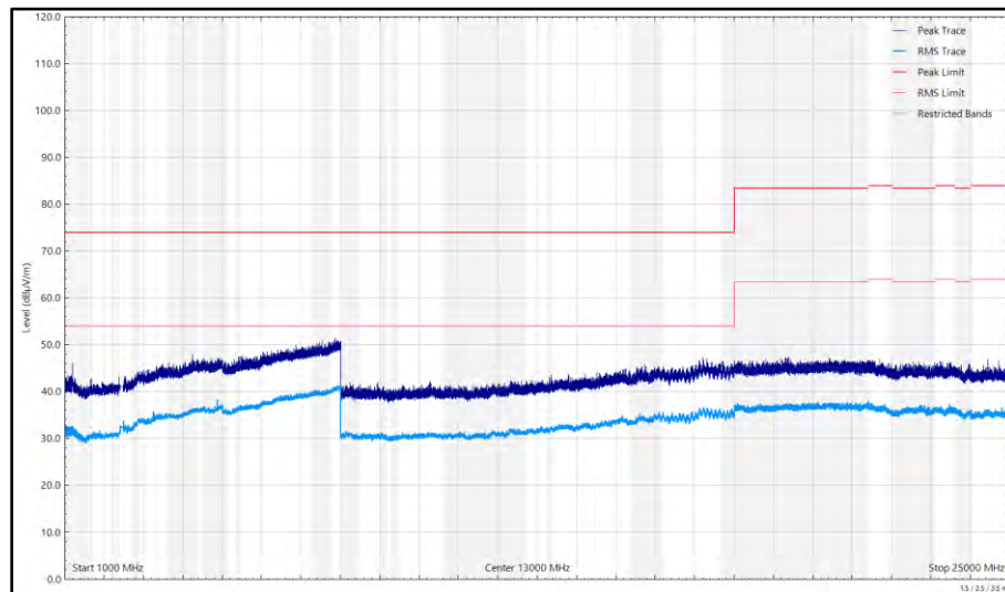
Figure 67 - Ch19_BLE_LE1M - 2440 MHz, 1 GHz to 25 GHz, Horizontal Z Orientation
