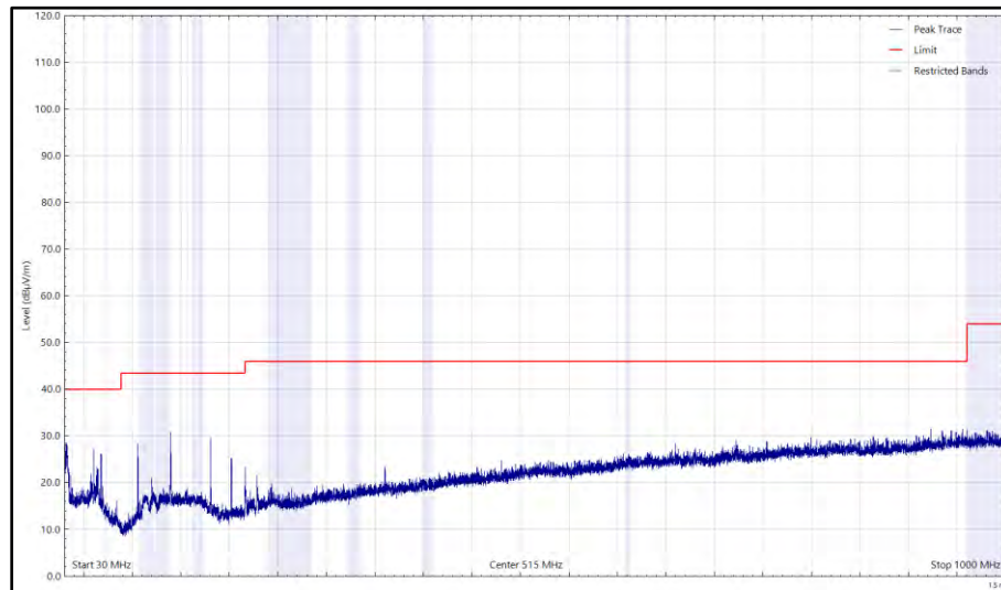
Figure 22 - Top_BLE_LE1M - 2478 MHz, 30 MHz to 1 GHz, Horizontal (Peak) Y Orientation
