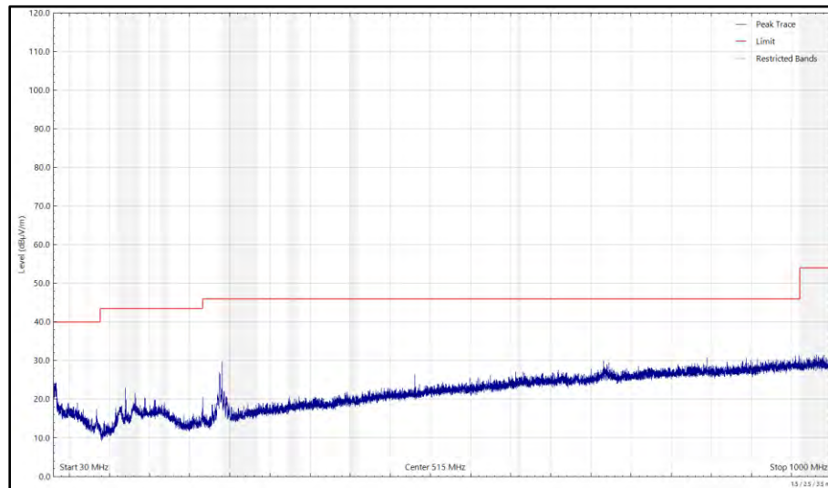
Figure 66 - Ch19_BLE_LE1M - 2440 MHz, 30 MHz to 1 GHz, Horizontal (Peak) Z Orientation
