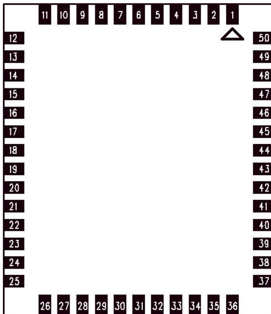
FIG 4 TOP VIEW
