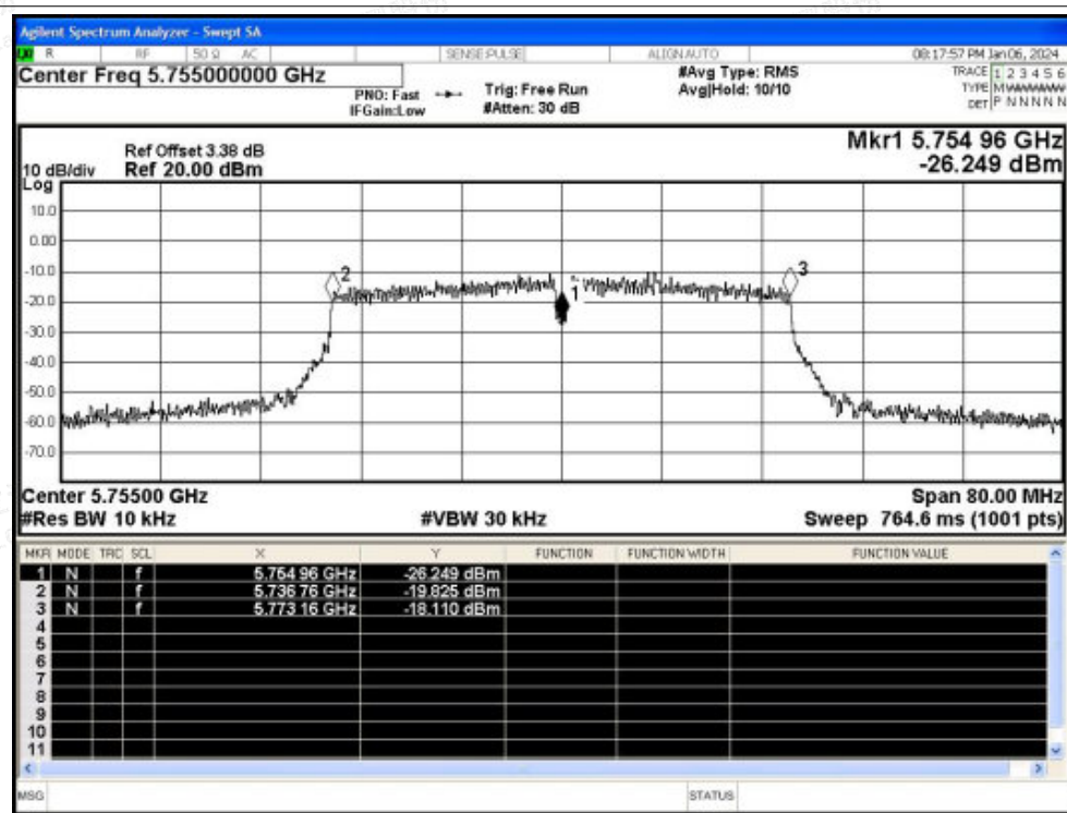
Freq. Stability NVNT ac40 5755MHz Ant3
