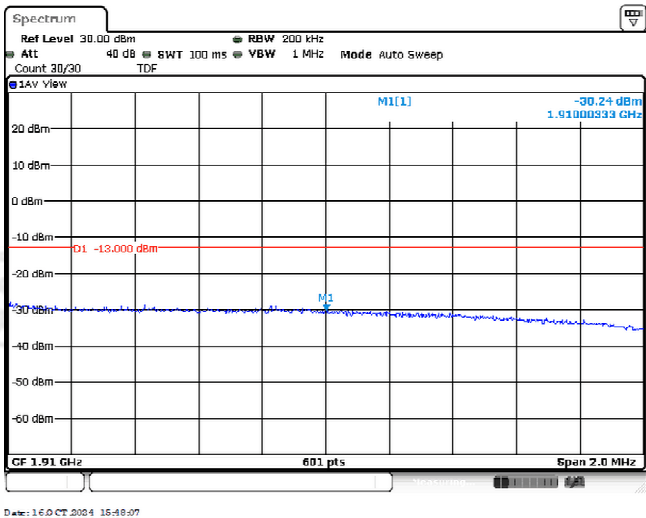
Band2-10MHz-16QAM-19150-1RB#24
