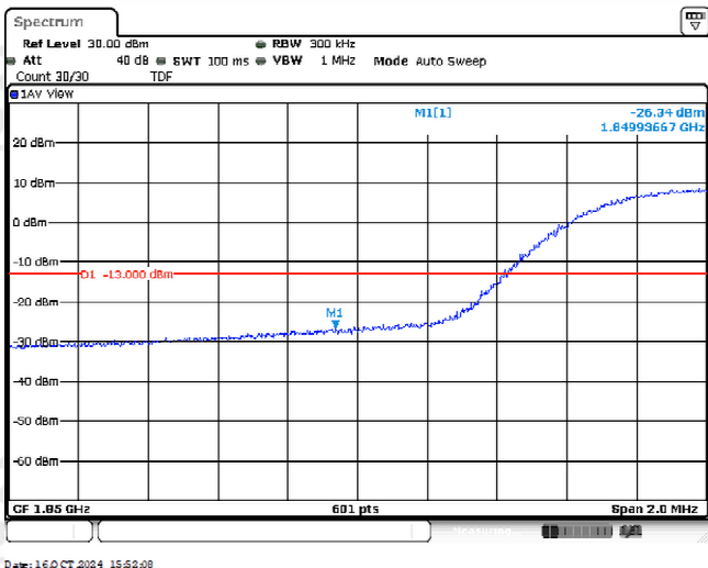
Band2-15MHz-16QAM-18675-25RB#0
