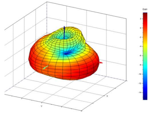
3D Radiation Pattern - Total Gain at 2480 MHz
