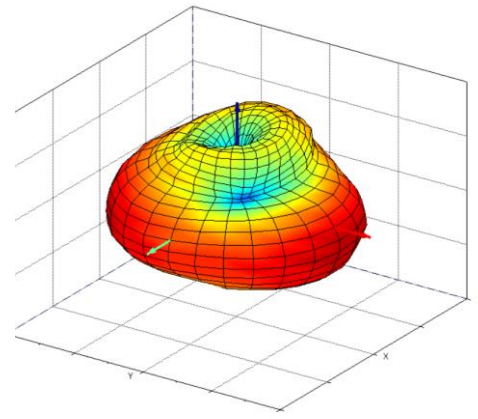
3) 3D Radiation Pattern - Total Gain at 2400 MHz
