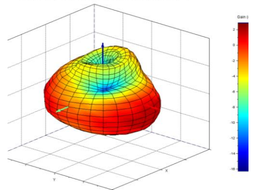
3D Radiation Pattern - Total Gain at 2440 MHz
