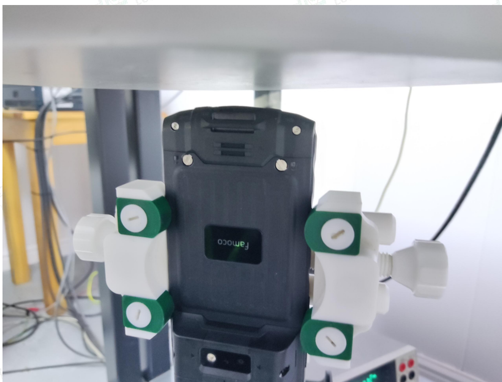
10mm body Vertical-Bottom Side Setup Photo
