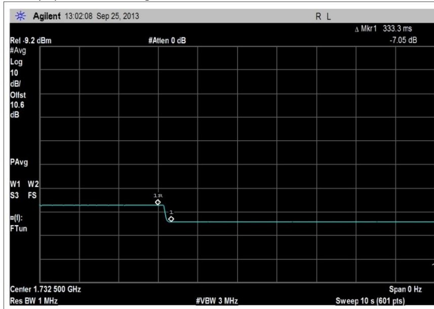
7.7.14 UL Timing_1710-1755MHz
