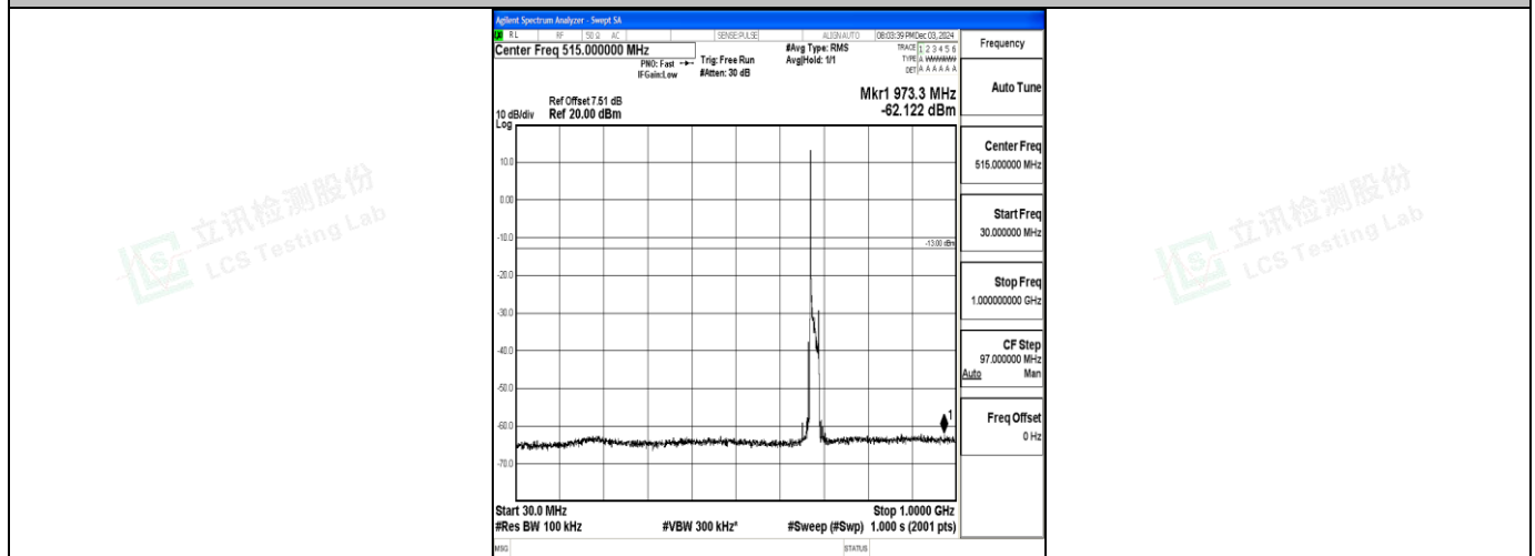
Band71_20MHz_QPSK_133372_1RB#0_30~1000_30~1000
