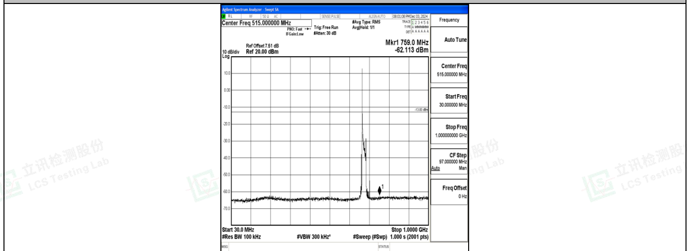
Band71_20MHz_QPSK_133322_1RB#0_30~1000_30~1000
