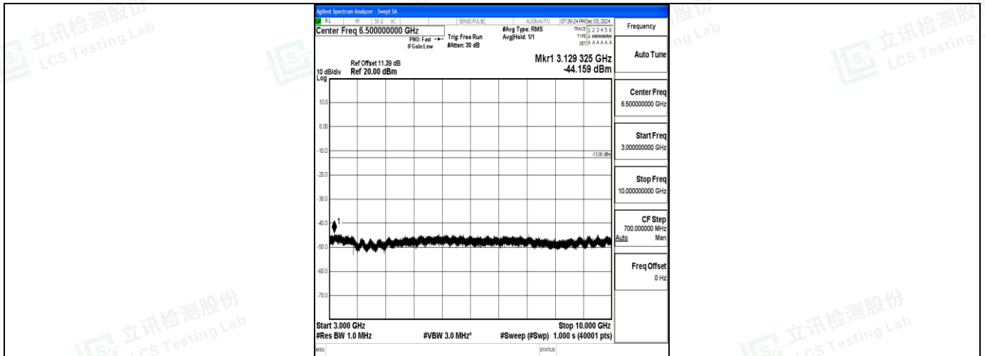
Band71_15MHz_16QAM_133397_1RB#0_3000~10000_3000~10000
