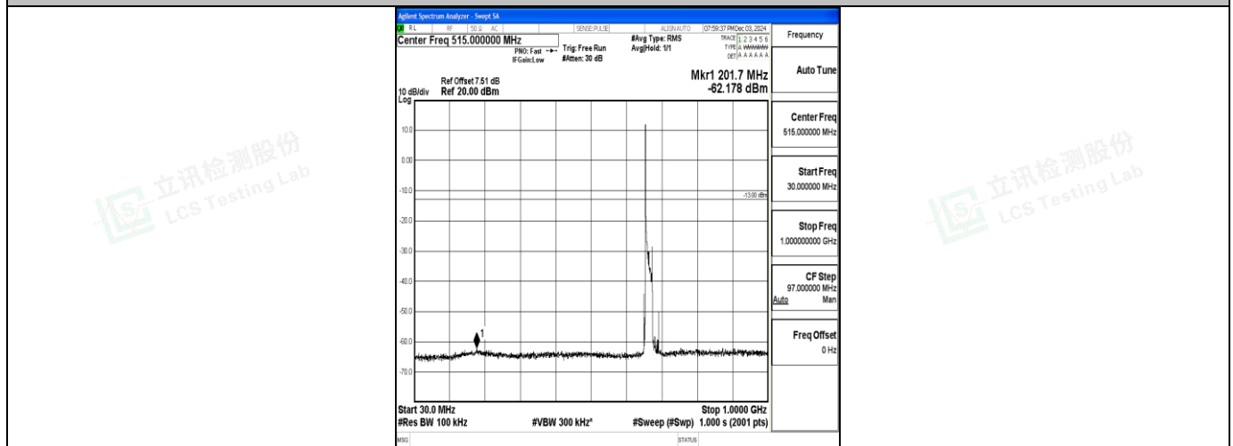
Band71_20MHz_16QAM_133222_1RB#0_30~1000_30~1000
