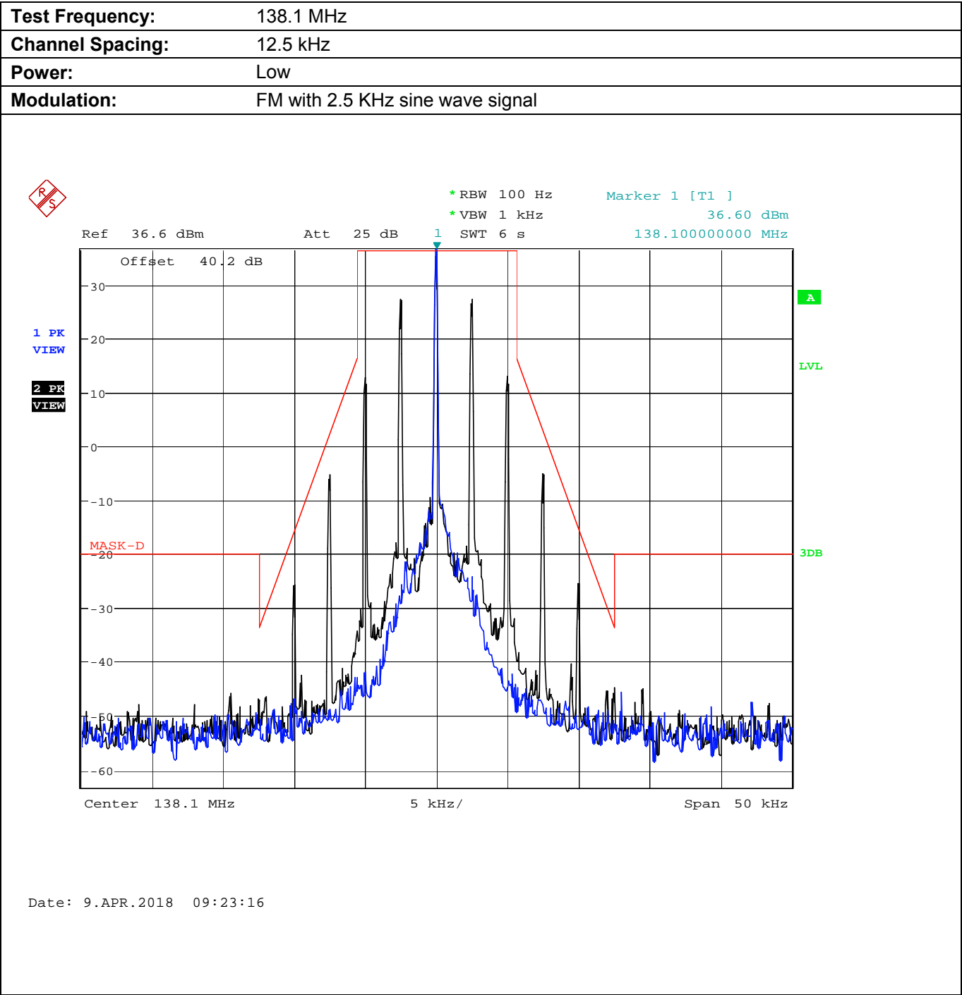
Plot 5.8.4.2.2. Emission Mask D, Low Power
