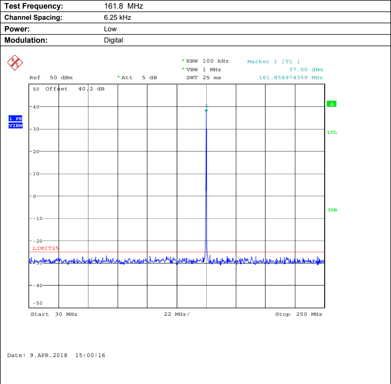
Plot 5.9.4.3.2. Conducted Transmitter Spurious Emissions for 161.8 MHz, Low Power
