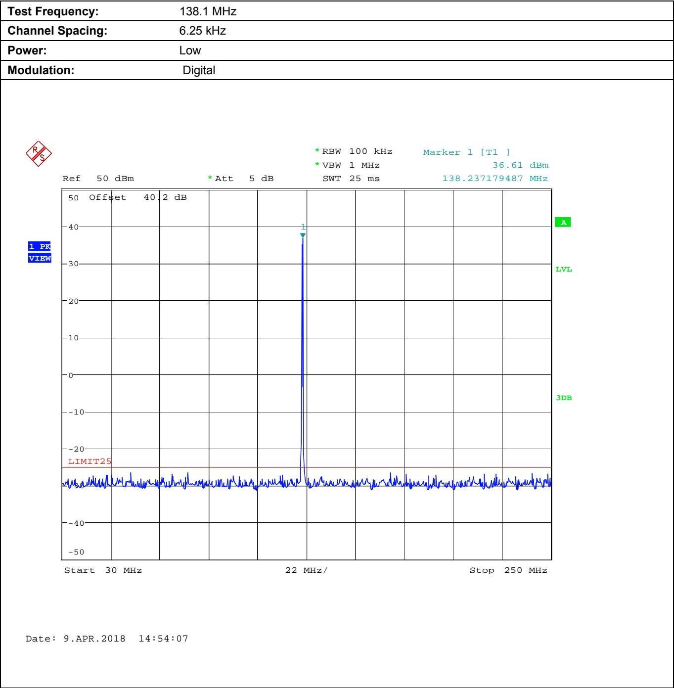
Plot 5.9.4.1.2. Conducted Transmitter Spurious Emissions for 138.1 MHz, Low Power
