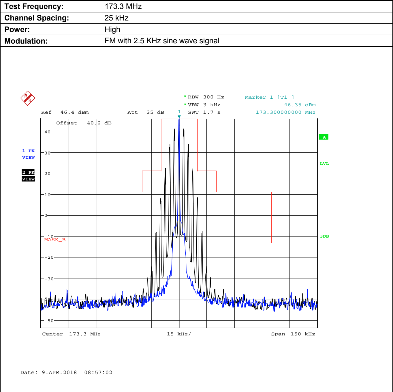
Plot 5.8.4.3.7. Emission Mask B, High Power
