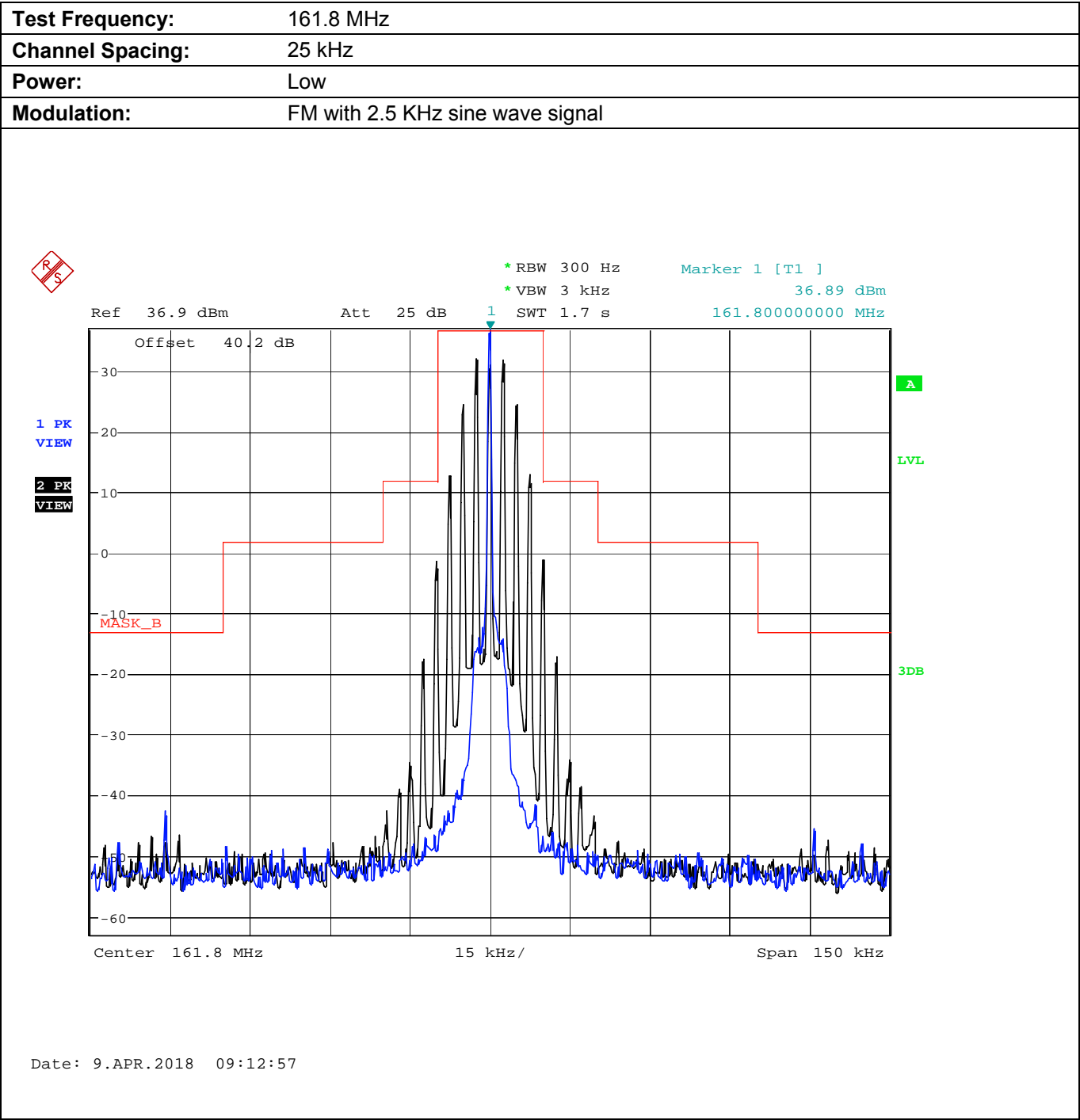
Plot 5.8.4.3.6. Emission Mask B, Low Power
