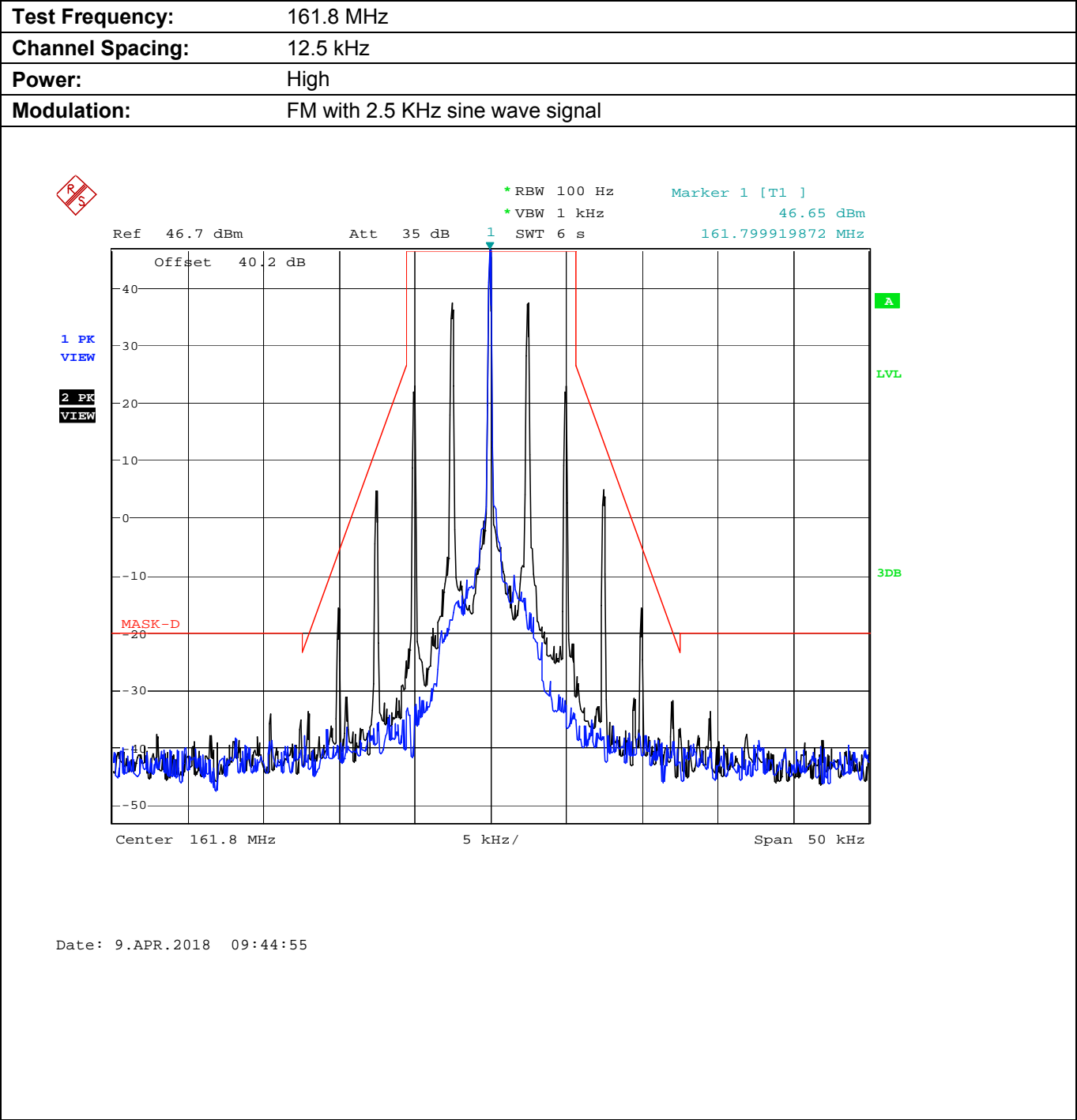
Plot 5.8.4.2.5. Emission Mask D, High Power
