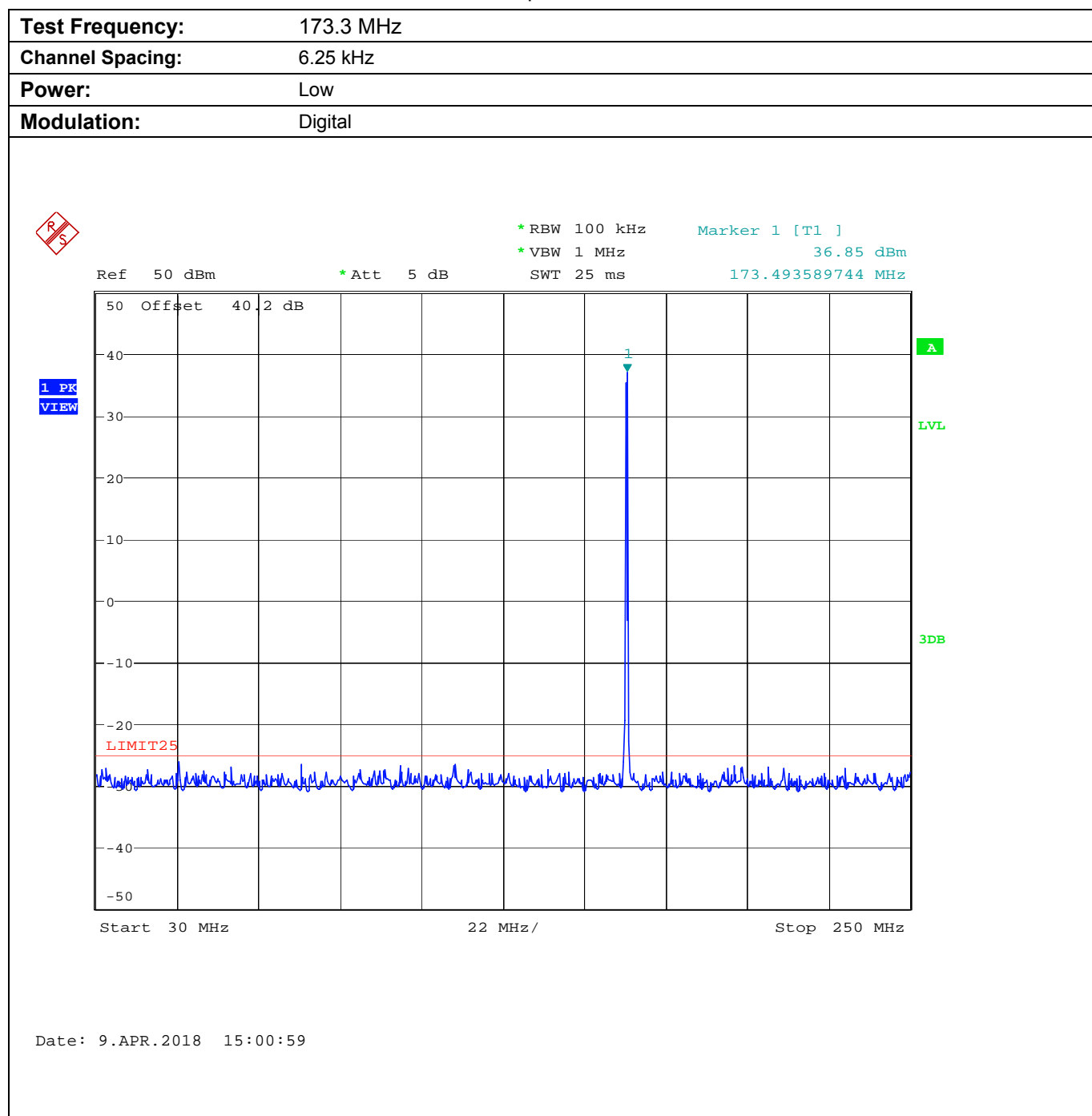
Plot 5.9.4.4.2. Conducted Transmitter Spurious Emissions for 173.3 MHz, Low Power
