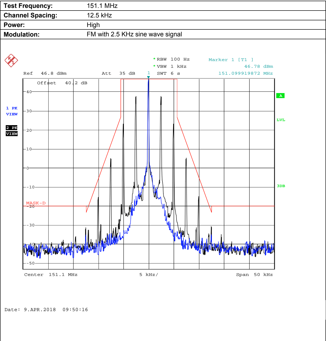
Plot 5.8.4.2.3. Emission Mask D, High Power
