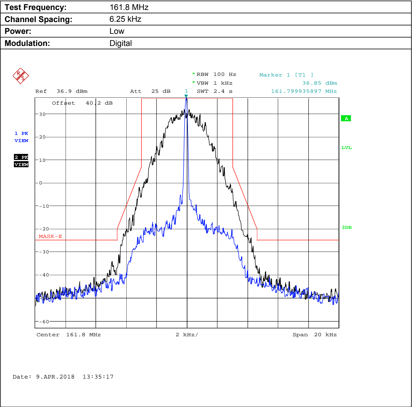
Plot 5.8.4.1.6. Emission Mask E, Low Power
