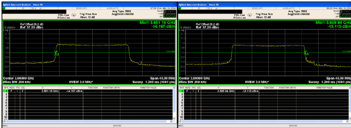
Figure 64. FL, FH for QPSK modulation, 20.0°C/115.0V - 20MHz CBW
