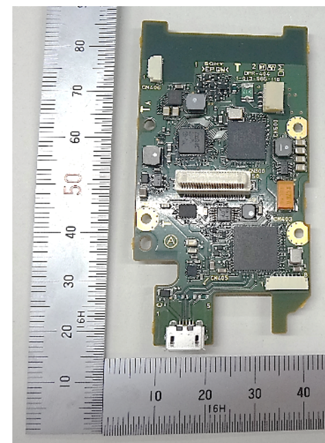
Fig.23:Side A of board DPR-404
