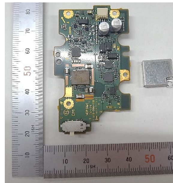
Fig.27 Remove the shield case
