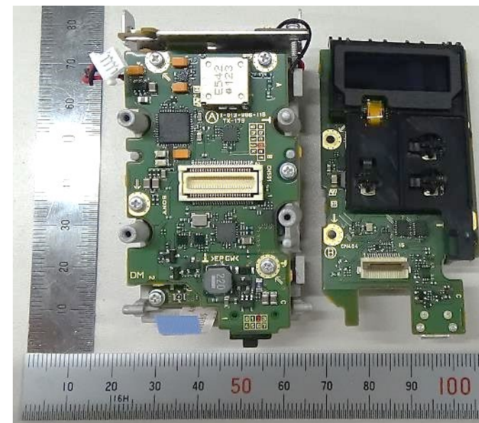
Fig.20:Remove board DPR-404
