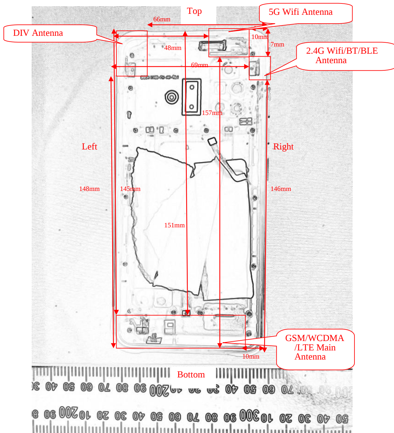
Front View
