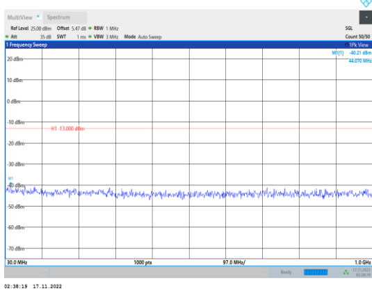
Band4-20MHz-64QAM-20050-1RB#0- Range1:30~1000MHz
