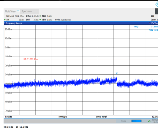
Band5-10MHz-16QAM-20600-1RB#0- Range2:1000~10000MHz
