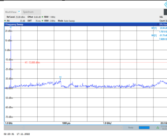
Band4-5MHz-64QAM-20375-1RB#0- Range2:1000~20000MHz
