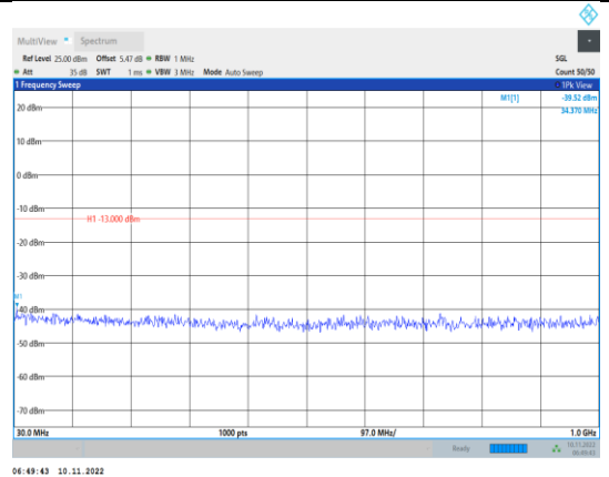
Band4-15MHz-16QAM-20325-1RB#0- Range1:30~1000MHz
