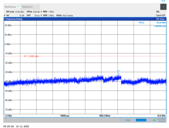
Band5-3MHz-QPSK-20525-1RB#0- Range2:1000~10000MHz
