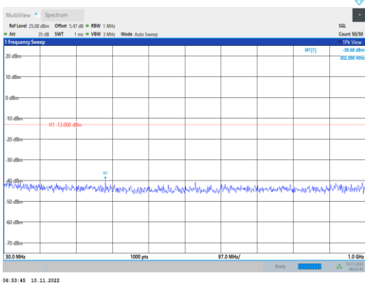
Band4-20MHz-QPSK-20050-1RB#0- Range1:30~1000MHz
