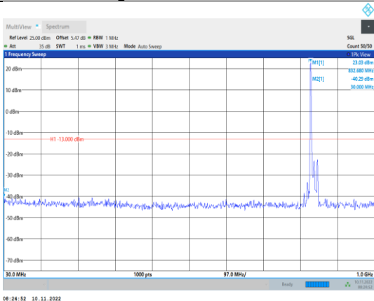
Band5-10MHz-16QAM-20525-1RB#0- Range1:30~1000MHz
