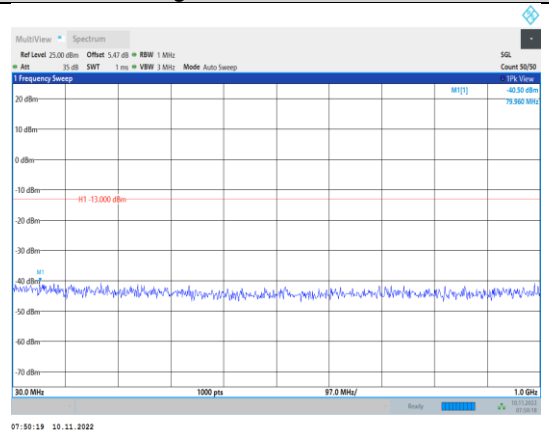
Band4-10MHz-QPSK-20350-1RB#0- Range1:30~1000MHz
