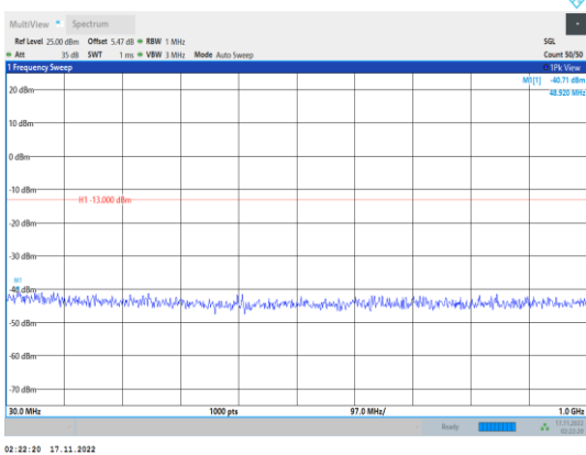
Band4-5MHz-64QAM-19975-1RB#0- Range1:30~1000MHz
