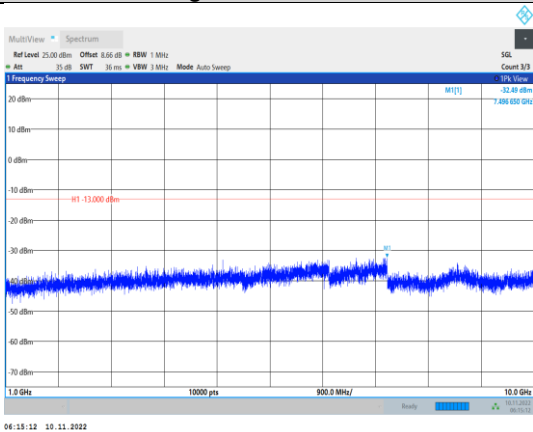
Band5-1.4MHz-16QAM-20407-1RB#0- Range2:1000~10000MHz
