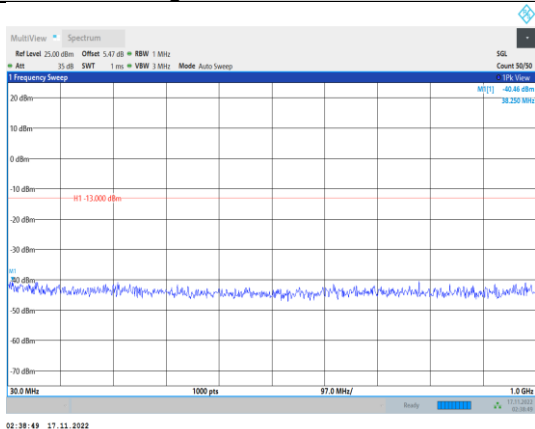
Band4-20MHz-64QAM-20175-1RB#0- Range1:30~1000MHz
