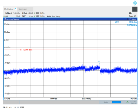
Band5-5MHz-QPSK-20625-1RB#0- Range2:1000~10000MHz
