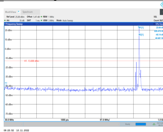
Band5-10MHz-16QAM-20600-1RB#0- Range1:30~1000MHz
