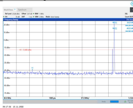
Band5-1.4MHz-16QAM-20643-1RB#0- Range1:30~1000MHz
