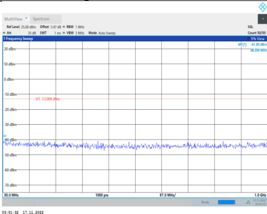
Band4-15MHz-64QAM-20175-1RB#0- Range1:30~1000MHz
