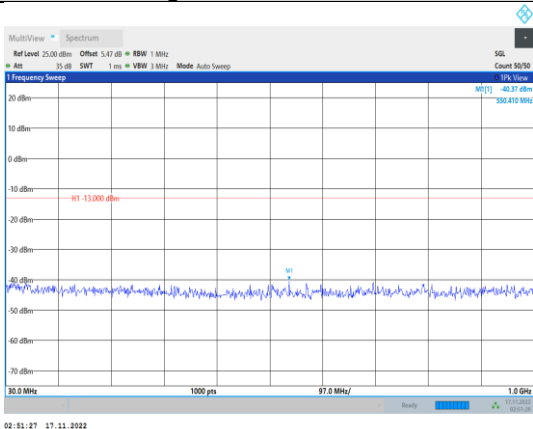
Band4-10MHz-64QAM-20175-1RB#0- Range1:30~1000MHz
