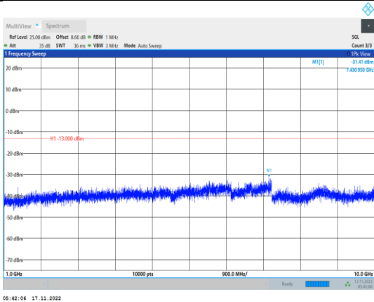
Band5-5MHz-64QAM-20425-1RB#0- Range2:1000~10000MHz
