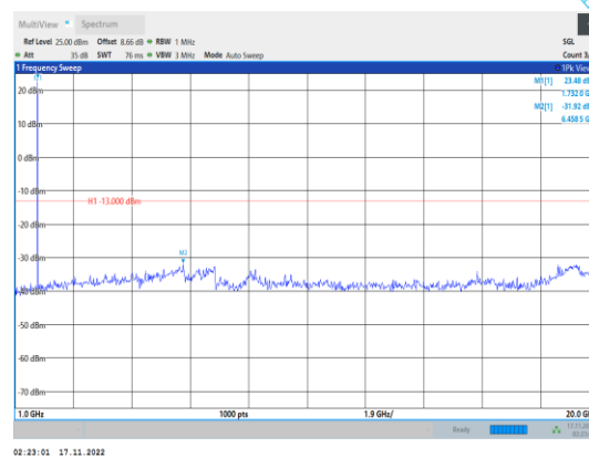
Band4-5MHz-64QAM-20175-1RB#0- Range2:1000~20000MHz
