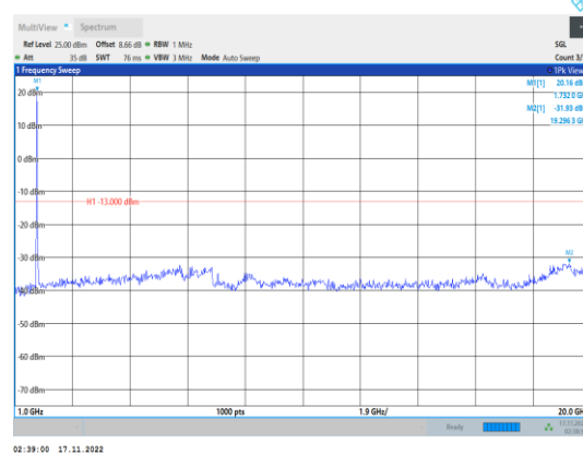
Band4-20MHz-64QAM-20175-1RB#0- Range2:1000~20000MHz
