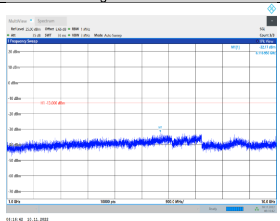
Band5-1.4MHz-QPSK-20643-1RB#0- Range2:1000~10000MHz
