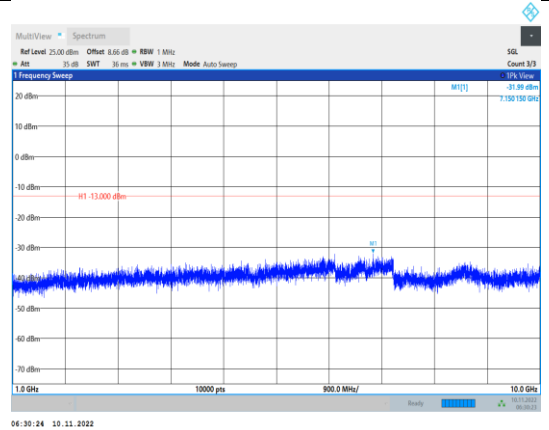
Band5-3MHz-QPSK-20635-1RB#0- Range2:1000~10000MHz
