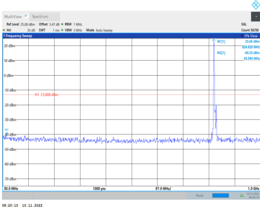
Band5-5MHz-16QAM-20425-1RB#0- Range1:30~1000MHz
