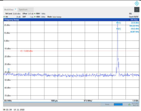
Band5-5MHz-QPSK-20625-1RB#0- Range1:30~1000MHz
