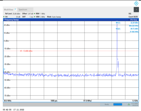
Band5-5MHz-64QAM-20625-1RB#0- Range1:30~1000MHz
