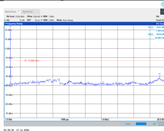
Band4-20MHz-64QAM-20300-1RB#0- Range2:1000~20000MHz
