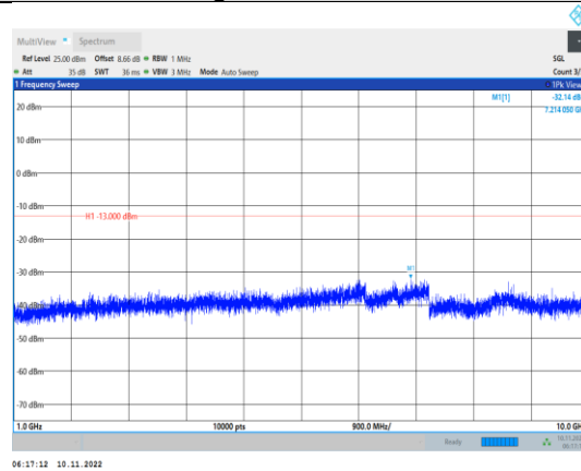
Band5-1.4MHz-16QAM-20643-1RB#0- Range2:1000~10000MHz
