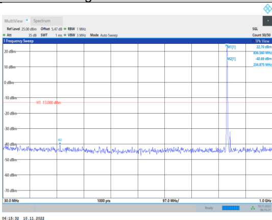
Band5-1.4MHz-QPSK-20525-1RB#0- Range1:30~1000MHz
