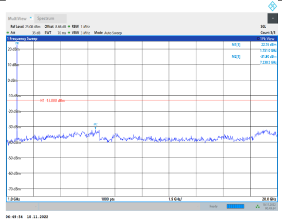
Band4-15MHz-16QAM-20325-1RB#0- Range2:1000~20000MHz
