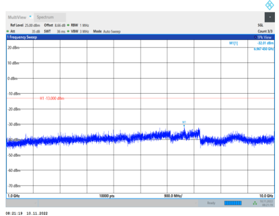
Band5-5MHz-16QAM-20525-1RB#0- Range2:1000~10000MHz
