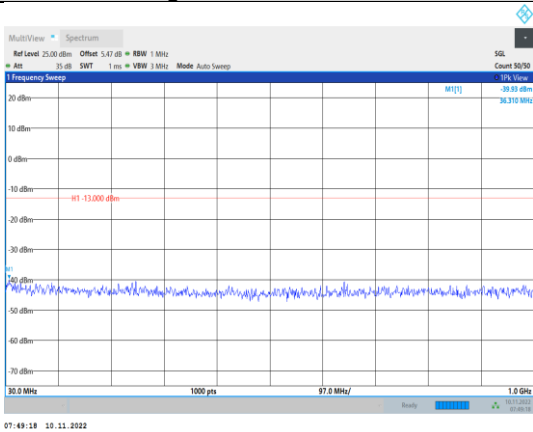
Band4-10MHz-QPSK-20175-1RB#0- Range1:30~1000MHz
