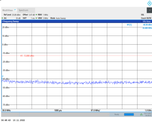
Band4-15MHz-16QAM-20175-1RB#0- Range1:30~1000MHz
