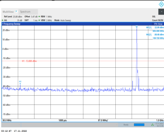
Band5-3MHz-64QAM-20525-1RB#0- Range1:30~1000MHz
