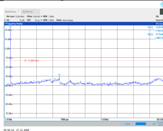
Band4-15MHz-64QAM-20325-1RB#0- Range2:1000~20000MHz
