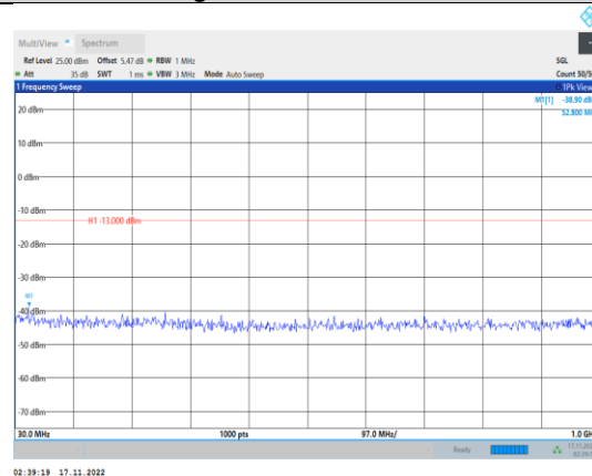
Band4-20MHz-64QAM-20300-1RB#0- Range1:30~1000MHz
