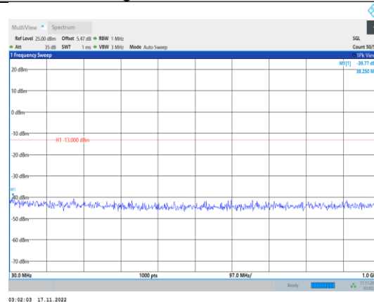
Band4-15MHz-64QAM-20325-1RB#0- Range1:30~1000MHz
