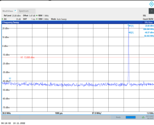
Band5-1.4MHz-16QAM-20525-1RB#0- Range1:30~1000MHz
