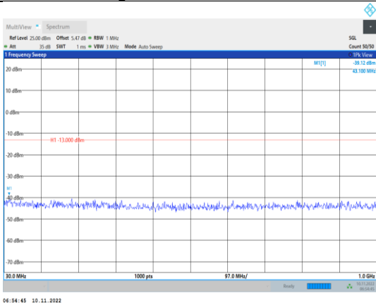
Band4-20MHz-QPSK-20175-1RB#0- Range1:30~1000MHz
