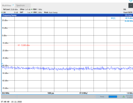
Band4-10MHz-16QAM-20000-1RB#0- Range1:30~1000MHz
