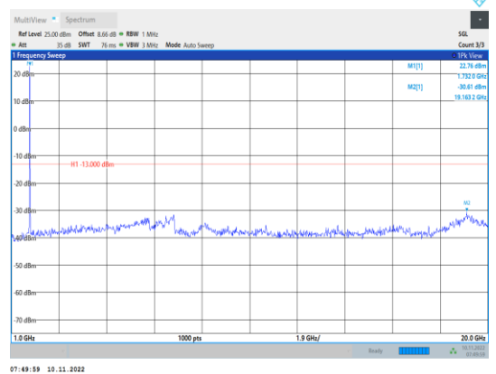
Band4-10MHz-16QAM-20175-1RB#0- Range2:1000~20000MHz
