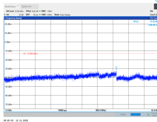
Band5-10MHz-16QAM-20525-1RB#0- Range2:1000~10000MHz
