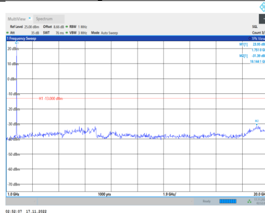
Band4-10MHz-64QAM-20350-1RB#0- Range2:1000~20000MHz
