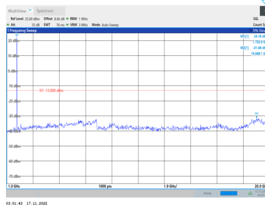
Band4-15MHz-64QAM-20175-1RB#0- Range2:1000~20000MHz
