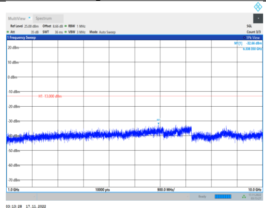
Band5-3MHz-64QAM-20635-1RB#0- Range2:1000~10000MHz
