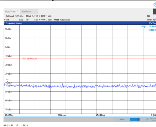
Band4-5MHz-64QAM-20375-1RB#0- Range1:30~1000MHz
