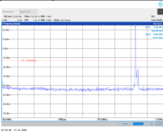
Band5-10MHz-64QAM-20525-1RB#0- Range1:30~1000MHz
