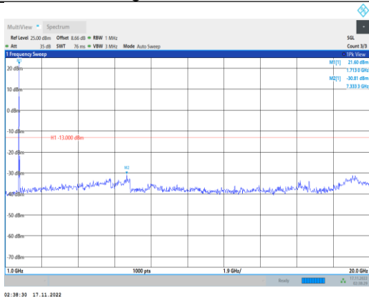
Band4-20MHz-64QAM-20050-1RB#0- Range2:1000~20000MHz
