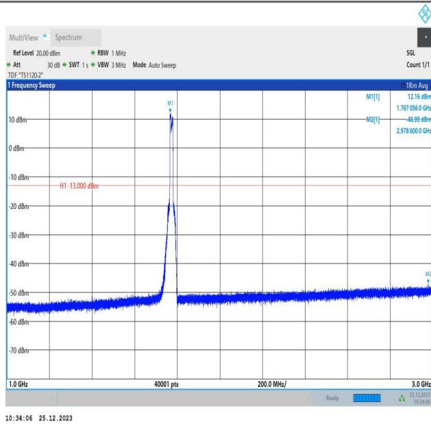
66-66-5MHz-10MHz-16QAM-16QAM-132550-132622-25RB# 0-50RB#0-1000~3000MHz-PASS
