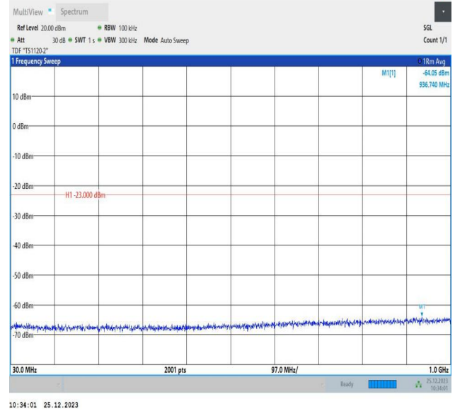
66-66-5MHz-10MHz-16QAM-16QAM-132550-132622-25RB# 0-50RB#0-30~1000MHz-PASS
