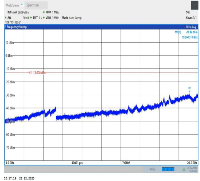
66-66-5MHz-10MHz-16QAM-16QAM-132000-132072-1RB#0-1RB#49-3000~20000MHz-PASS
