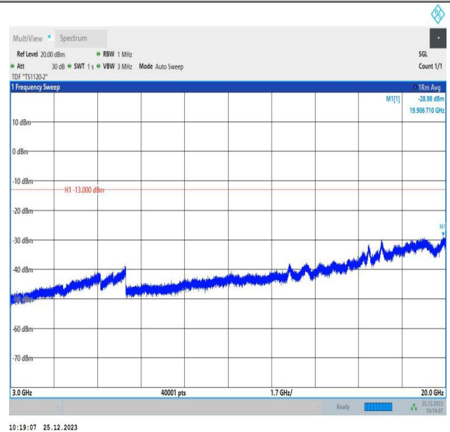
66-66-5MHz-10MHz-16QAM-16QAM-132000-132072-25RB# 0-50RB#0-3000~20000MHz-PASS
