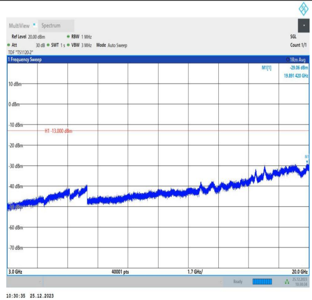
66-66-5MHz-10MHz-16QAM-16QAM-132550-132622-1RB#2 4-ORB#0-3000~20000MHz-PASS
