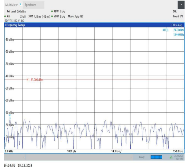
66-66-5MHz-10MHz-16QAM-16QAM-132000-132072-1RB#0- 1RB#49-0.009~0.15MHz-PASS
