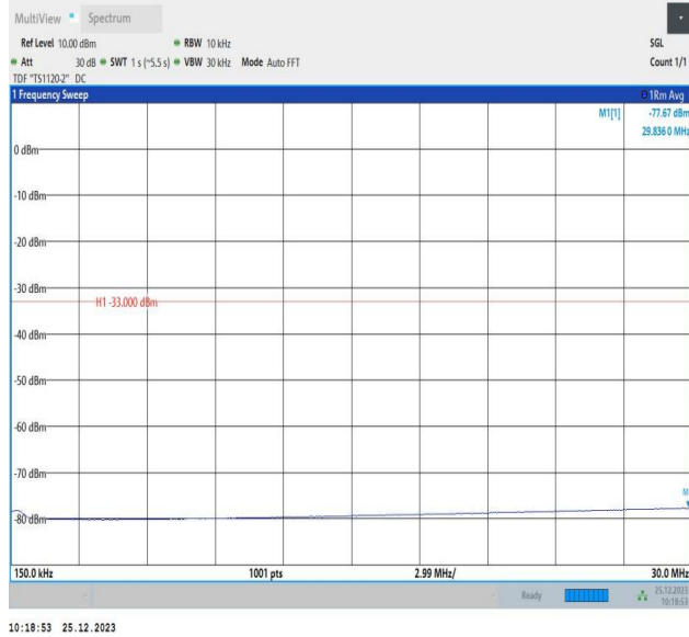
66-66-5MHz-10MHz-16QAM-16QAM-132000-132072-25RB# 0-50RB#0-0.15~30MHz-PASS
