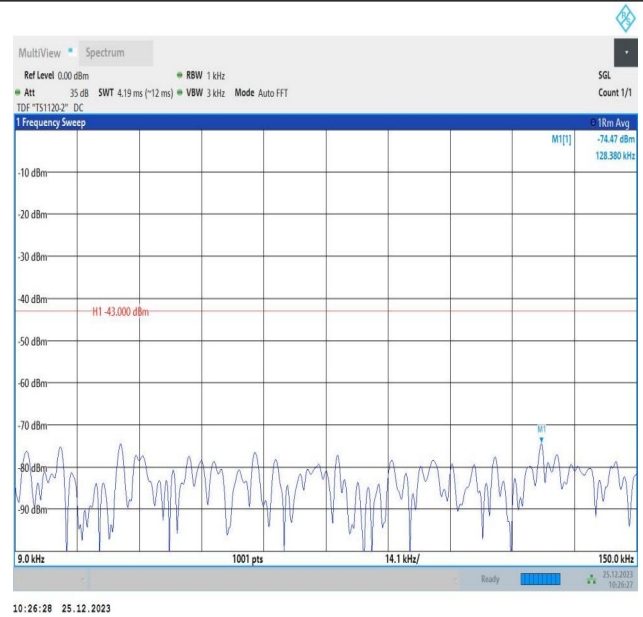
66-66-5MHz-10MHz-16QAM-16QAM-132375-132447-25RB#0-50RB#0-0.009~0.15MHz-PASS
