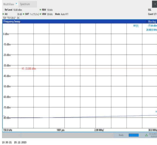
66-66-5MHz-10MHz-16QAM-16QAM-132550-132622-1RB#2 4-ORB#0-0.15~30MHz-PASS
