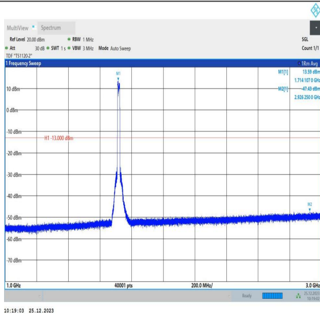
66-66-5MHz-10MHz-16QAM-16QAM-132000-132072-25RB# 0-50RB#0-1000~3000MHz-PASS
