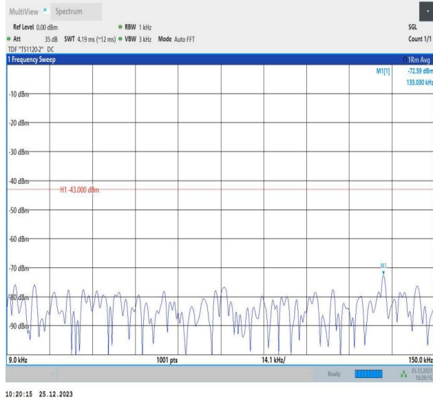
66-66-5MHz-10MHz-QPSK-QPSK-132375-132447-1RB#0-0 RB#0-0.009~0.15MHz-PASS
