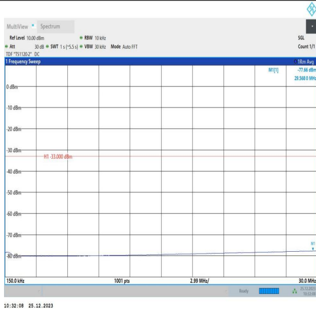
66-66-5MHz-10MHz-16QAM-16QAM-132550-132622-1RB#0 -1RB#49-0.15~30MHz-PASS
