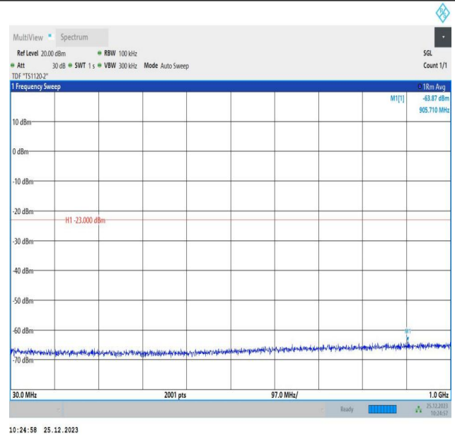
66-66-5MHz-10MHz-16QAM-16QAM-132375-132447-1RB#0- 1RB#49-30~1000MHz-PASS
