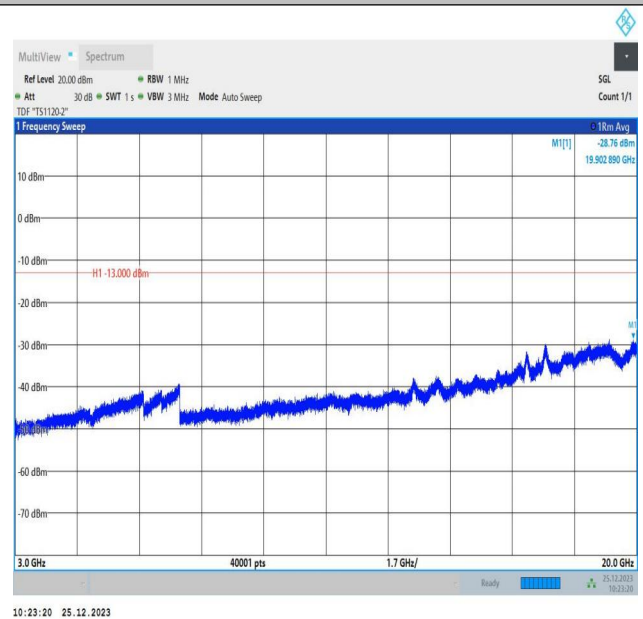
66-66-5MHz-10MHz-16QAM-16QAM-132375-132447-1RB#2 4-ORB#0-3000~20000MHz-PASS
