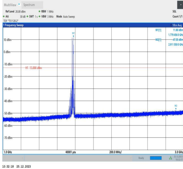
66-66-5MHz-10MHz-16QAM-16QAM-132550-132622-1RB#0-1RB#49-1000~3000MHz-PASS
