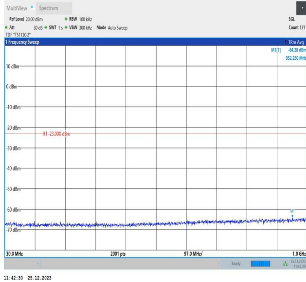
66-66-10MHz-5MHz-QPSK-QPSK-132022-132094-1RB#49- ORB#0-30~1000MHz-PASS
