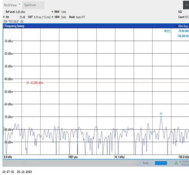
66-66-5MHz-10MHz-QPSK-QPSK-132550-132622-1RB#0-0 RB#0-0.009~0.15MHz-PASS
