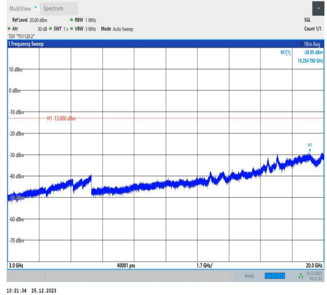
66-66-5MHz-10MHz-16QAM-16QAM-132375-132447-1RB#0-0RB#0-3000~20000MHz-PASS
