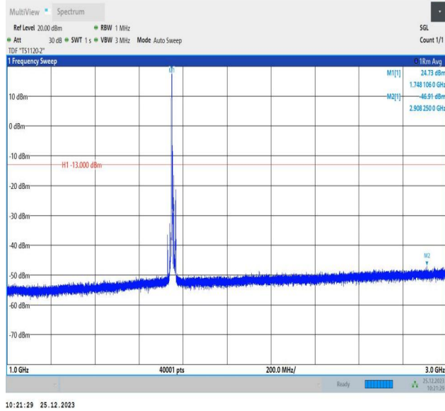
66-66-5MHz-10MHz-16QAM-16QAM-132375-132447-1RB#0-0RB#0-1000~3000MHz-PASS
