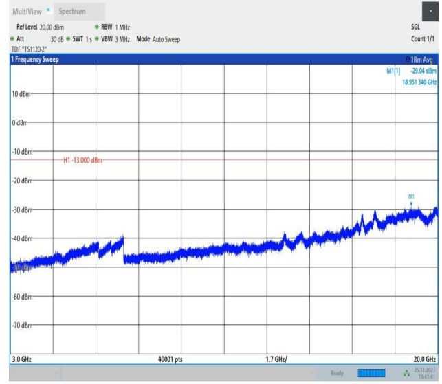
66-66-10MHz-5MHz-16QAM-16QAM-132022-132094-1RB#0-0RB#0-3000~20000MHz-PASS
