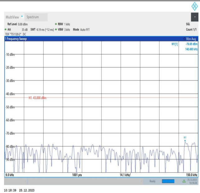
66-66-5MHz-10MHz-16QAM-16QAM-132000-132072-25RB#0-50RB#0-0.009~0.15MHz-PASS
