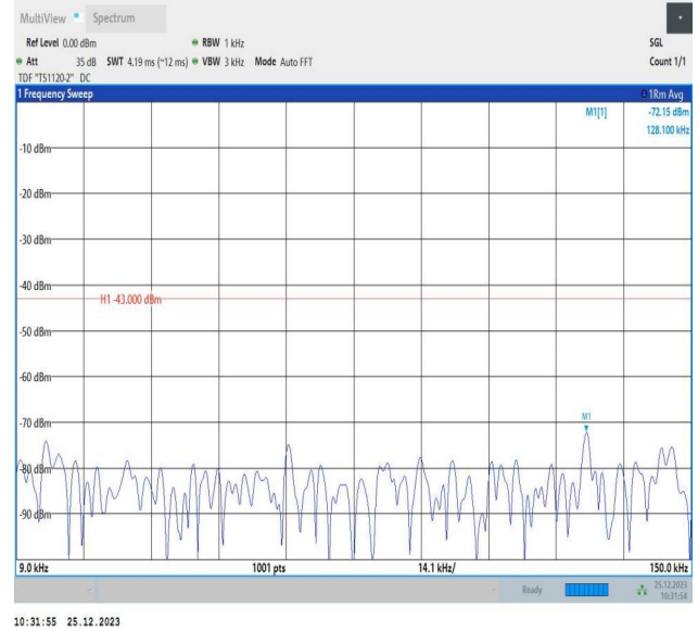
66-66-5MHz-10MHz-16QAM-16QAM-132550-132622-1RB#0- 1RB#49-0.009~0.15MHz-PASS
