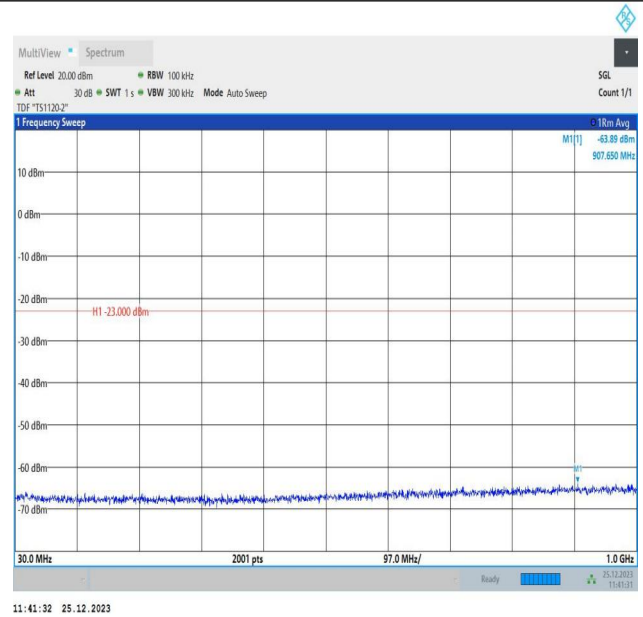
66-66-10MHz-5MHz-16QAM-16QAM-132022-132094-1RB#0-0RB#0-30~1000MHz-PASS
