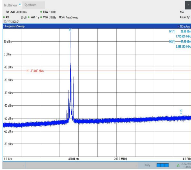
66-66-10MHz-5MHz-16QAM-16QAM-132022-132094-1RB#0-0RB#0-1000~3000MHz-PASS
