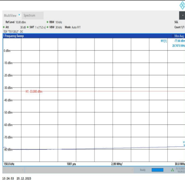
66-66-5MHz-10MHz-16QAM-16QAM-132375-132447-1RB#0 -1RB#49-0.15~30MHz-PASS
