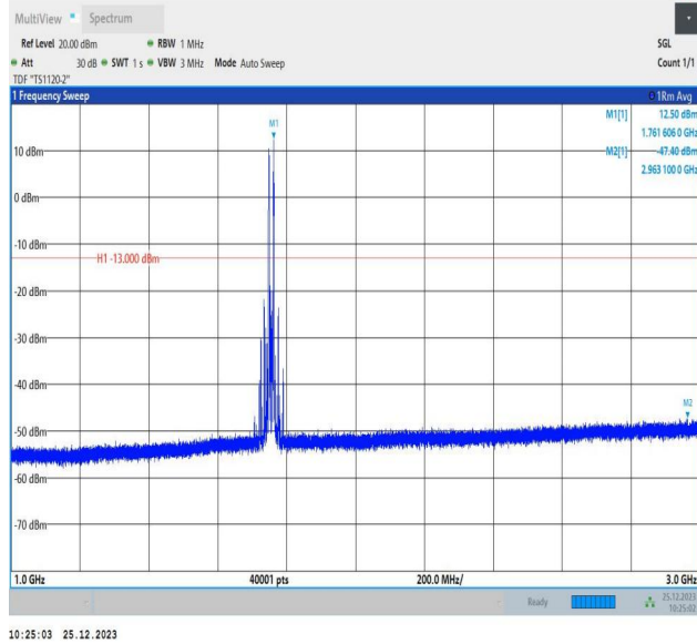
66-66-5MHz-10MHz-16QAM-16QAM-132375-132447-1RB#0-1RB#49-1000~3000MHz-PASS
