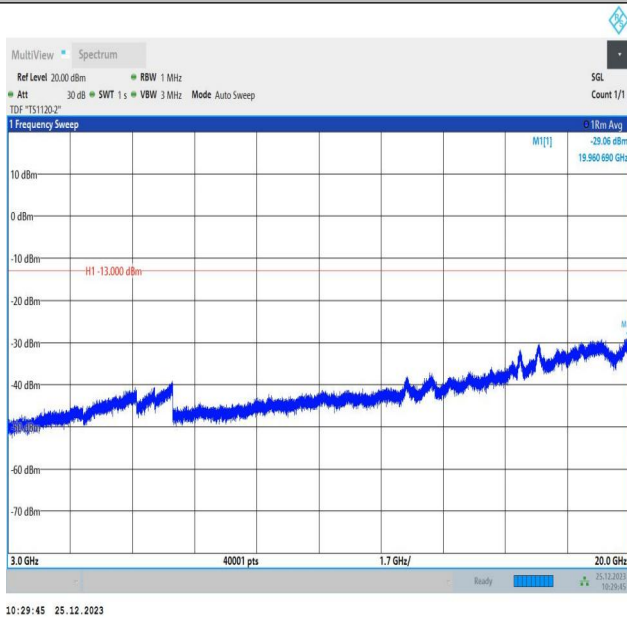
66-66-5MHz-10MHz-QPSK-QPSK-132550-132622-1RB#24- ORB#0-3000~20000MHz-PASS
