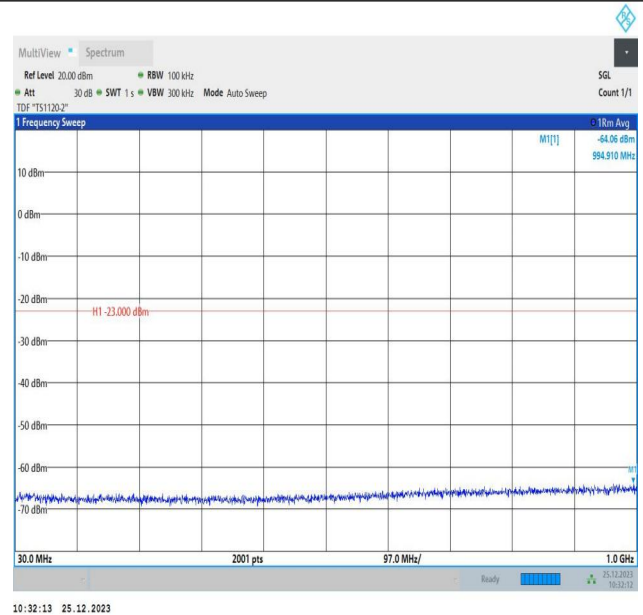
66-66-5MHz-10MHz-16QAM-16QAM-132550-132622-1RB#0- 1RB#49-30~1000MHz-PASS
