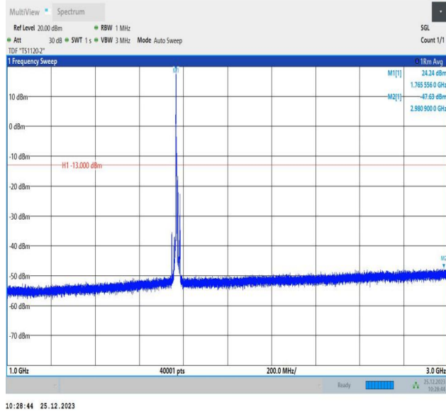
66-66-5MHz-10MHz-16QAM-16QAM-132550-132622-1RB#0-0RB#0-1000~3000MHz-PASS
