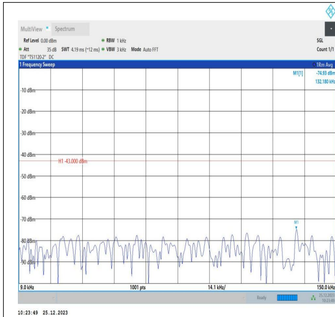
66-66-5MHz-10MHz-QPSK-QPSK-132375-132447-1RB#0-1 RB#49-0.009~0.15MHz-PASS
