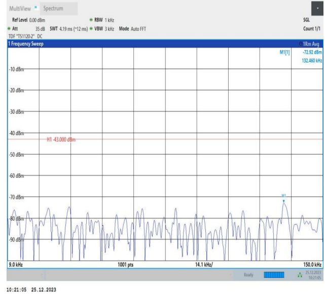
66-66-5MHz-10MHz-16QAM-16QAM-132375-132447-1RB#0-0 ORB#0-0.009~0.15MHz-PASS
