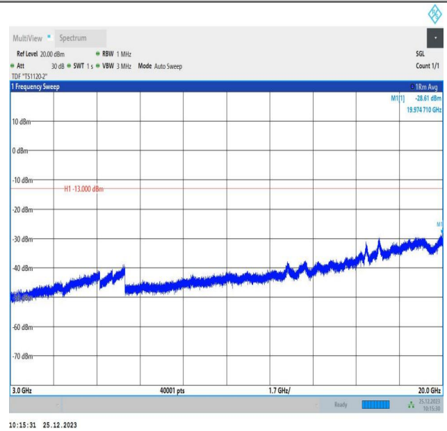
66-66-5MHz-10MHz-16QAM-16QAM-132000-132072-1RB#2 4-ORB#0-3000~20000MHz-PASS
