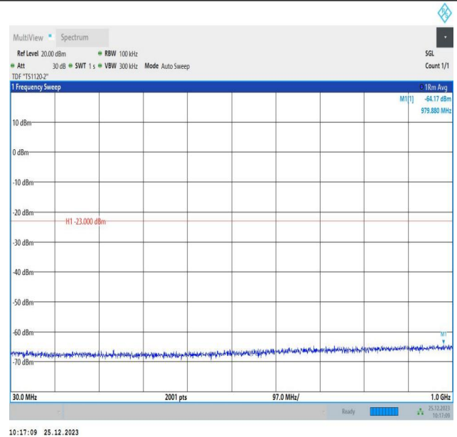
66-66-5MHz-10MHz-16QAM-16QAM-132000-132072-1RB#0- 1RB#49-30~1000MHz-PASS
