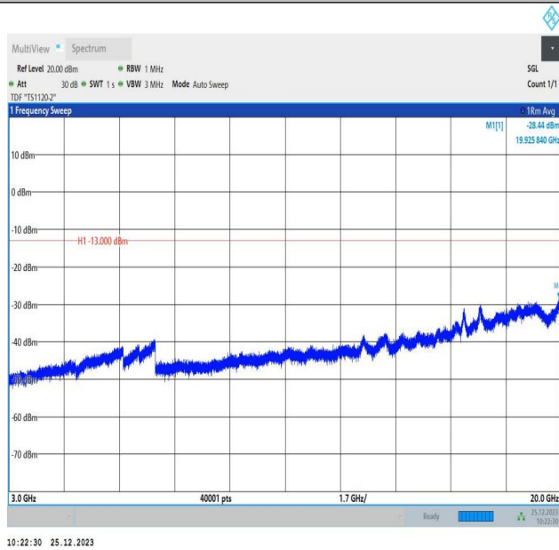
66-66-5MHz-10MHz-QPSK-QPSK-132375-132447-1RB#24- ORB#0-3000~20000MHz-PASS
