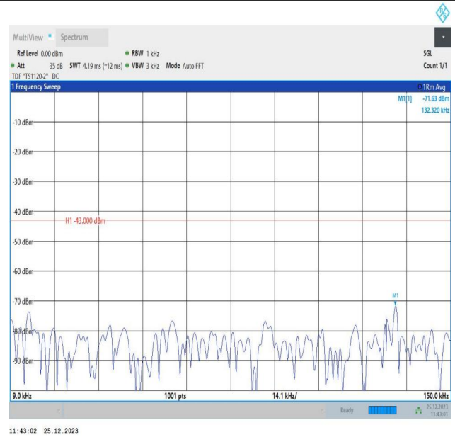
66-66-10MHz-5MHz-16QAM-16QAM-132022-132094-1RB#4 9-ORB#0-0.009~0.15MHz-PASS
