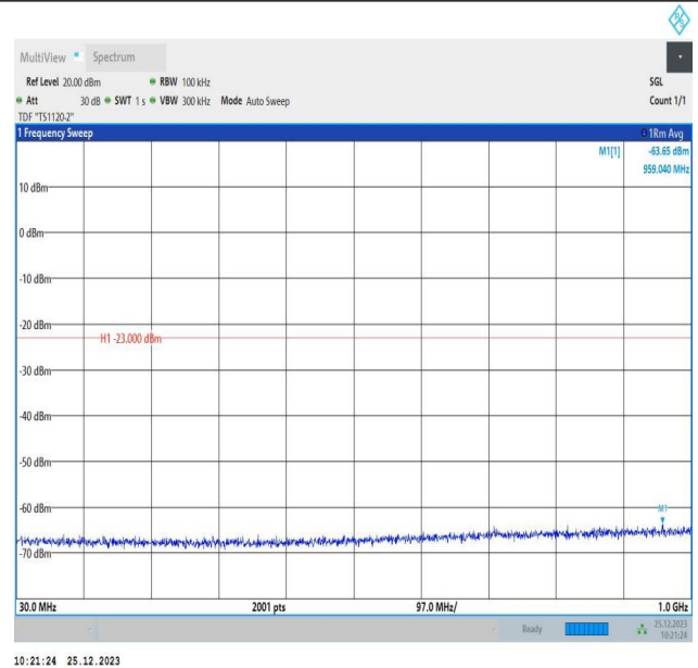
66-66-5MHz-10MHz-16QAM-16QAM-132375-132447-1RB#0-0 ORB#0-30~1000MHz-PASS
