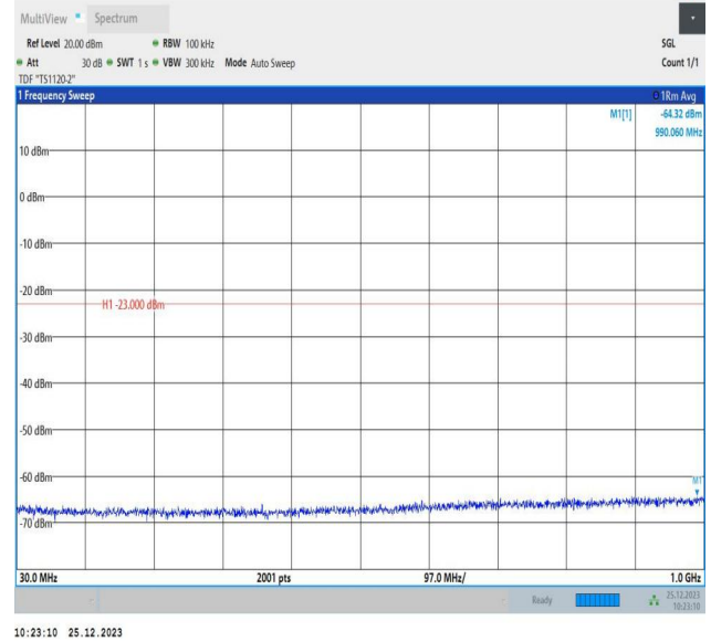
66-66-5MHz-10MHz-16QAM-16QAM-132375-132447-1RB#2 4-ORB#0-30~1000MHz-PASS
