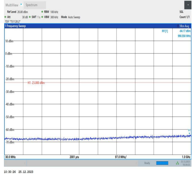
66-66-5MHz-10MHz-16QAM-16QAM-132550-132622-1RB#2 4-ORB#0-30~1000MHz-PASS
