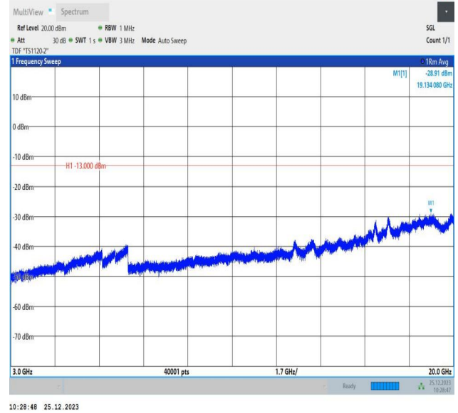
66-66-5MHz-10MHz-16QAM-16QAM-132550-132622-1RB#0-0RB#0-3000~20000MHz-PASS
