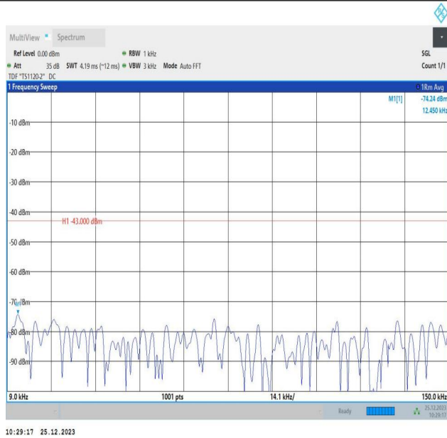
66-66-5MHz-10MHz-QPSK-QPSK-132550-132622-1RB#24-0RB#0-0.009~0.15MHz-PASS
