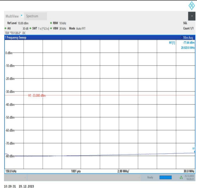
66-66-5MHz-10MHz-QPSK-QPSK-132550-132622-1RB#24-0RB#0-0.15~30MHz-PASS
