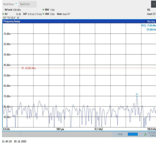
66-66-10MHz-5MHz-QPSK-QPSK-132022-132094-1RB#0-0 RB#0-0.009~0.15MHz-PASS
