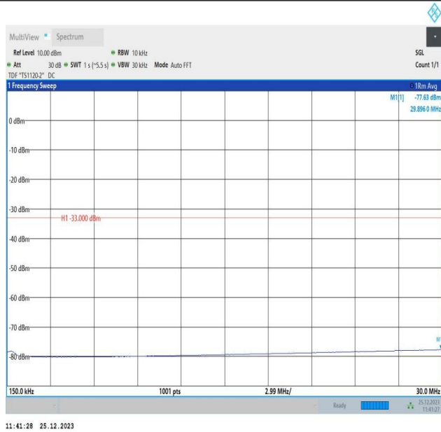
66-66-10MHz-5MHz-16QAM-16QAM-132022-132094-1RB#0-0RB#0-0.15~30MHz-PASS
