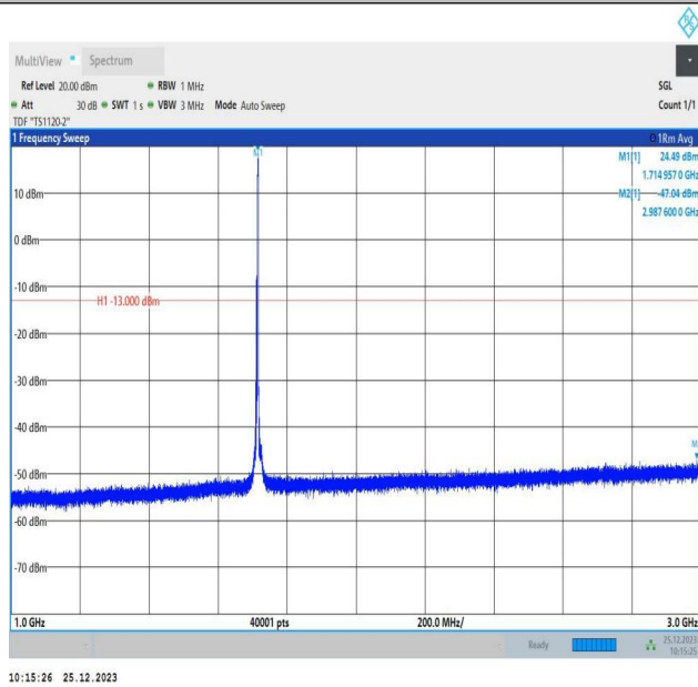
66-66-5MHz-10MHz-16QAM-16QAM-132000-132072-1RB#2 4-ORB#0-1000~3000MHz-PASS
