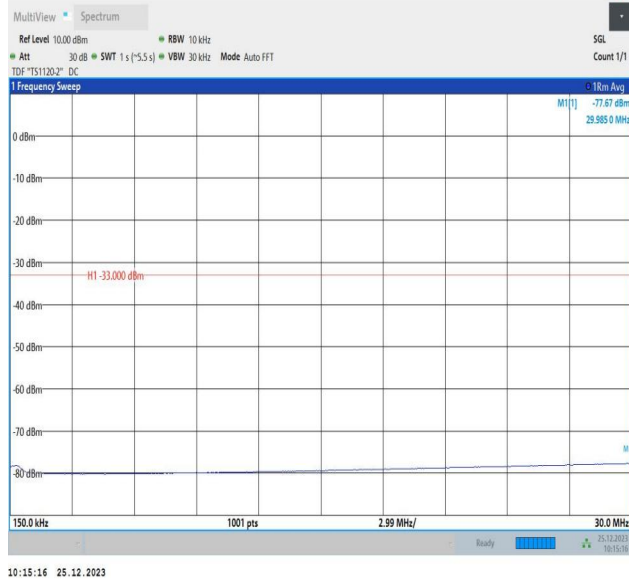
66-66-5MHz-10MHz-16QAM-16QAM-132000-132072-1RB#2 4-ORB#0-0.15~30MHz-PASS
