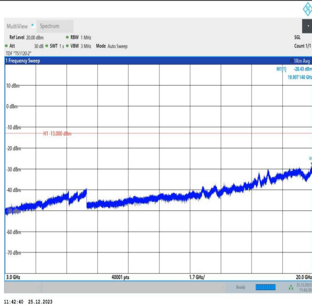
66-66-10MHz-5MHz-QPSK-QPSK-132022-132094-1RB#49- ORB#0-3000~20000MHz-PASS
