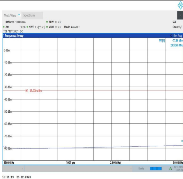
66-66-5MHz-10MHz-16QAM-16QAM-132375-132447-1RB#0-0 -ORB#0-0.15~30MHz-PASS
