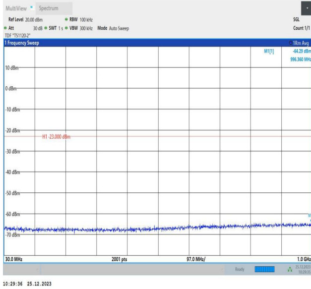
66-66-5MHz-10MHz-QPSK-QPSK-132550-132622-1RB#24- ORB#0-30~1000MHz-PASS
