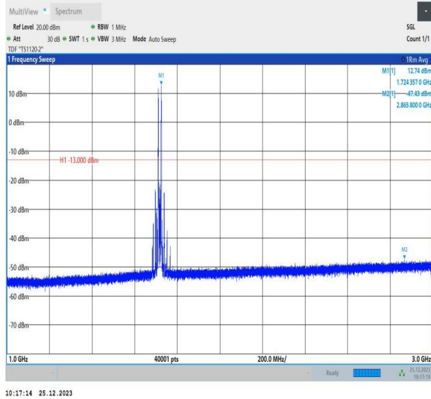
66-66-5MHz-10MHz-16QAM-16QAM-132000-132072-1RB#0-1RB#49-1000~3000MHz-PASS
