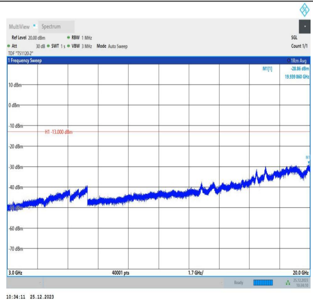
66-66-5MHz-10MHz-16QAM-16QAM-132550-132622-25RB# 0-50RB#0-3000~20000MHz-PASS
