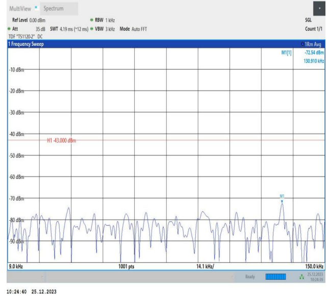
66-66-5MHz-10MHz-16QAM-16QAM-132375-132447-1RB#0- 1RB#49-0.009~0.15MHz-PASS
