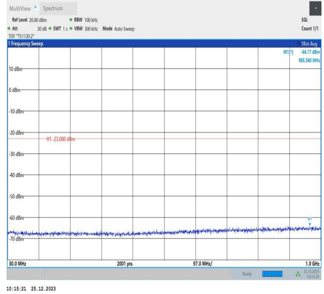
66-66-5MHz-10MHz-16QAM-16QAM-132000-132072-1RB#2 4-ORB#0-30~1000MHz-PASS
