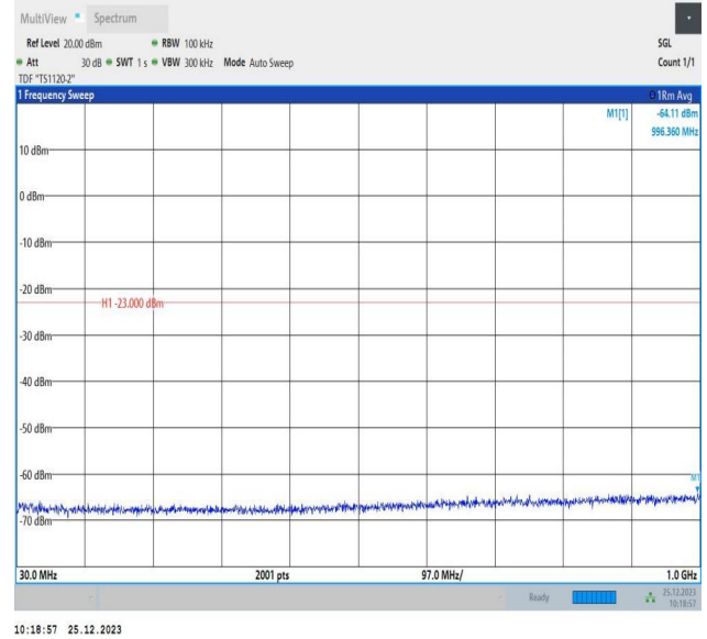
66-66-5MHz-10MHz-16QAM-16QAM-132000-132072-25RB# 0-50RB#0-30~1000MHz-PASS
