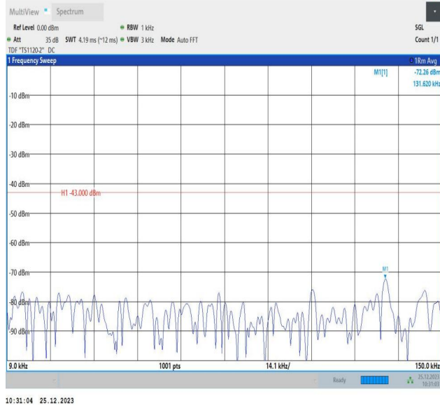
66-66-5MHz-10MHz-QPSK-QPSK-132550-132622-1RB#0-1 RB#49-0.009~0.15MHz-PASS
