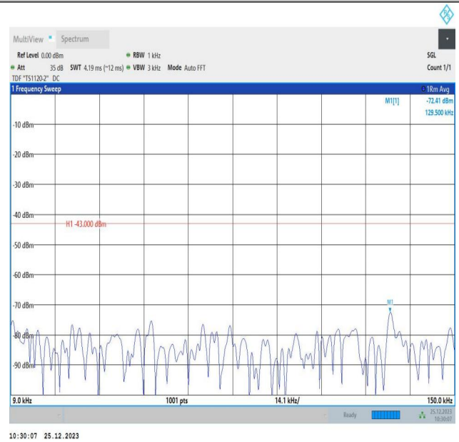
66-66-5MHz-10MHz-16QAM-16QAM-132550-132622-1RB#2 4-ORB#0-0.009~0.15MHz-PASS
