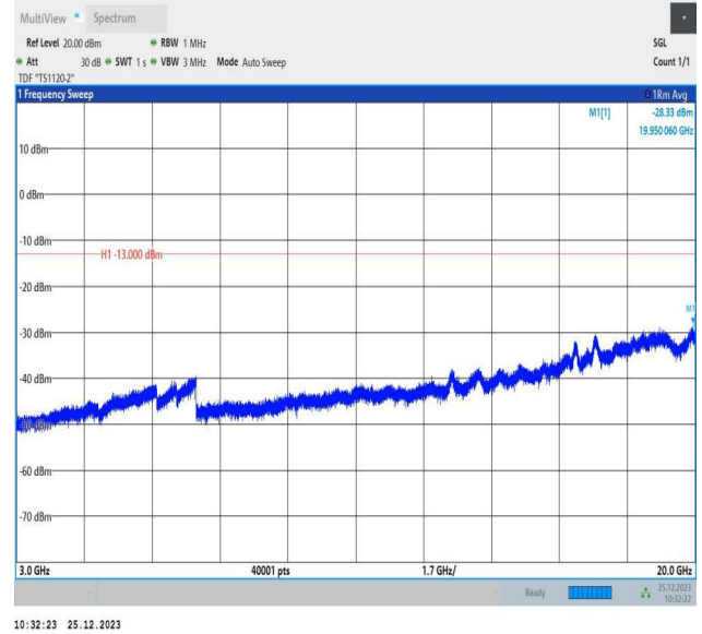
66-66-5MHz-10MHz-16QAM-16QAM-132550-132622-1RB#0-1RB#49-3000~20000MHz-PASS
