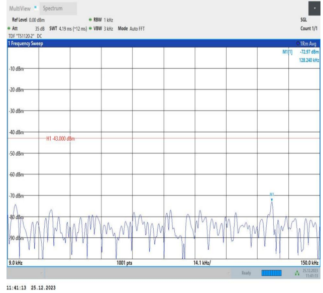
66-66-10MHz-5MHz-16QAM-16QAM-132022-132094-1RB#0-0RB#0-0.009~0.15MHz-PASS
