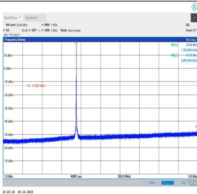
66-66-5MHz-10MHz-16QAM-16QAM-132375-132447-1RB#2 4-ORB#0-1000~3000MHz-PASS
