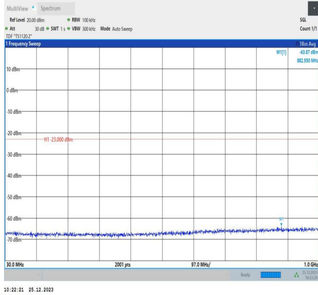
66-66-5MHz-10MHz-QPSK-QPSK-132375-132447-1RB#24- ORB#0-30~1000MHz-PASS
