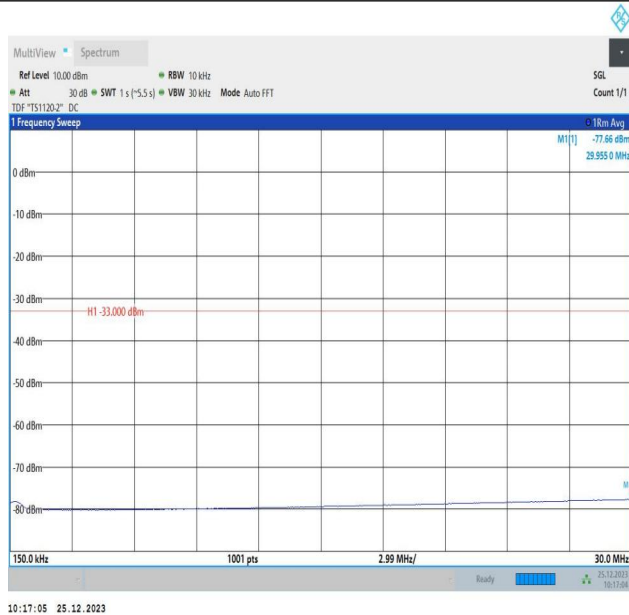
66-66-5MHz-10MHz-16QAM-16QAM-132000-132072-1RB#0 -1RB#49-0.15~30MHz-PASS
