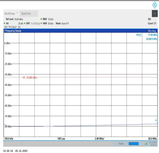
66-66-5MHz-10MHz-QPSK-QPSK-132375-132447-1RB#24-0RB#0-0.15~30MHz-PASS
