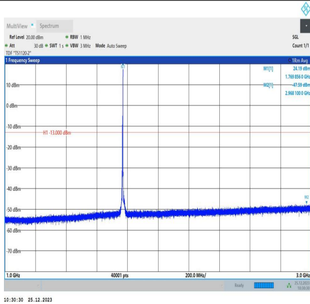
66-66-5MHz-10MHz-16QAM-16QAM-132550-132622-1RB#2 4-ORB#0-1000~3000MHz-PASS
