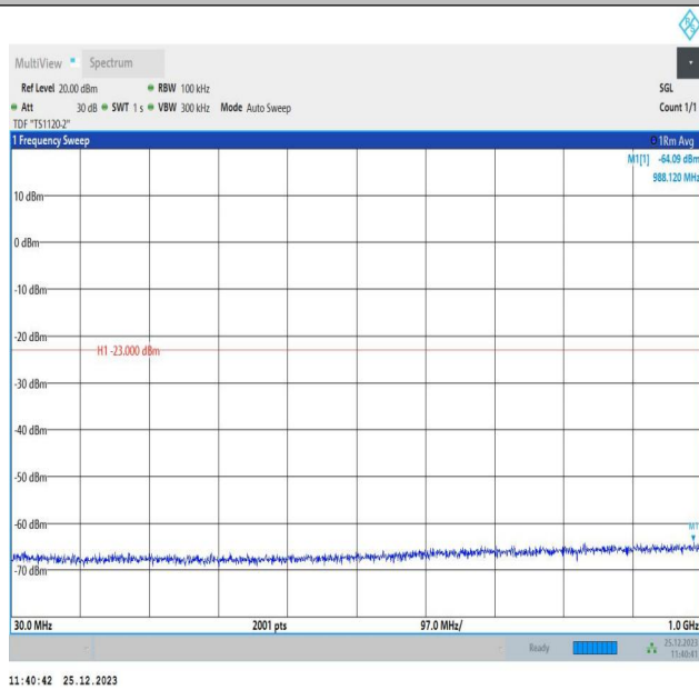
66-66-10MHz-5MHz-QPSK-QPSK-132022-132094-1RB#0-0 RB#0-30~1000MHz-PASS
