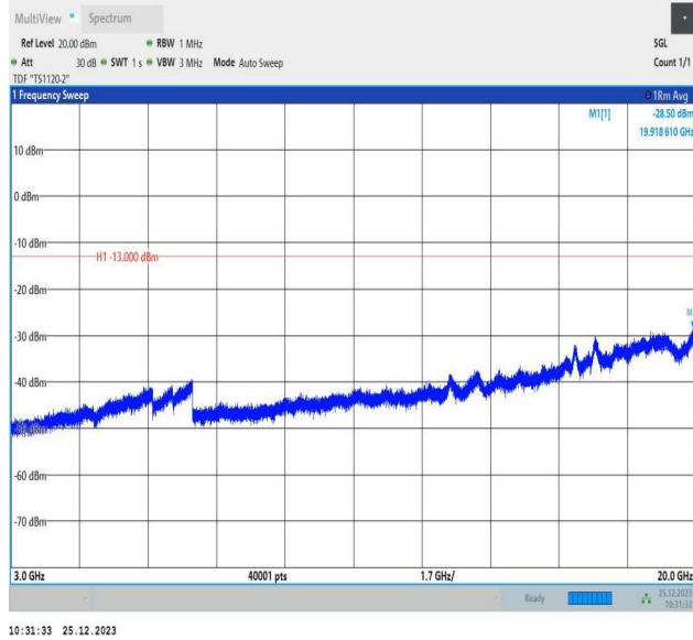
66-66-5MHz-10MHz-QPSK-QPSK-132550-132622-1RB#0-1 RB#49-3000~20000MHz-PASS
