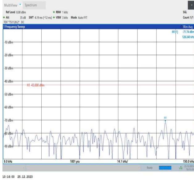
66-66-5MHz-10MHz-QPSK-QPSK-132000-132072-1RB#0-1 RB#49-0.009~0.15MHz-PASS
