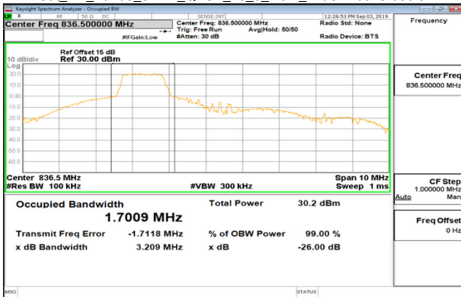
Cat_M1_Band5_5MHz_QPSK_25_0_Main_MidCH20525-836.5
