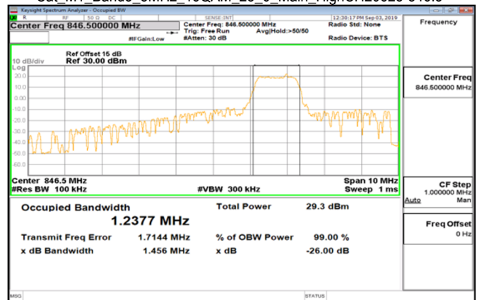
Cat_M1_Band5_5MHz_16QAM_25_0_Main_HighCH20625-846.5
