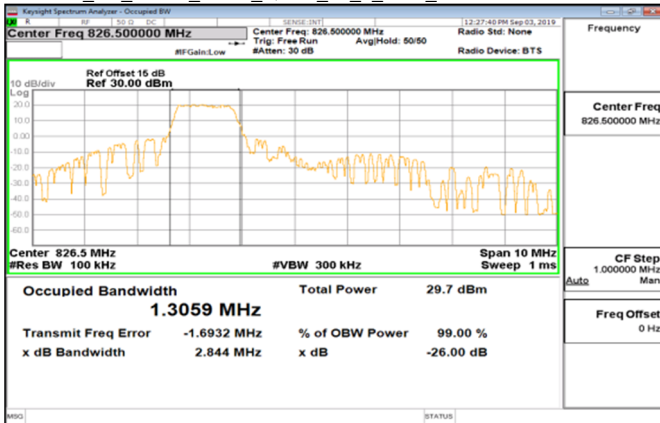
Cat_M1_Band5_5MHz_QPSK_25_0_Main_LowCH20425-826.5
