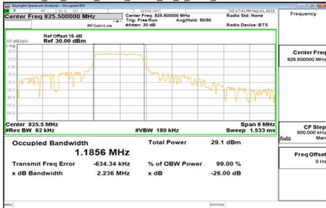
Cat_M1_Band5_3MHz_QPSK_15_0_Main_LowCH20415-825.5
