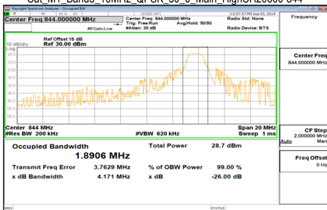
Cat_M1_Band5_10MHz_QPSK_50_0_Main_HighCH20600-844
