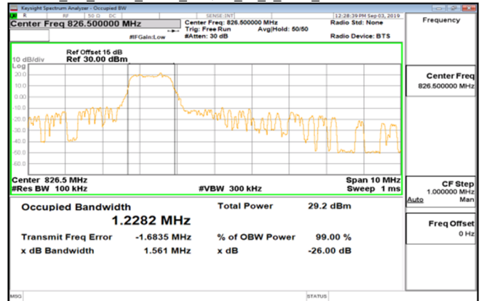
Cat_M1_Band5_5MHz_16QAM_25_0_Main_LowCH20425-826.5
