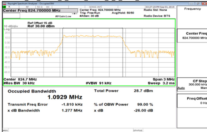
Cat_M1_Band5_1_4MHz_QPSK_6_0_Main_LowCH20407-824.7
