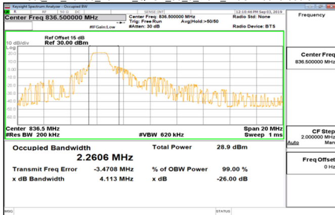
Cat_M1_Band5_10MHz_QPSK_50_0_Main_MidCH20525-836.5
