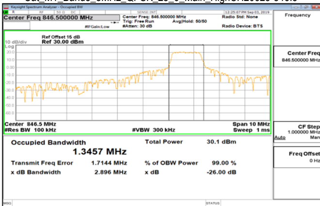
Cat_M1_Band5_5MHz_QPSK_25_0_Main_HighCH20625-846.5
