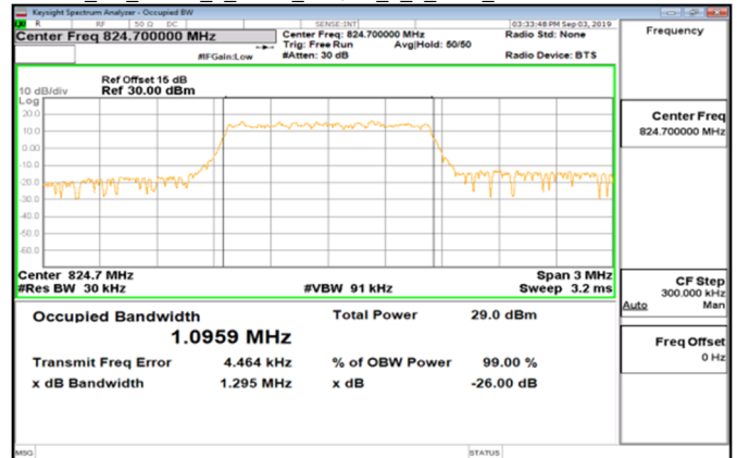
Cat_M1_Band5_1_4MHz_16QAM_6_0_Main_LowCH20407-824.7
