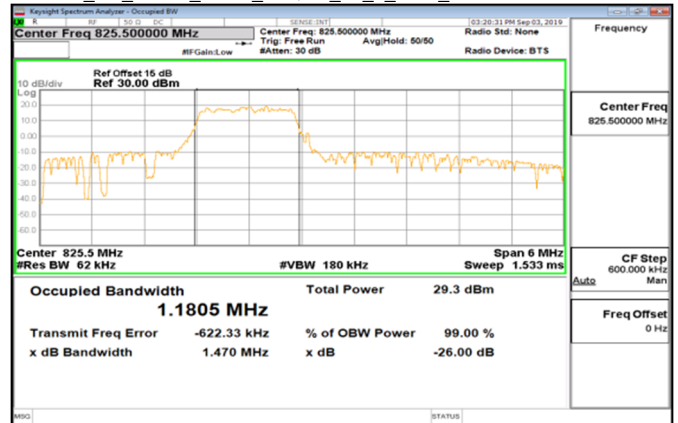
Cat_M1_Band5_3MHz_16QAM_15_0_Main_LowCH20415-825.5
