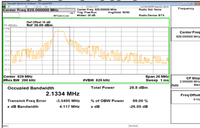
Cat_M1_Band5_10MHz_QPSK_50_0_Main_LowCH20450-829
