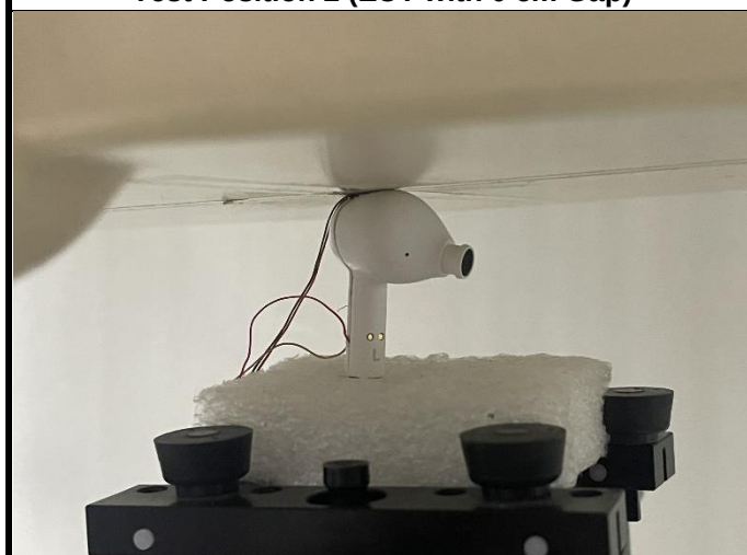
Test Position 4 (EUT with 0 cm Gap)
