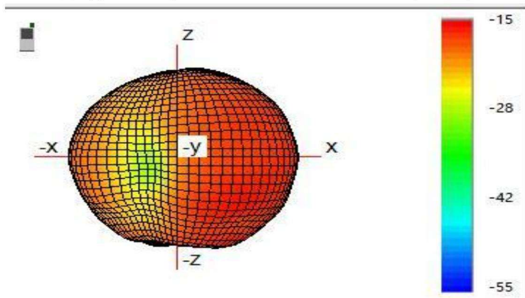
(4) Typical Free Space 3D Radiation Pattern at 928MHz(unit:dBi):
