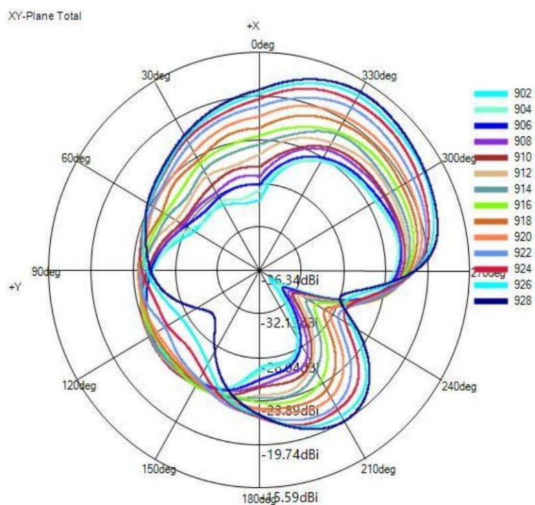
(3) X-Y Plane(unit:dBi):
