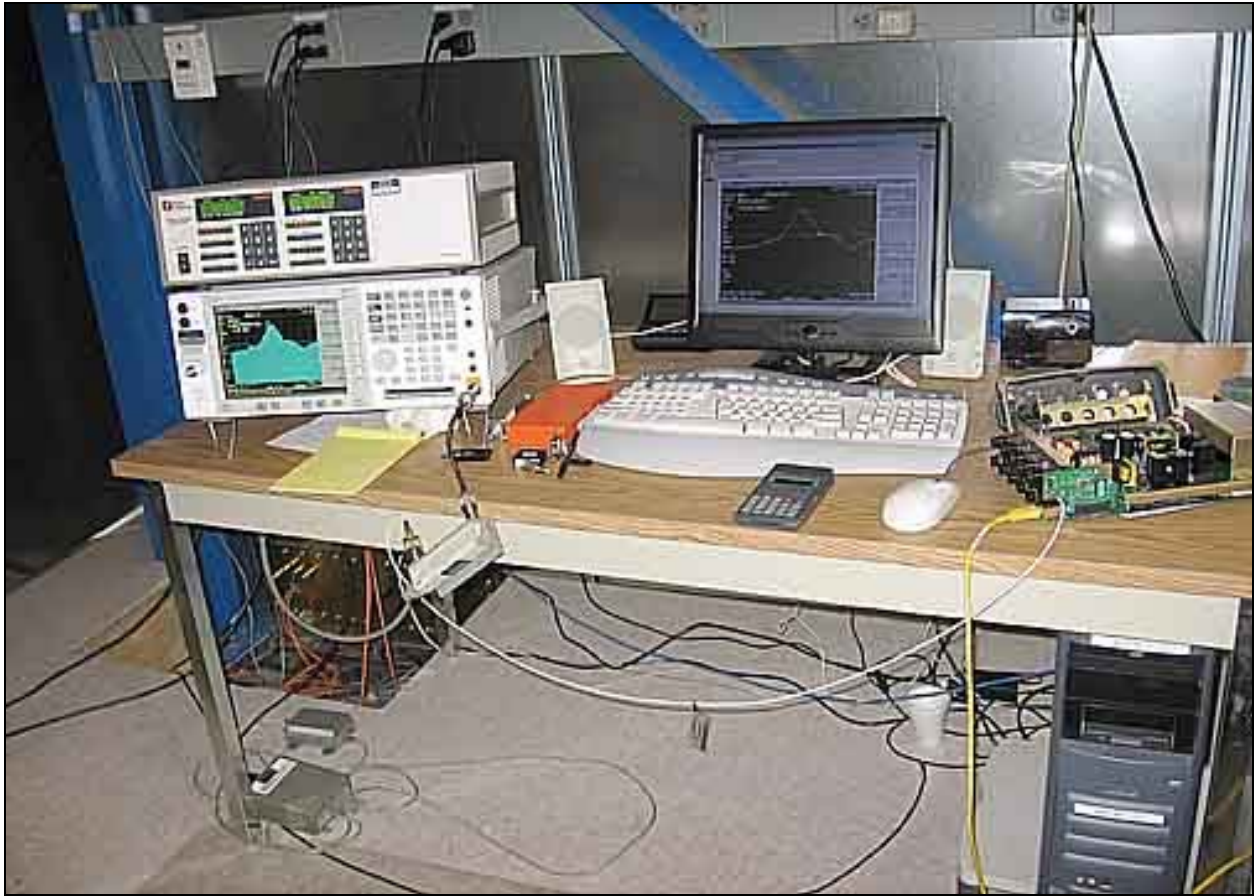
Voltage Variations
