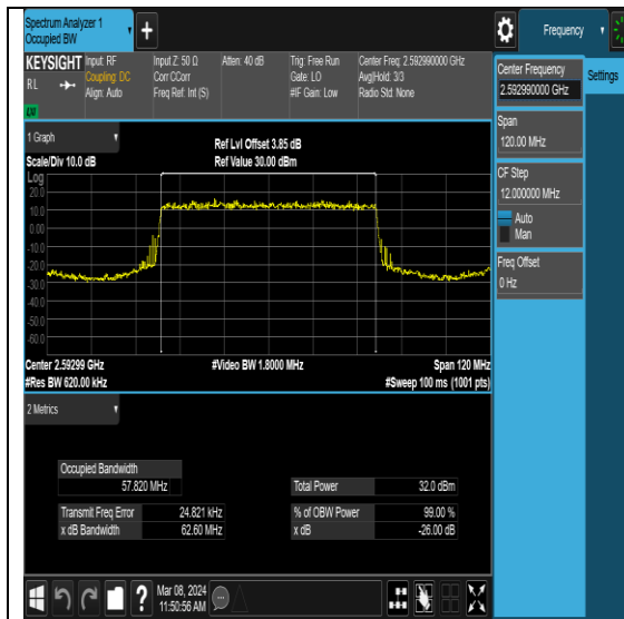
NTNV-N41-PC2-30-60-M-DFT-PI2BPSK- Outer_Full-Ant0-PASS
