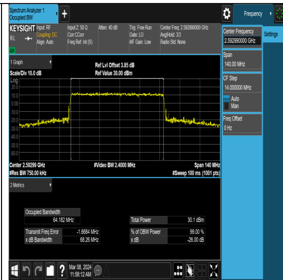
NTNV-N41-PC2-30-70-M-DFT-256QAM-Outer_Full-Ant0-PASS
