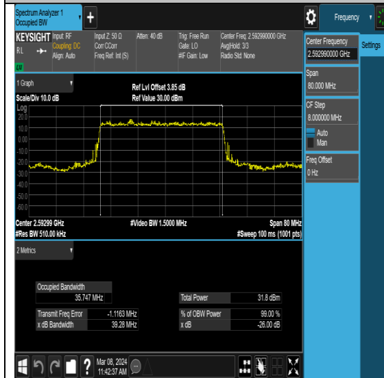
NTNV-N41-PC2-30-40-M-DFT-PI2BPSK-Outer_Full-Ant0-PASS
