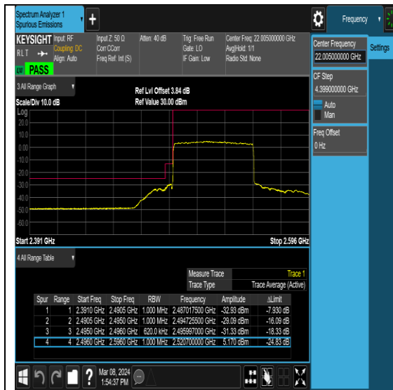
NTNV-N41-PC2-30-60-L-DFT-QPSK-Outter_Full-Ant0-PASS
