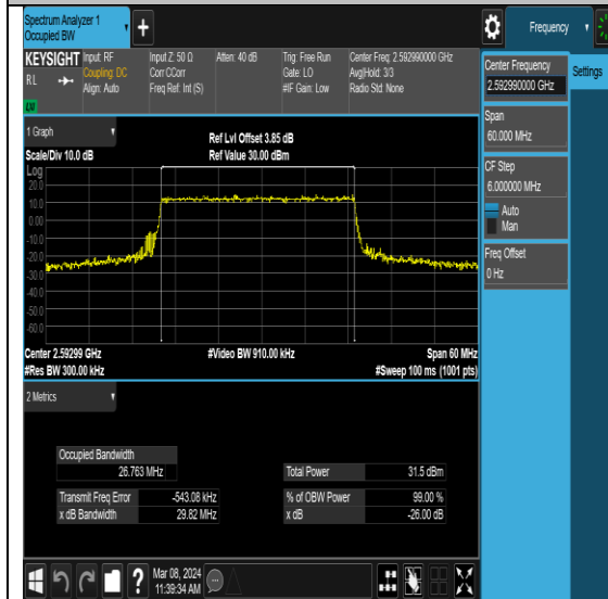
NTNV-N41-PC2-30-30-M-DFT-QPSK-Outer_Full-Ant0-PASS
