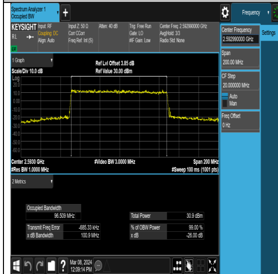
NTNV-N41-PC2-30-100-M-DFT-16QAM-Outer_Full-Ant0-PASS
