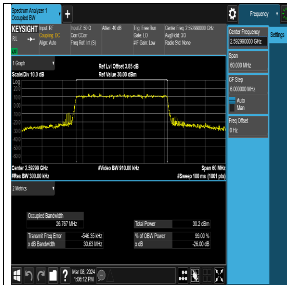
NTNV-N41-PC2-30-30-M-DFT-64QAM-Outer_Full-Ant0-PASS
