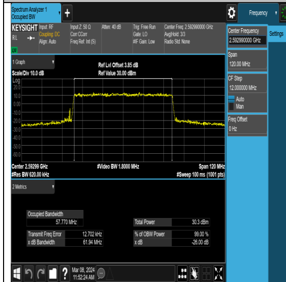
NTNV-N41-PC2-30-60-M-DFT-16QAM-Outer_Full-Ant0-PASS
