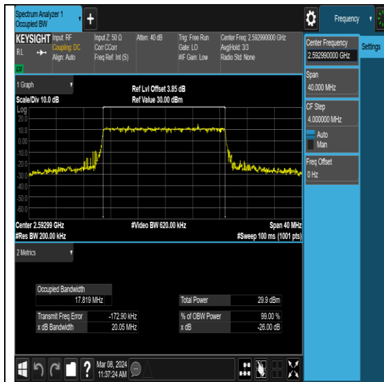
NTNV-N41-PC2-30-20-M-DFT-256QAM-Outer_Full-Ant0-PASS
