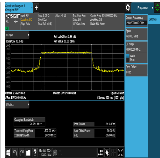
NTNV-N41-PC2-30-30-M-DFT-PI2BPSK-Outer_Full-Ant0-PASS
