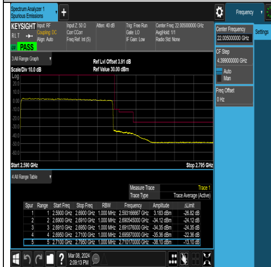
NTNV-N41-PC2-30-100-H-DFT-QPSK-Outet_Full-Ant0-PASS
