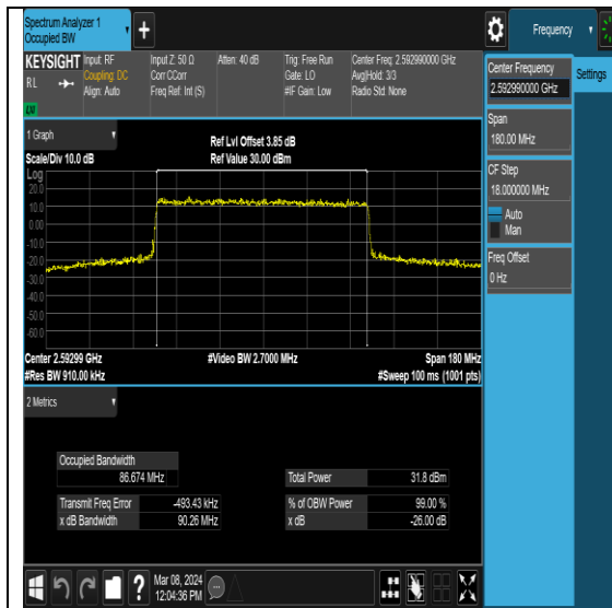
NTNV-N41-PC2-30-90-M-DFT-QPSK-Outer_Full-Ant0-PASS
