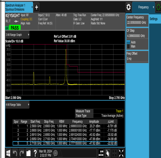
NTNV-N41-PC2-30-60-H-DFT-QPSK-Edge_1RB_Right-Ant0-PASS
