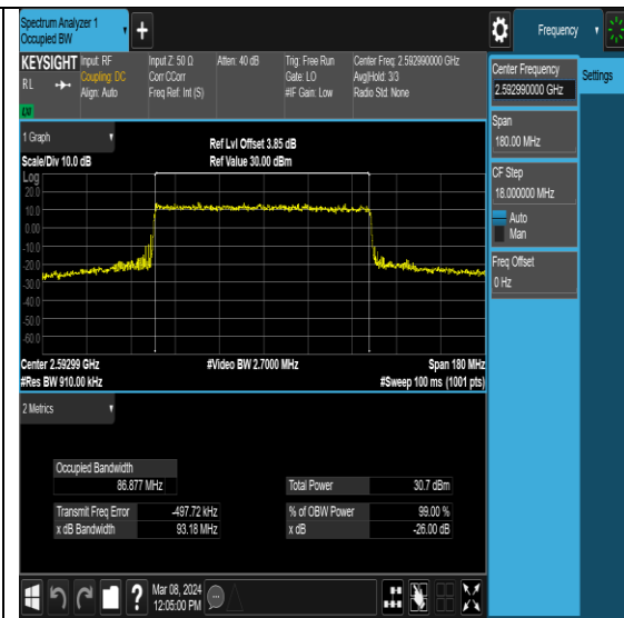
NTNV-N41-PC2-30-90-M-DFT-16QAM-Outer_Full-Ant0-PASS
