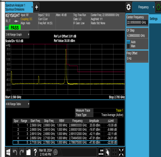
NTNV-N41-PC2-30-100-H-DFT-QPSK-Edge_1RB_Right-Ant0-PASS
