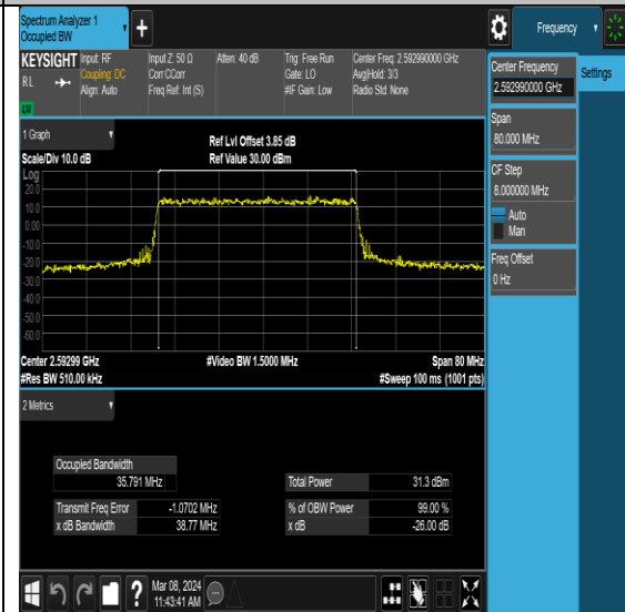
NTNV-N41-PC2-30-40-M-DFT-QPSK-Outer_Full-Ant0-PASS
