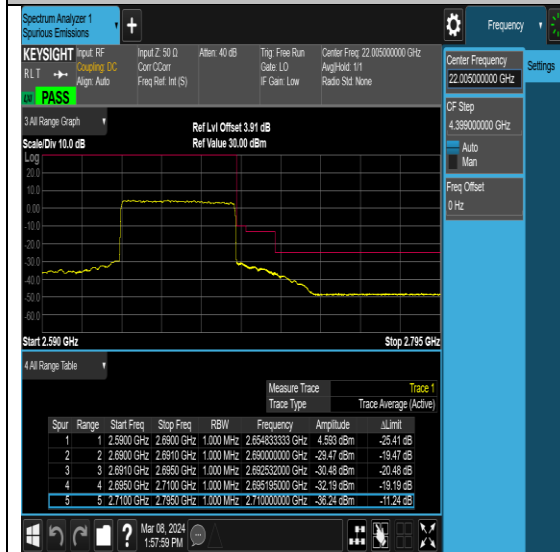
NTNV-N41-PC2-30-60-H-DFT-QPSK-Outter_Full-Ant0-PASS
