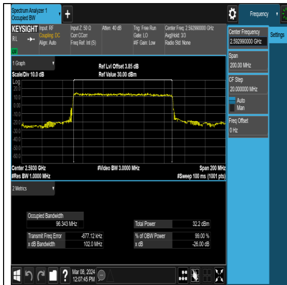
NTNV-N41-PC2-30-100-M-DFT-PI2BPSK-Outer_Full-Ant0-PASS
