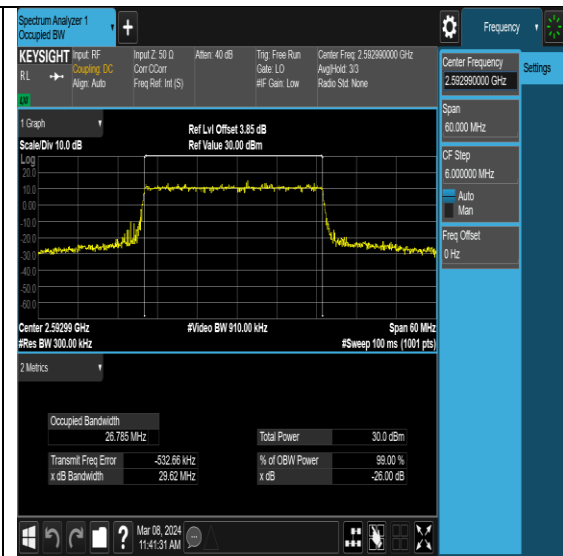
NTNV-N41-PC2-30-30-M-DFT-256QAM-Outer_Full-Ant0-PASS
