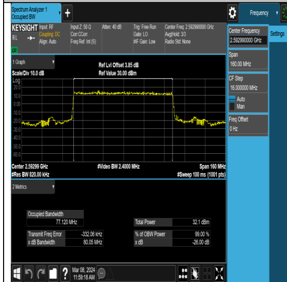
NTNV-N41-PC2-30-80-M-DFT-PI2BPSK-Outer_Full-Ant0-PASS
