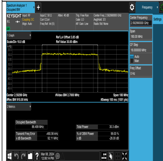
NTNV-N41-PC2-30-90-M-DFT-64QAM-Outer_Full-Ant0-PASS
