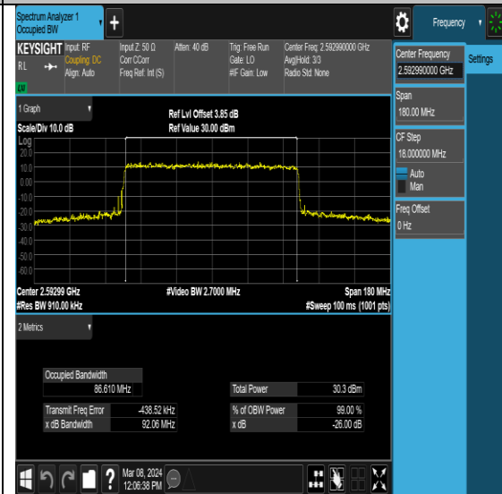
NTNV-N41-PC2-30-90-M-DFT-256QAM-Outer_Full-Ant0-PASS
