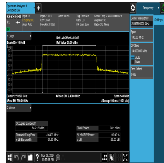
NTNV-N41-PC2-30-70-M-DFT-64QAM-Outer_Full-Ant0-PASS
