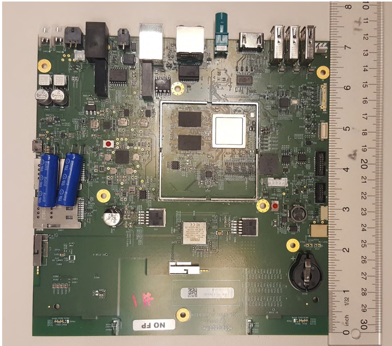
Picture front side of module
