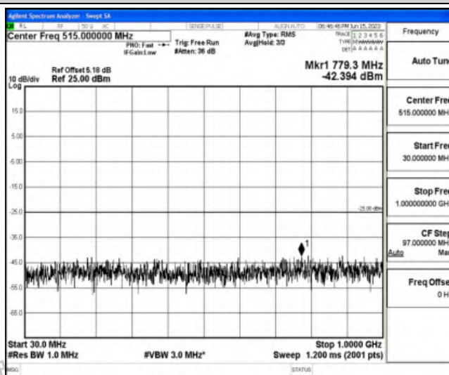
Band41-5MHz-QPSK-41565-1RB#0-Range3:30~1000MHz
