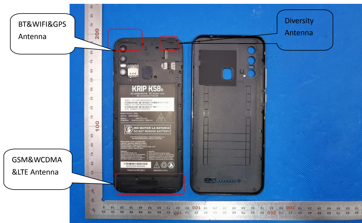
OPEN VIEW OF EUT(FIGURE 2)
