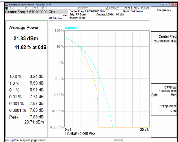
n41 40M DFT-s-OFDM 256QAM Outer_Full High
