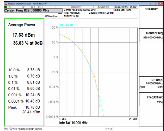
n26(824-849MHz) 10M CP-OFDM 256QAM Outer_Full Low
