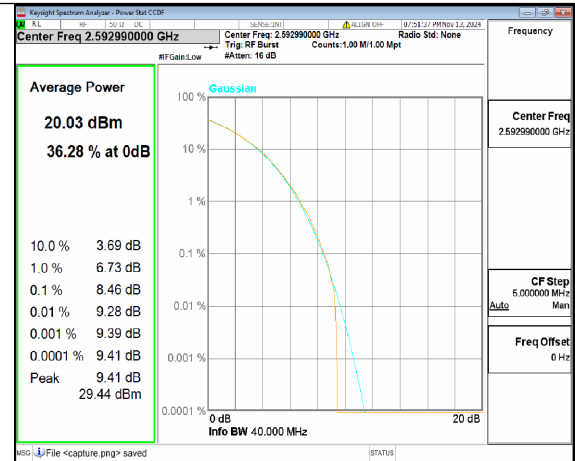
n41 40M CP-OFDM 256QAM Outer_Full Mid
