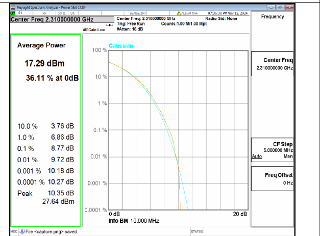
n30 10M CP-OFDM 256QAM Outer_Full Mid
