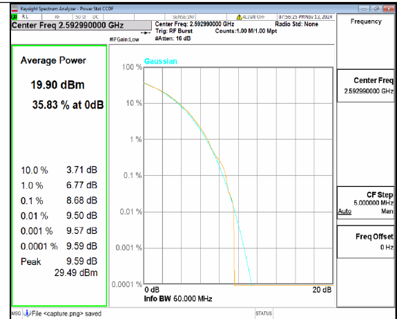
n41 50M CP-OFDM 256QAM Outer_Full Mid
