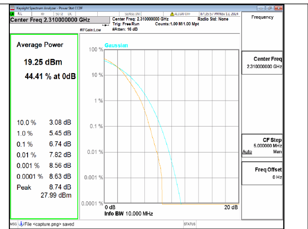
n30 10M DFT-s-OFDM 256QAM Outer_Full Mid
