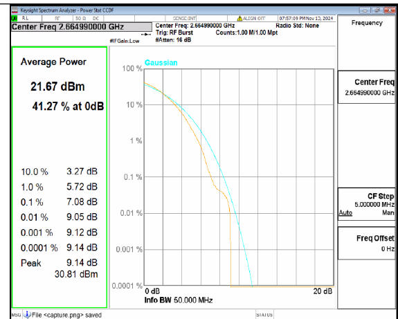
n41 50M DFT-s-OFDM 256QAM Outer_Full High
