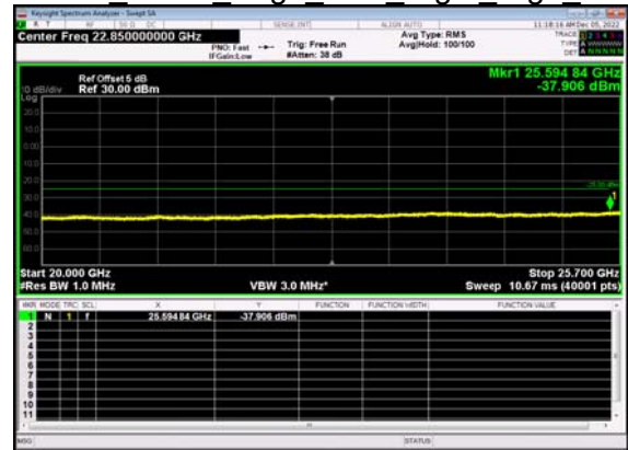
N7(15M)_DFT-s- OFDM BPSK Edge 1RB Right High CH
