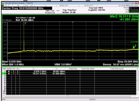
N38(10M)_DFT-s- OFDM BPSK Edge 1RB Right Low CH
