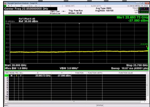
N7(20M)_DFT-s- OFDM QPSK Outer Full Low CH
