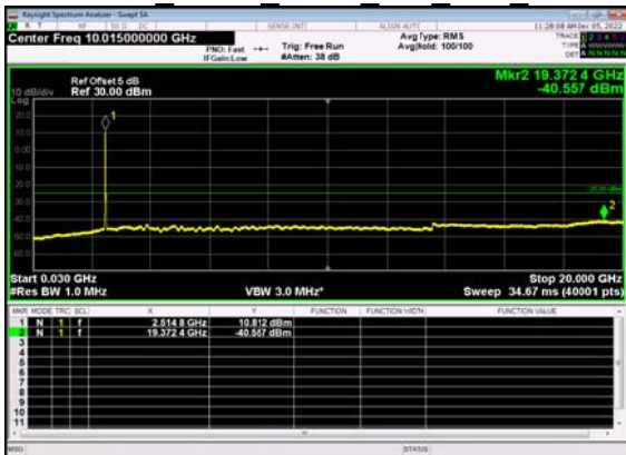
N7(20M)_DFT-s- OFDM BPSK Outer Full Low CH
