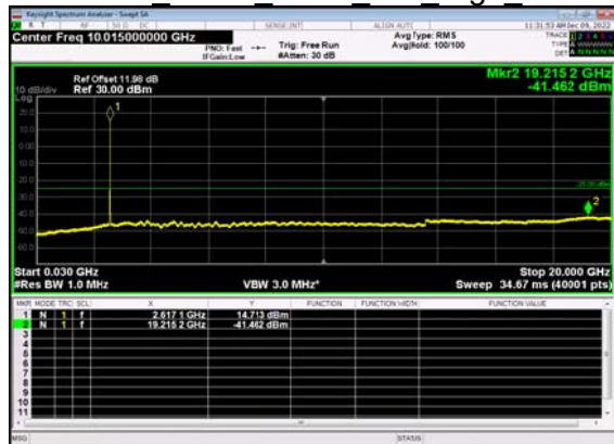
N38(10M)_DFT-s- OFDM BPSK Outer Full High CH
