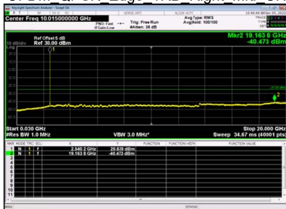
N7(10M)_DFT-s- OFDM QPSK Edge 1RB Right Mid CH
