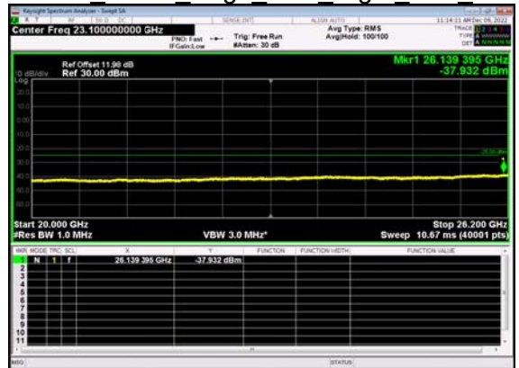
N38(10M)_DFT-s- OFDM BPSK Edge 1RB Right Low CH
