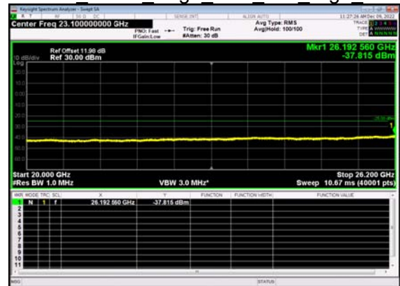
N38(10M)_DFT-s- OFDM BPSK Edge 1RB Left High CH
