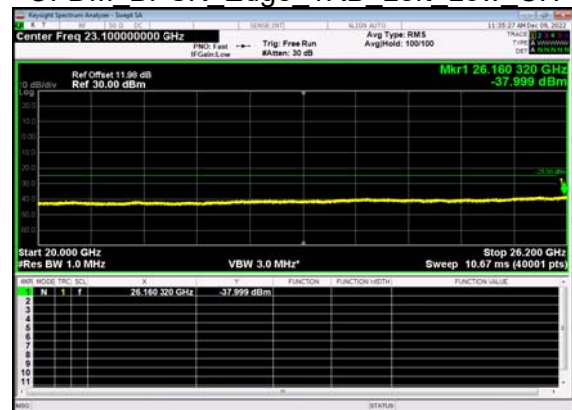
N38(15M)_DFT-s- OFDM BPSK Edge 1RB Left Low CH
