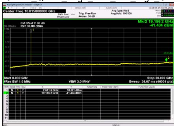
N38(10M)_DFT-s- OFDM QPSK Edge 1RB Left High CH
