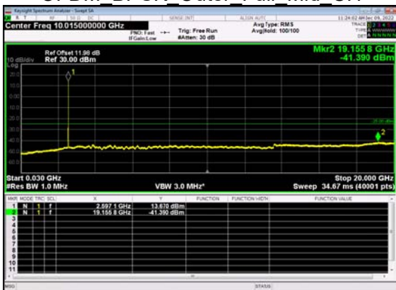
N38(10M)_DFT-s- OFDM BPSK Outer Full Mid CH
