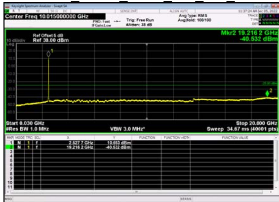
N7(20M)_DFT-s- OFDM QPSK Outer Full Mid CH
