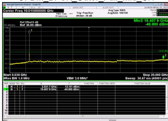
N7(10M)_DFT-s- OFDM BPSK Outer Full Mid CH
