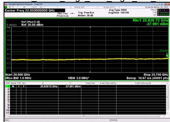
N7(10M)_DFT-s- OFDM BPSK Edge 1RB Right Mid CH
