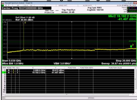
N38(10M)_DFT-s- OFDM BPSK Edge 1RB Right Mid CH
