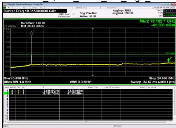
N38(10M)_DFT-s- OFDM QPSK Outer Full High CH
