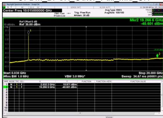
N7(20M)_DFT-s- OFDM BPSK Outer Full Mid CH
