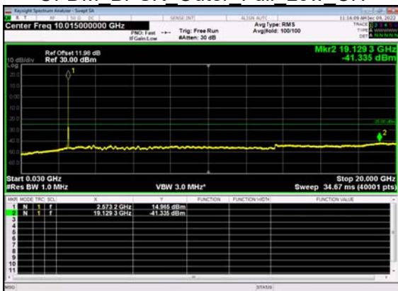
N38(10M)_DFT-s- OFDM BPSK Outer Full Low CH
