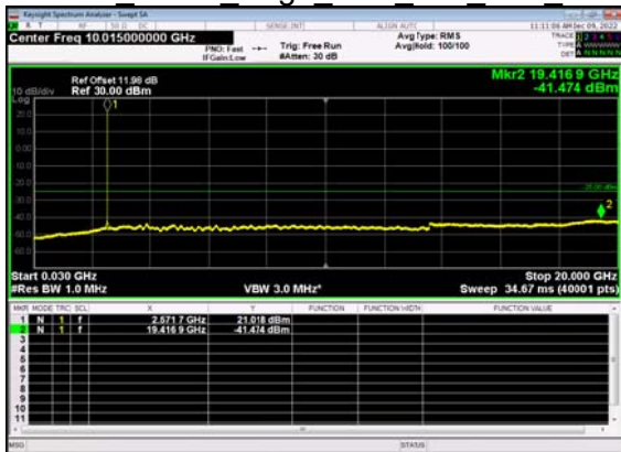
N38(10M)_DFT-s- OFDM BPSK Edge 1RB Left Low CH
