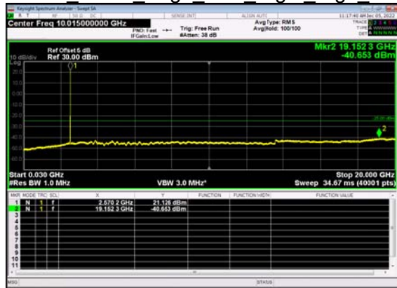
N7(15M)_DFT-s- OFDM BPSK Edge 1RB Right High CH
