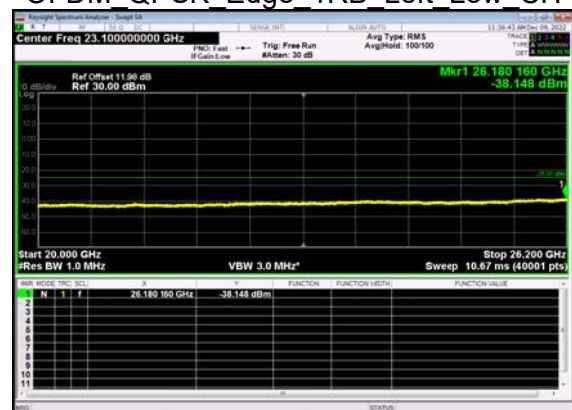
N38(15M)_DFT-s- OFDM QPSK Edge 1RB Left Low CH
