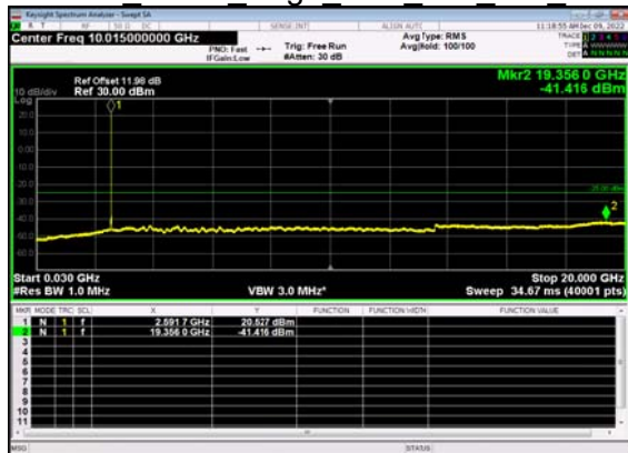
N38(10M)_DFT-s- OFDM BPSK Edge 1RB Left Mid CH
