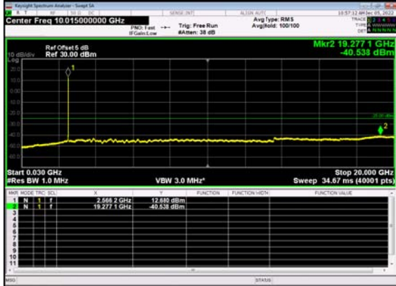
N7(10M)_DFT-s- OFDM QPSK Outer Full High CH
