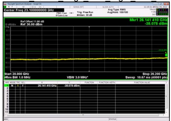
N38(10M)_DFT-s- OFDM QPSK Edge 1RB Right Low CH
