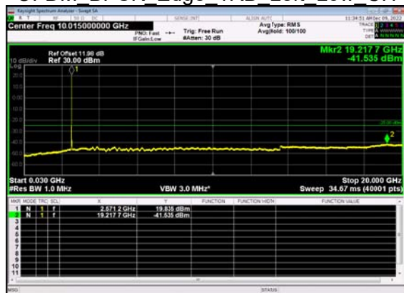
N38(15M)_DFT-s- OFDM BPSK Edge 1RB Left Low CH
