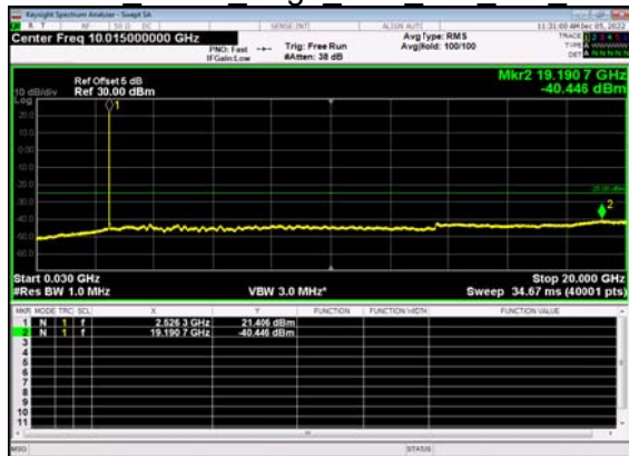
N7(20M)_DFT-s- OFDM BPSK Edge 1RB Left Mid CH
