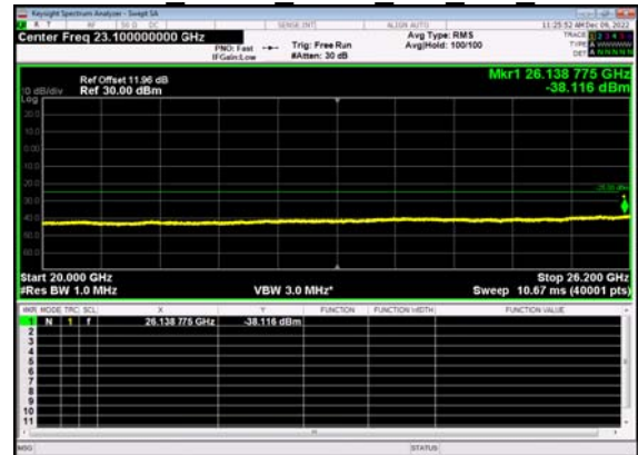
N38(10M)_DFT-s- OFDM QPSK Outer Full Mid CH
