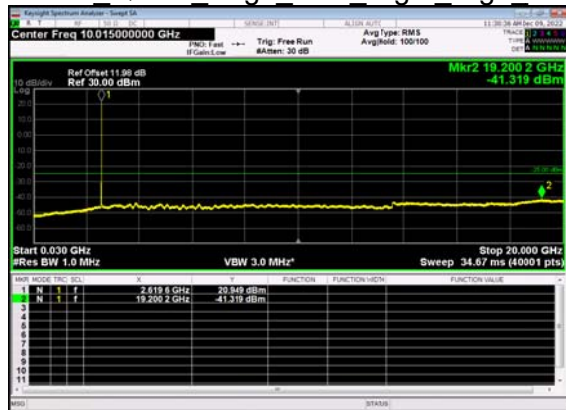
N38(10M)_DFT-s- OFDM QPSK Edge 1RB Right High CH
