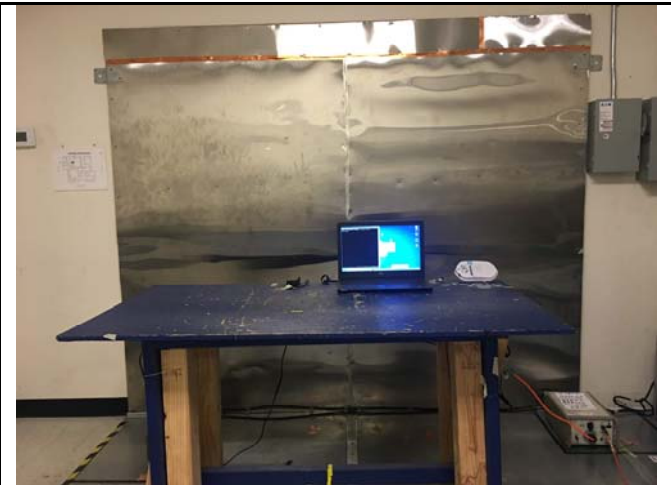
Conducted Emission- Rear View
