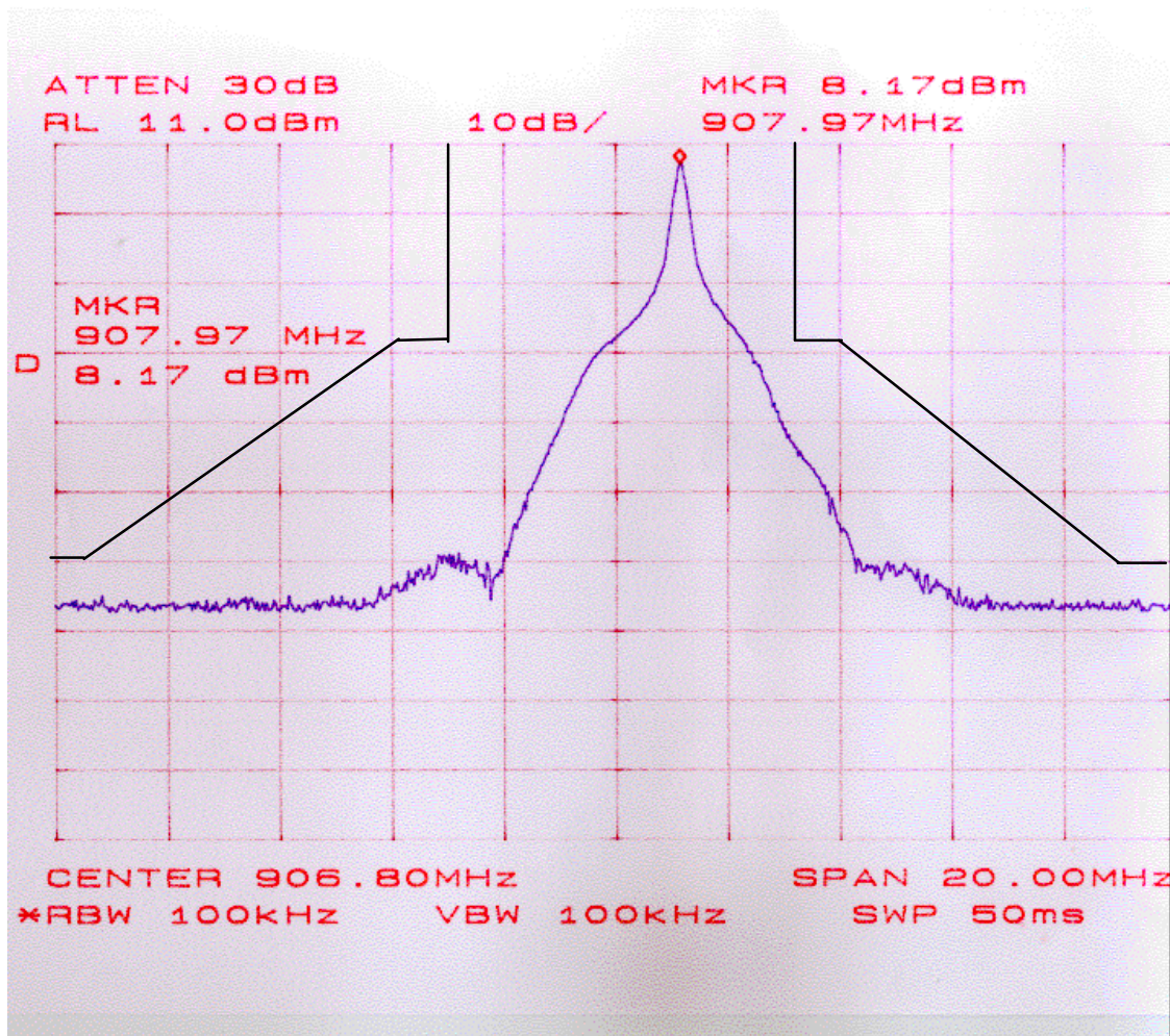
Plot 1.3.1 Emission mask
