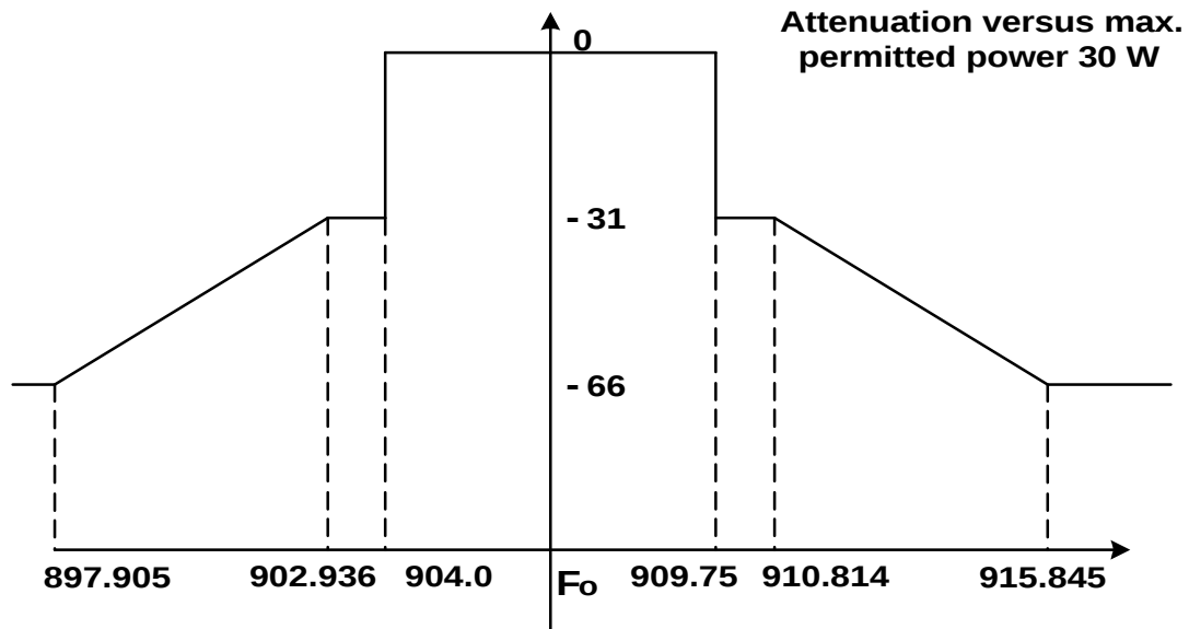
Figure 1.3.2 Emission mask ( F_0 = 906.875 MHz) Attenuation versus emitted power (see Plot 1.3.1)
