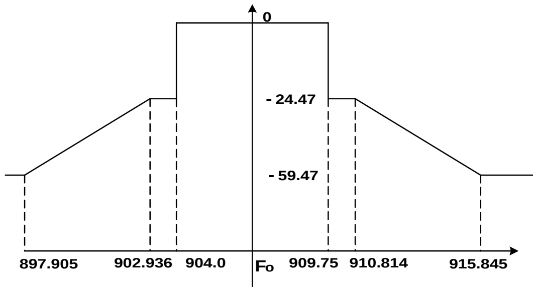
Figure 1.3.2 Emission mask ( F_0 = 906.875 MHz) Attenuation versus emitted power (see Plot 1.3.1)
