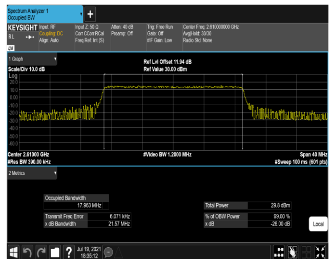
Band38-20MHz-16QAM-38150-100RB#0
