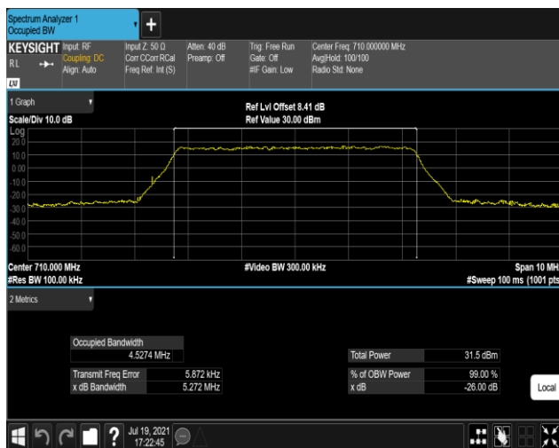
Band17-5MHz-16QAM-23790-25RB#0
