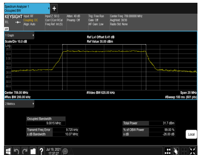
Band17-10MHz-16QAM-23800-50RB#0
