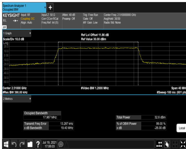
Band7-20MHz-QPSK-21350-100RB#0
