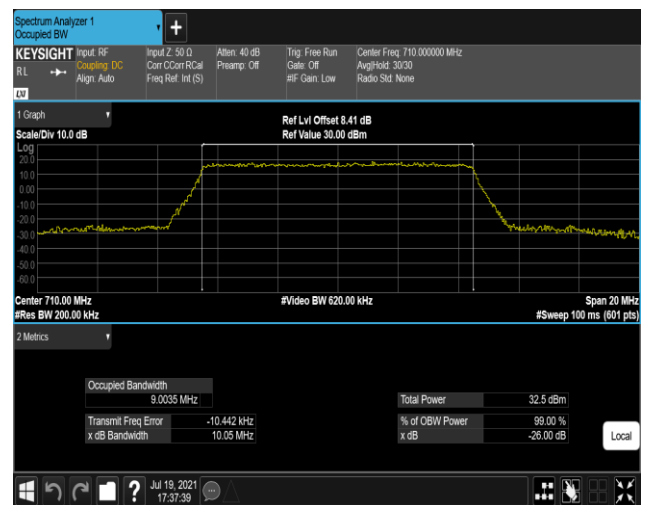
Band17-10MHz-16QAM-23780-50RB#0
