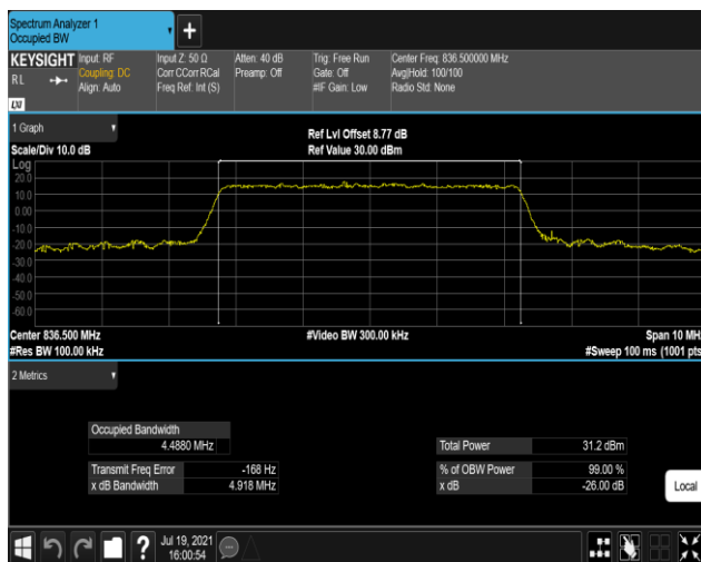
Band5-5MHz-16QAM-20525-25RB#0
