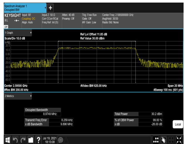
Band38-10MHz-16QAM-37800-50RB#0
