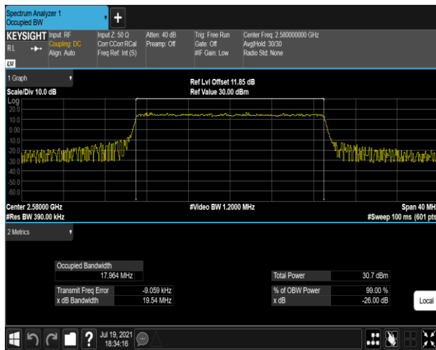
Band38-20MHz-QPSK-38150-100RB#0
