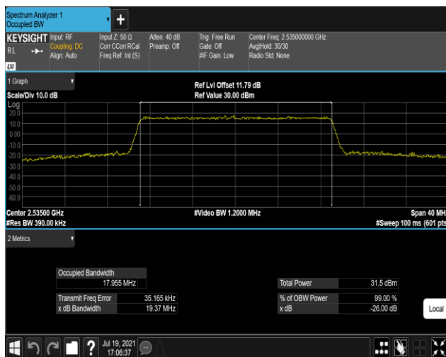
Band7-20MHz-16QAM-21100-100RB#0
