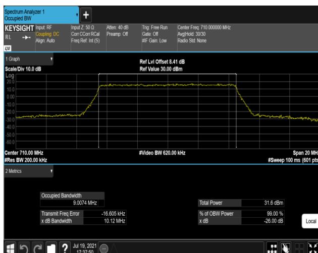
Band17-10MHz-16QAM-23790-50RB#0
