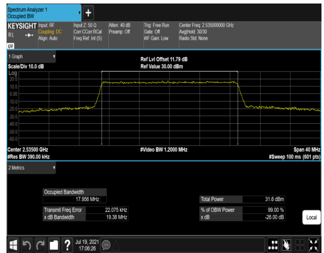
Band7-20MHz-16QAM-20850-100RB#0
