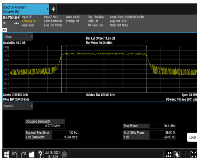
Band38-10MHz-16QAM-38000-50RB#0
