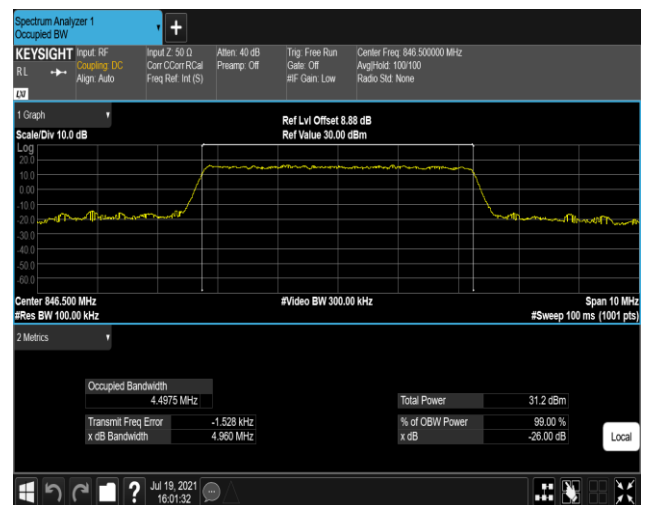
Band5-5MHz-16QAM-20625-25RB#0
