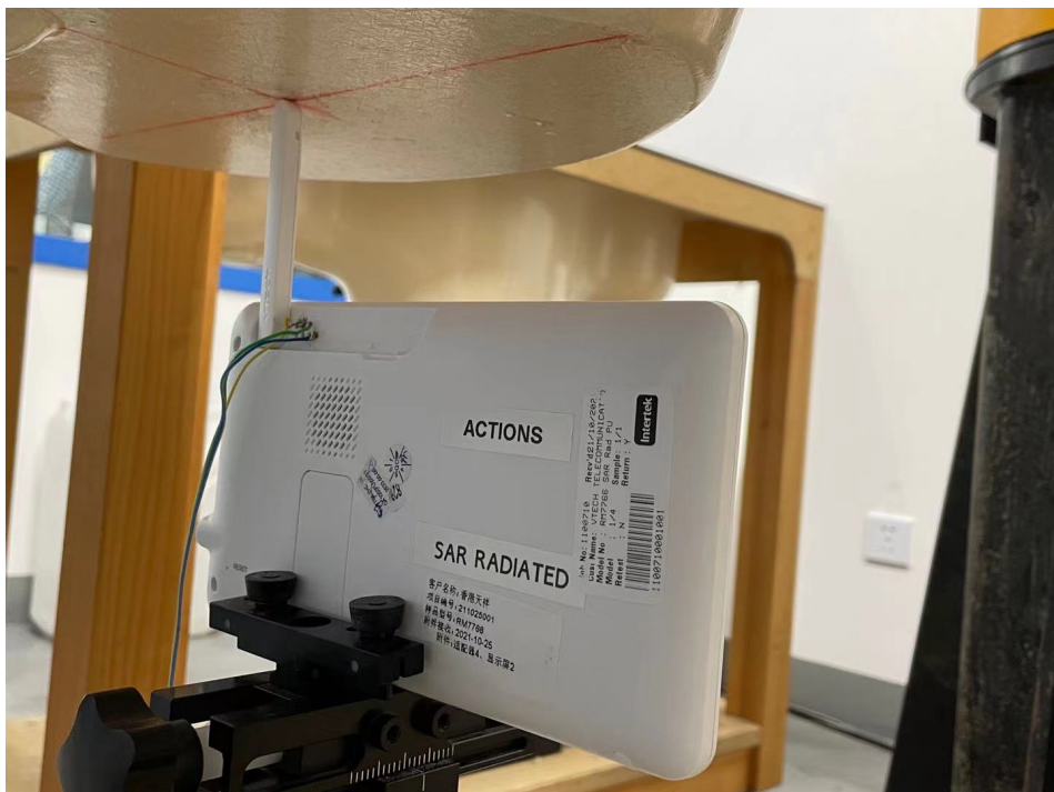
Figure 8 – Top with 0mm Separation (antenna extended)
