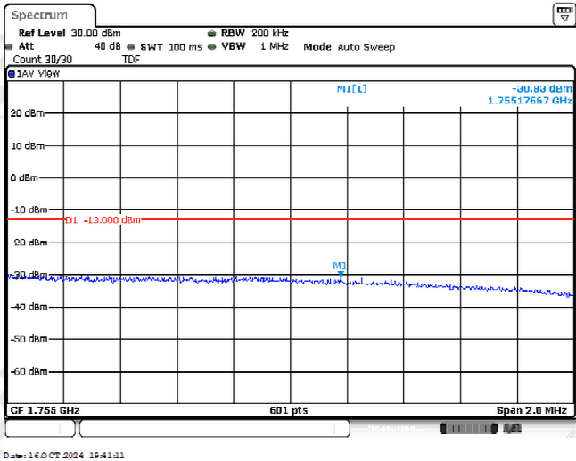
Band4-10MHz-16QAM-20350-1RB#24
