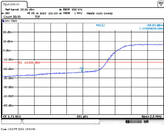
Band4-10MHz-16QAM-20000-25RB#0
