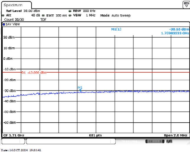
Band4-10MHz-16QAM-20000-1RB#24
