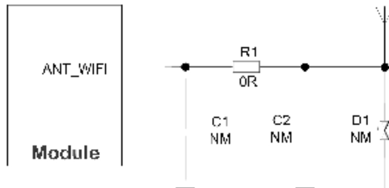
Figure 5: Reference Circuit for RF Antenna Interface
