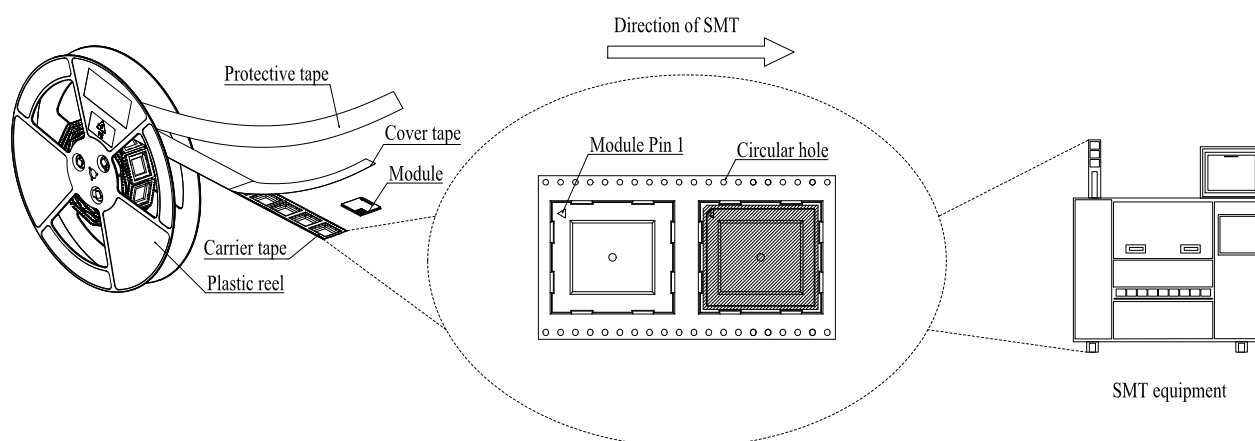
Figure 28: Mounting Direction
