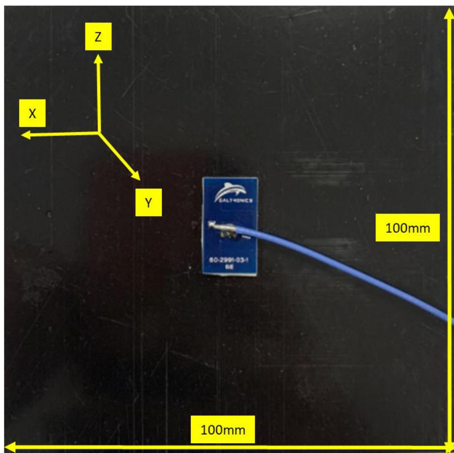
Figure 3 Measurement Orientation
