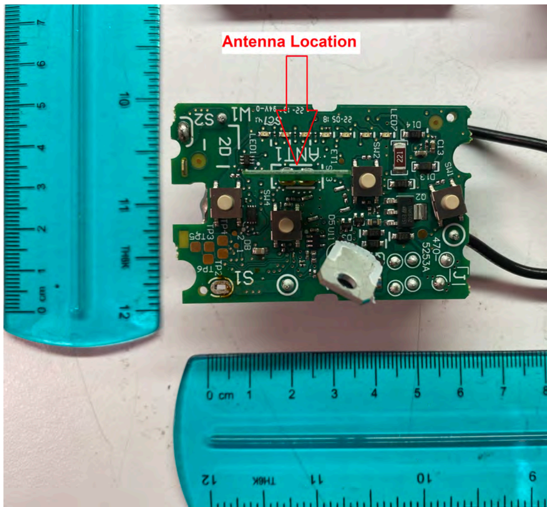
Top PCB (antenna location)
