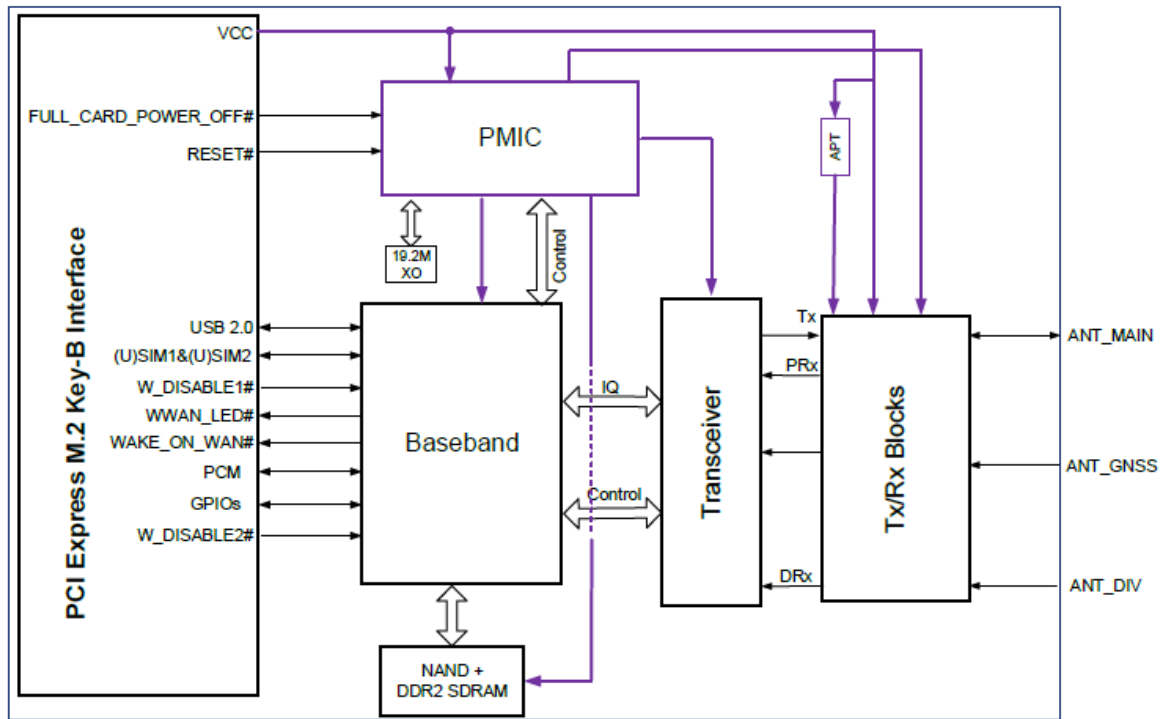
Figure 1: Functional Diagram
