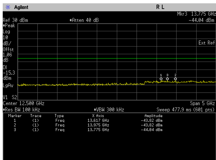
Conducted Emissions(Peak). Bluetooth LE, Frequency 2440 Emission Level, 10 GHz -> 15 GHz
