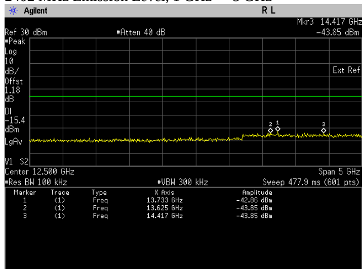
Conducted Emissions(Peak). Bluetooth LE, Frequency 2402 MHz Emission Level, 10 GHz -> 15 GHz
