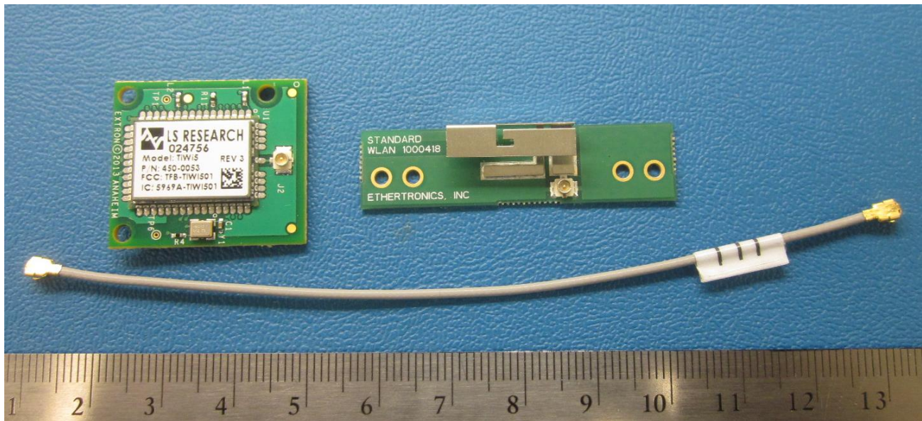
Figure C.1.3 – EUT with Antenna and RF cable View 1
