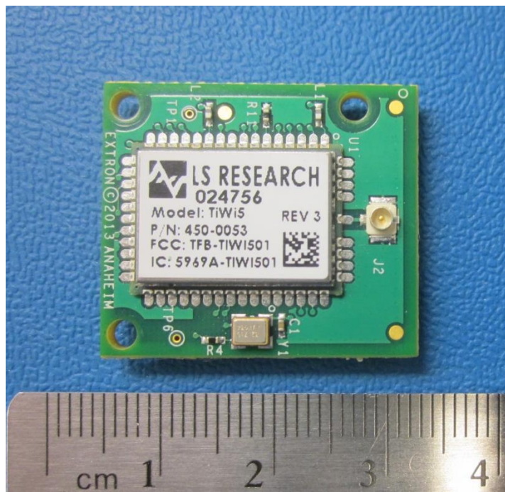
Figure C.1.1 - EUT Top View
