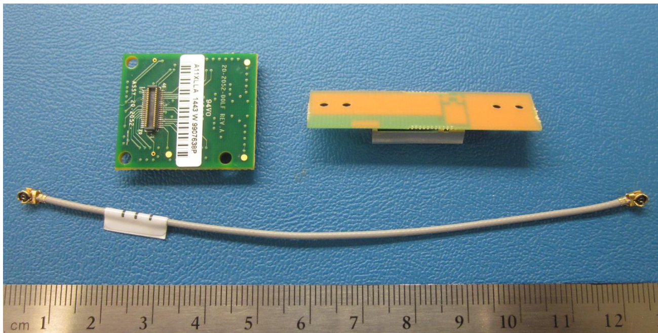
Figure C.1.4 – EUT with Antenna and RF cable View 2
