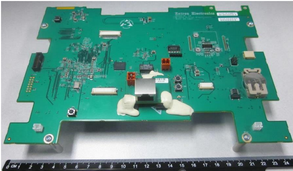
Figure C.2.1- Control Board
