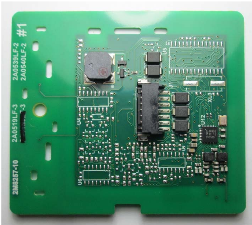
T12 Mifare - PCB (Rear Side)
