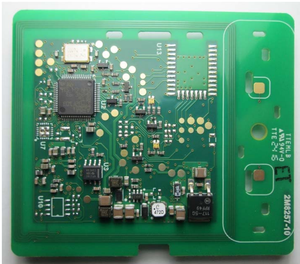
T12 Mifare - PCB (Front Side)
