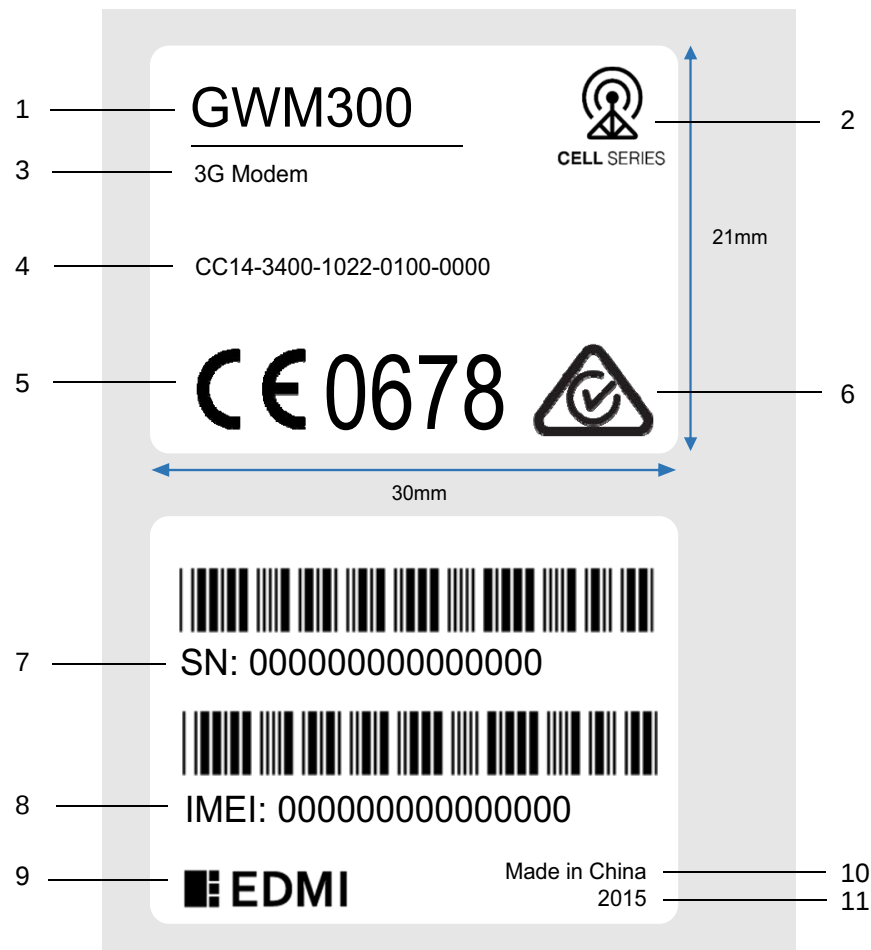
Figure 1: Sample GWM300 labels
