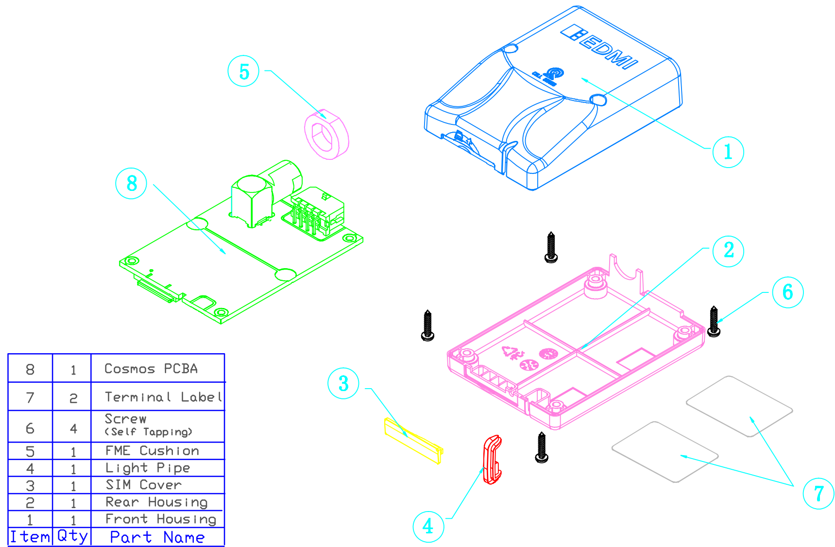
Figure 9: GWM300 exploded view
