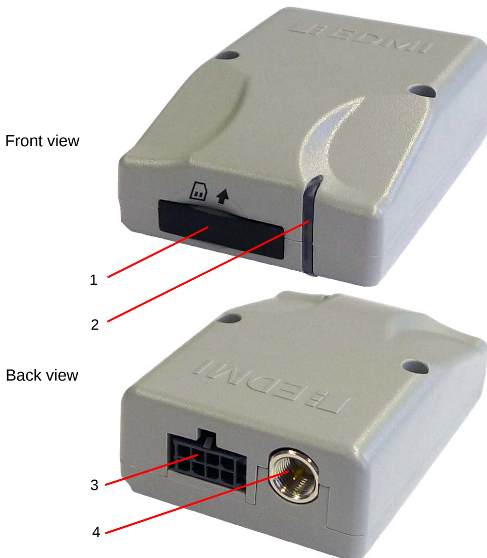
Figure 2: GWM300 interfaces
