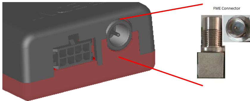
Figure 7: Antenna connector
