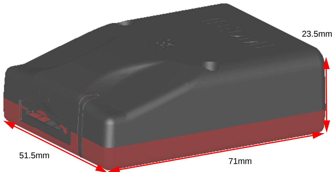
Figure 8: GWM300 3D overview
