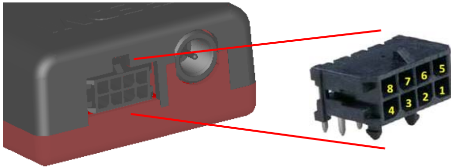
Figure 4: Pin assignment Molex Microfit
