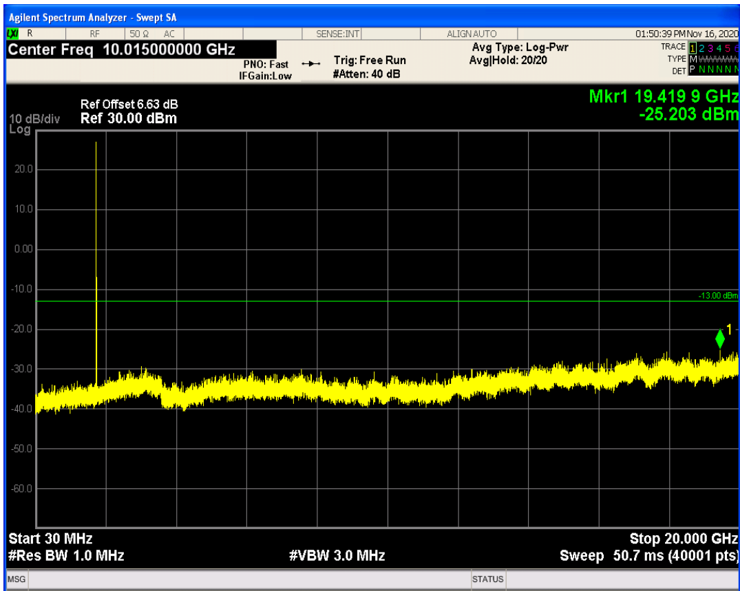
LTE Band4 QPSK BW=1.4MHz Channel=20393 RB Size=6 Position=#0
