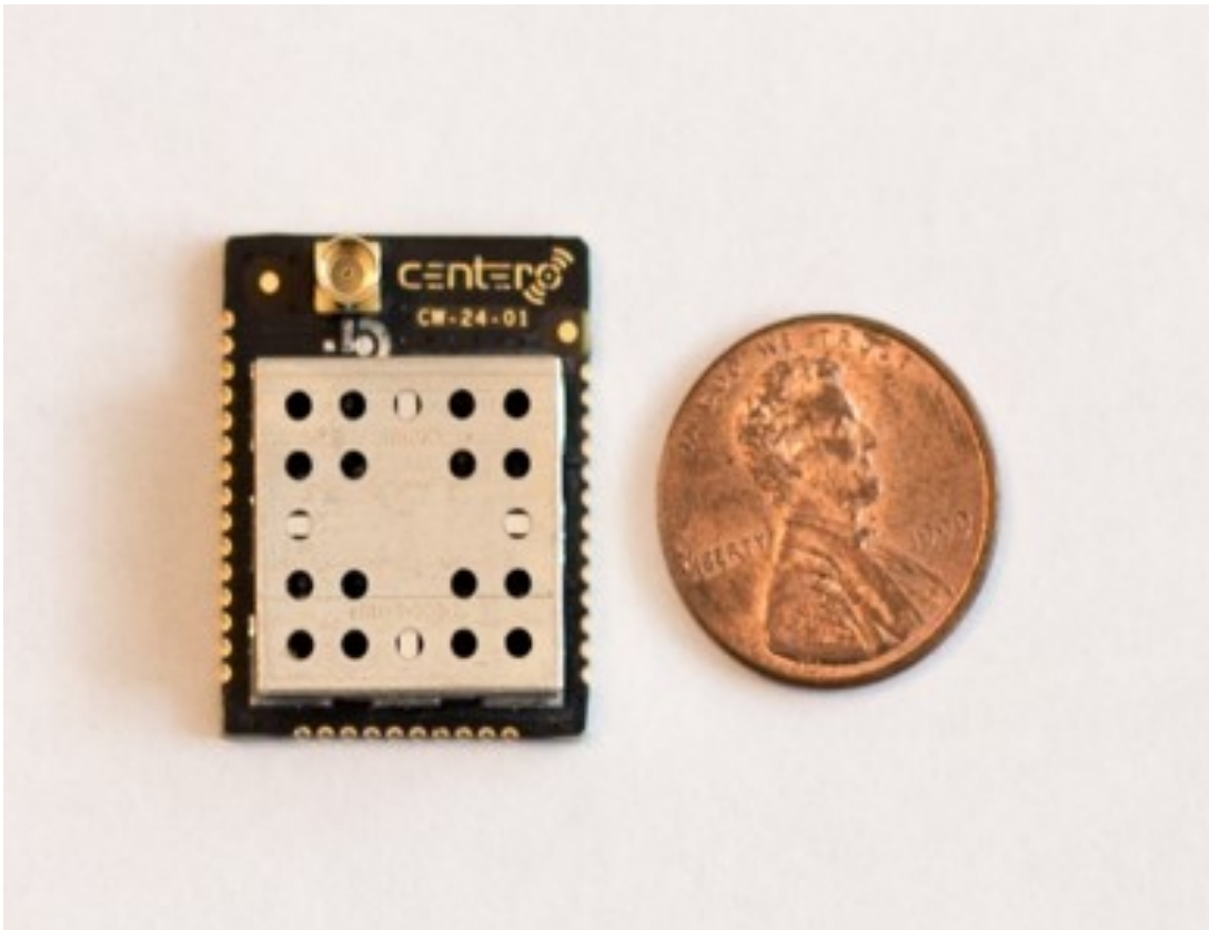
Figure 1. Top of 2.4 GHz ISA Radio, PCB Component View (With Shield)
