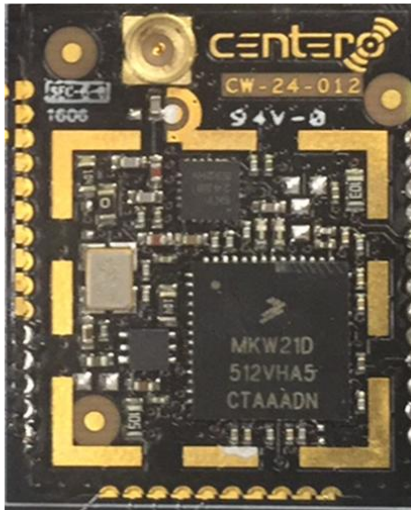
Figure 2. Top of 2.4 GHz ISA Radio, PCB Component View (Without Shield)
