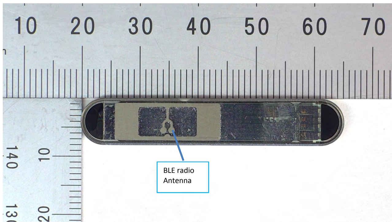
Figure 6 LINQ II Back View
