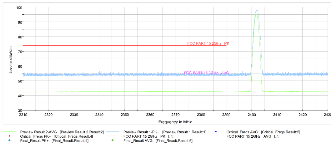
Fig.13. Frequency Band Edges: GFSK, Channel 0, 2.31 GHz – 2.43GHz
