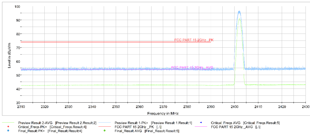
Fig.15. Frequency Band Edges: \pi/4 DQPSK, Channel 0, 2.31 GHz - 2.43GHz
