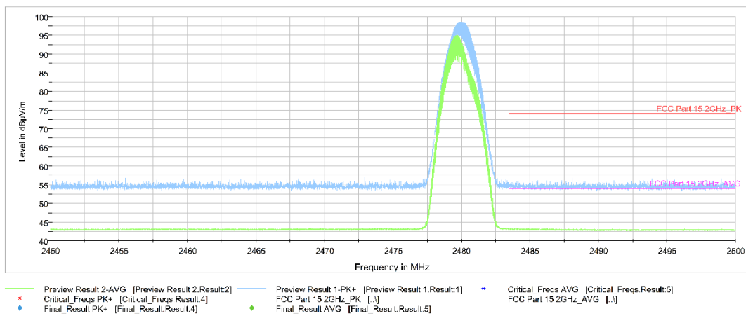
Fig.16. Frequency Band Edges: \pi/4 DQPSK, Channel 78, 2.45 GHz - 2.50GHz
