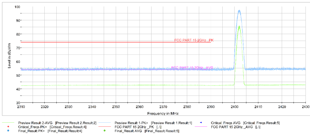
Fig.17. Frequency Band Edges: 8DPSK, Channel 0, 2.31 GHz - 2.43GHz
