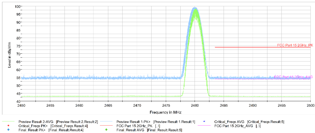
Fig.14. Frequency Band Edges: GFSK, Channel 78, 2.45 GHz - 2.50GHz
