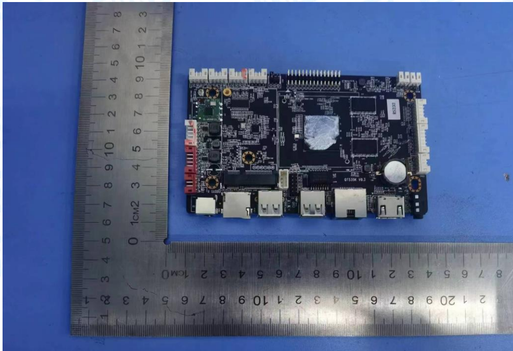
Photo 22 Appearance of PCB
