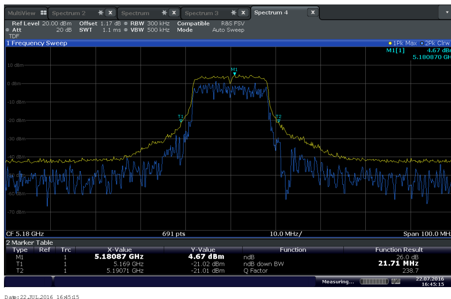
Low Channel U-NII 1 802.11a
