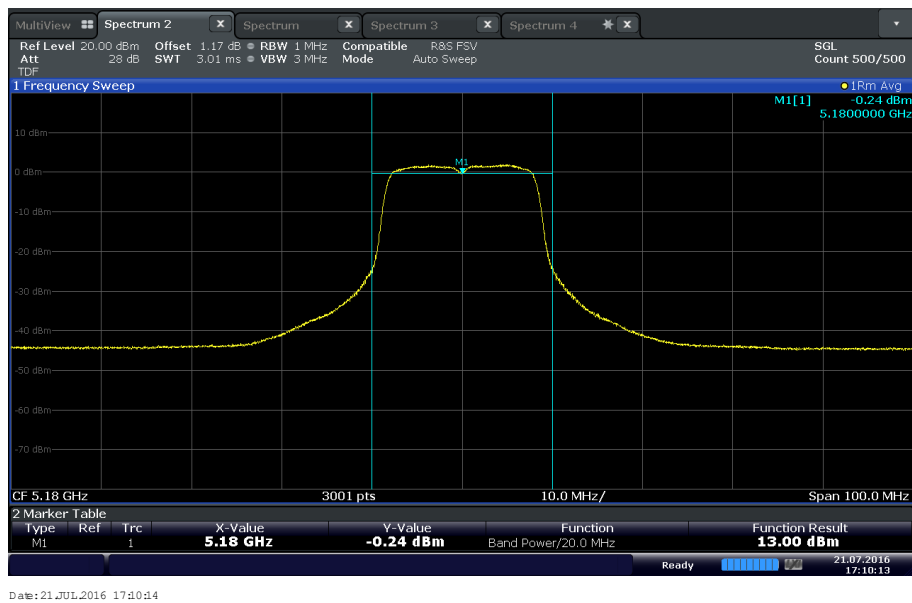
Low Channel, 802.11a U-NII 1 HT20 18 Mbps
