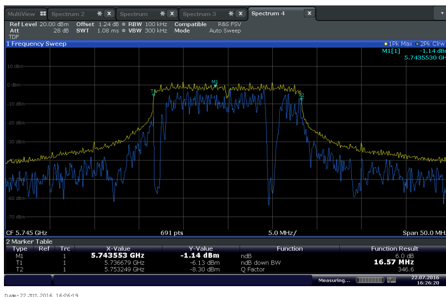
Low Channel U-NII 3 802.11a
