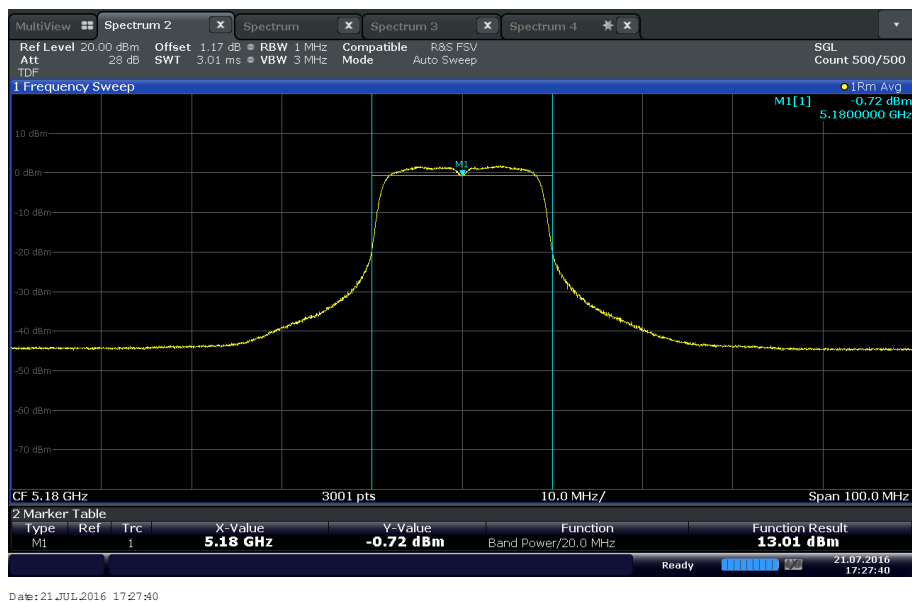
Low Channel, 802.11n U-NII 1 HT20 MCS6 58.5 Mbps
