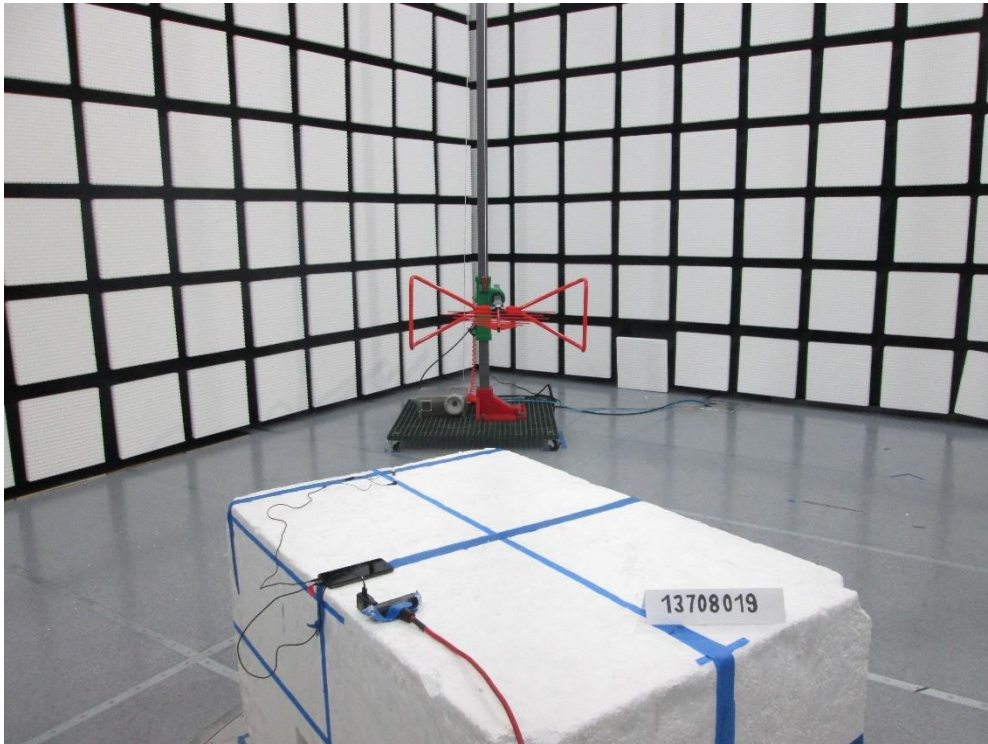
RADIATED BACK PHOTO (BELOW 1GHz)
