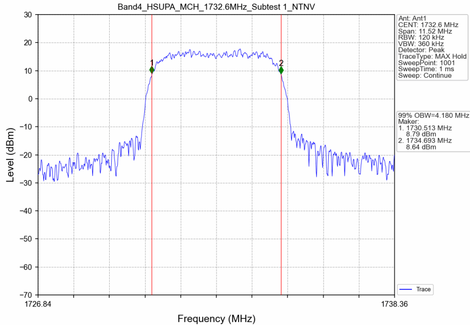
Band IV_HSUPA_MCH_1732.6MHz_Subtest 1_NTNV
