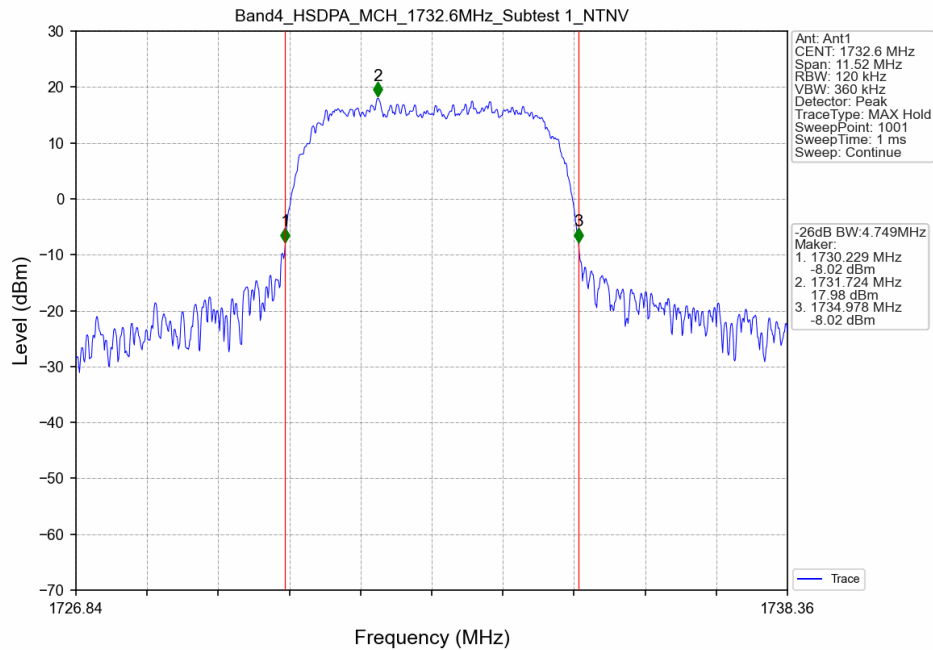
Band IV_HSDPA_MCH_1732.6MHz_Subtest 1_NTNV
