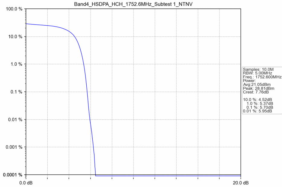
Band IV_HSDPA_HCH_1752.6MHz_Subtest 1_NTNV
