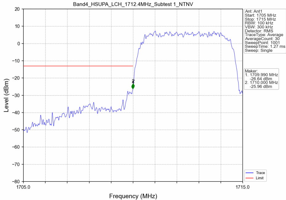
Band IV_HSUPA_LCH_1712.4MHz_Subtest 1_NTNV
