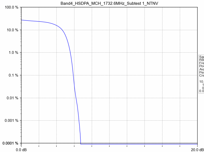
Band IV_HSDPA_MCH_1732.6MHz_Subtest 1_NTNV
