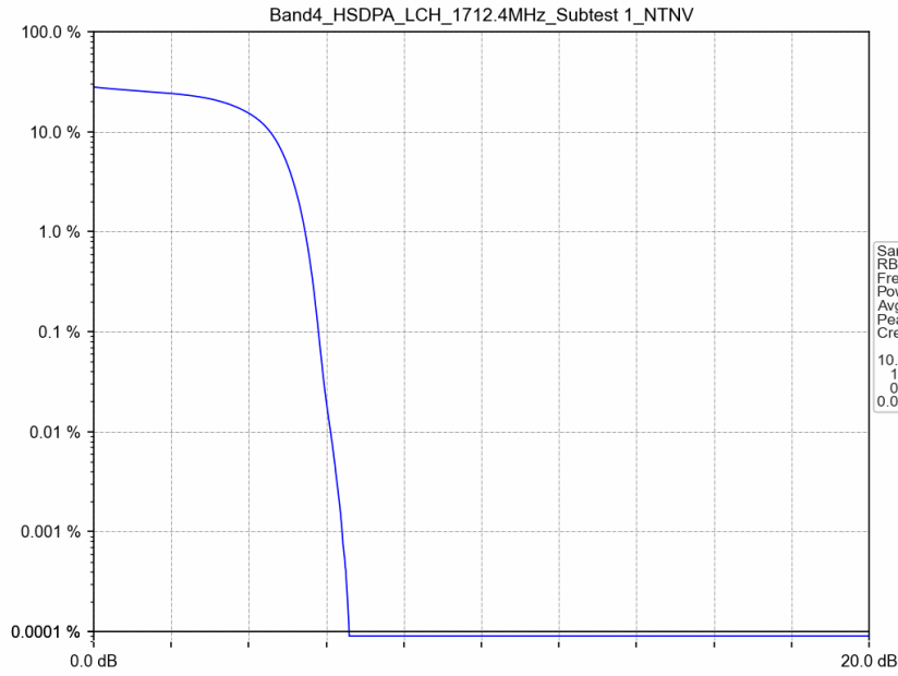
Band IV_HSDPA_LCH_1712.4MHz_Subtest 1_NTNV
