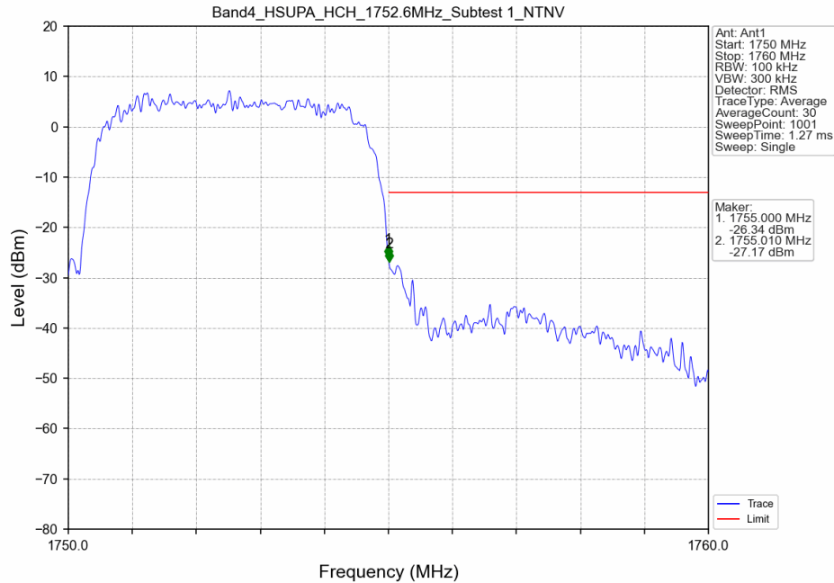
Band IV_HSUPA_HCH_1752.6MHz_Subtest 1_NTNV
