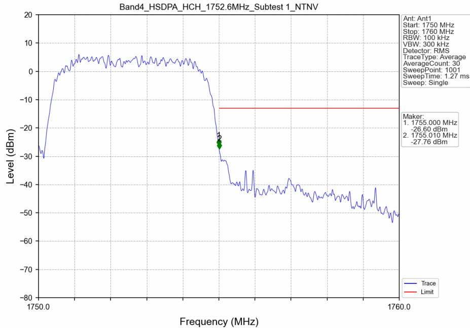
Band IV_HSDPA_HCH_1752.6MHz_Subtest 1_NTNV
