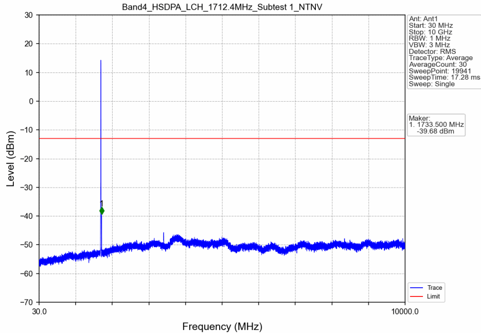
Band IV_HSDPA_LCH_1712.4MHz_Subtest 1_NTNV
