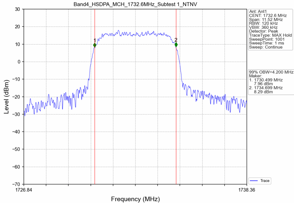
Band IV_HSDPA_MCH_1732.6MHz_Subtest 1_NTNV
