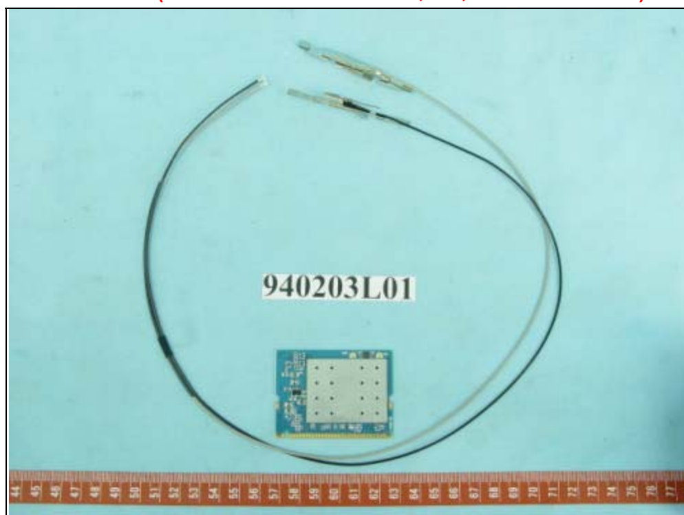
Antenna 1 (Brand: NISSEI Electric Co., Ltd, P/N: CP115407-01)
