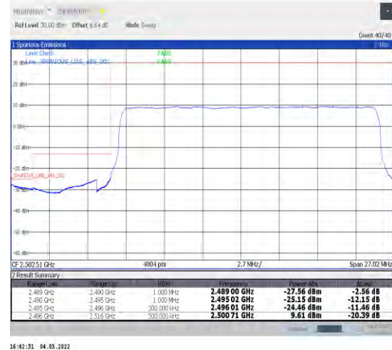
1-N41--30-20-L-3-DFT-PI2BPSK-Outer_Full-50@0-Ant1-PASS-see graph
