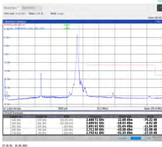
1-N41--30-50-H-5-CP-QPSK-Edge_1RB_Right-1@132 -Ant1-PASS-see graph
