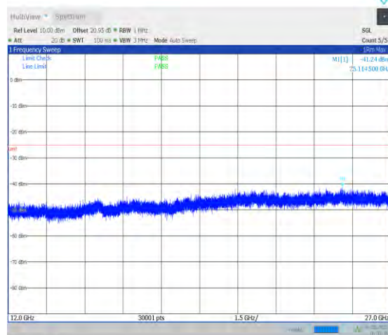
1-N41--30-100-L-1-DFT-PI2BPSK-Inner_1RB_Left-1 @1-12000-27000-Ant1--41.24--25-PASS
