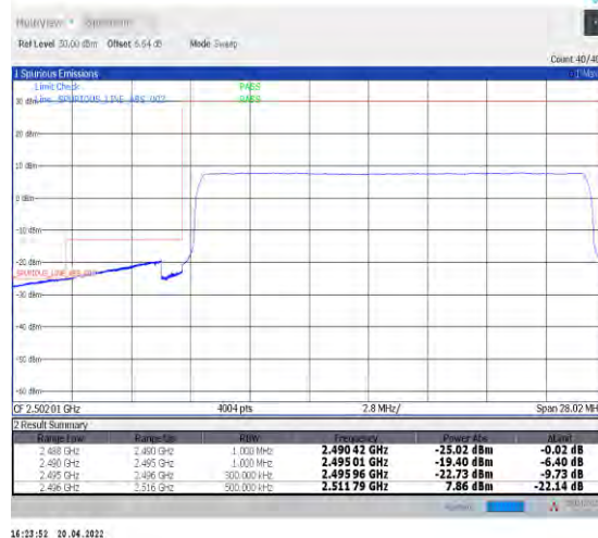
1-N41--30-20-L-6-CP-QPSK-Outer_Full-51@0-Ant1-PASS-see graph
