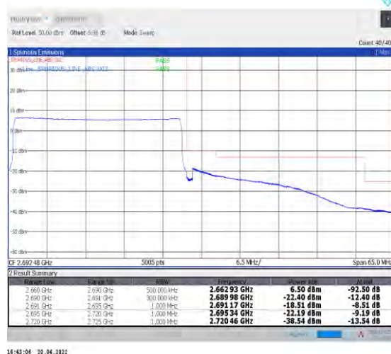
1-N41--30-30-H-6-CP-QPSK-Outer_Full-78@0-Ant1-PASS-see graph
