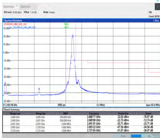
1-N41-PC1-30-30-H-2-DFT-PI2BPSK-Edge_1RB_Right-t1@77-Ant1-1--PASS-see graph
