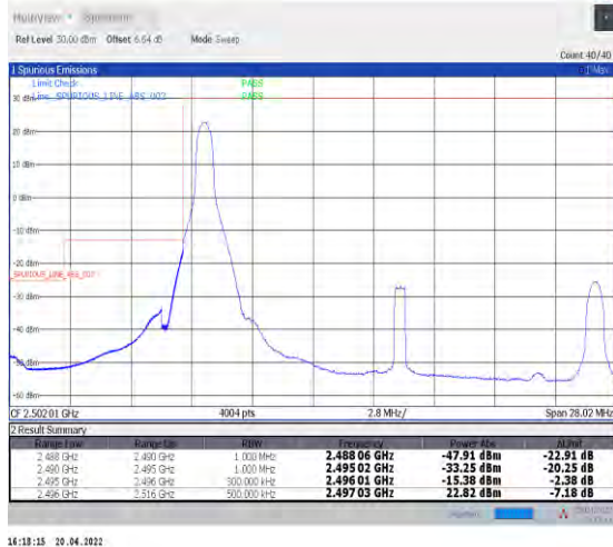
1-N41--30-20-L-1-DFT-PI2BPSK-Edge_1RB_Left-1@0-Ant1-PASS-see graph
