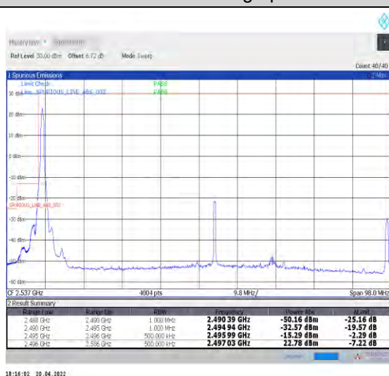
1-N41--30-90-L-4-CP-QPSK-Edge_1RB_Left-1@0-Ant1-PASS-see graph
