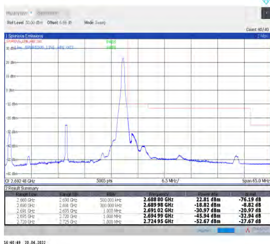
1-N41--30-30-H-5-CP-QPSK-Edge_1RB_Right-1@77-Ant1-PASS-see graph
