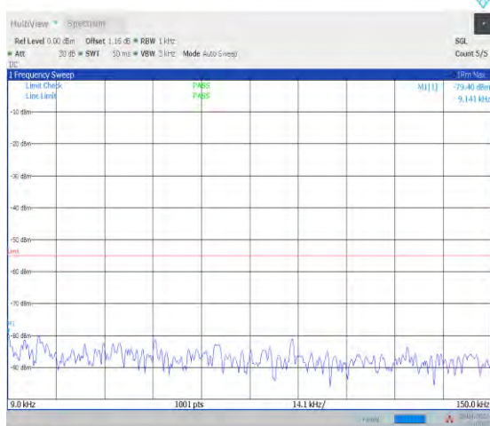
1-N41--30-100-M-1-DFT-PI2BPSK-Inner_1RB_Left-1 @1-0.009-0.15-Ant1--79.40--55-PASS
