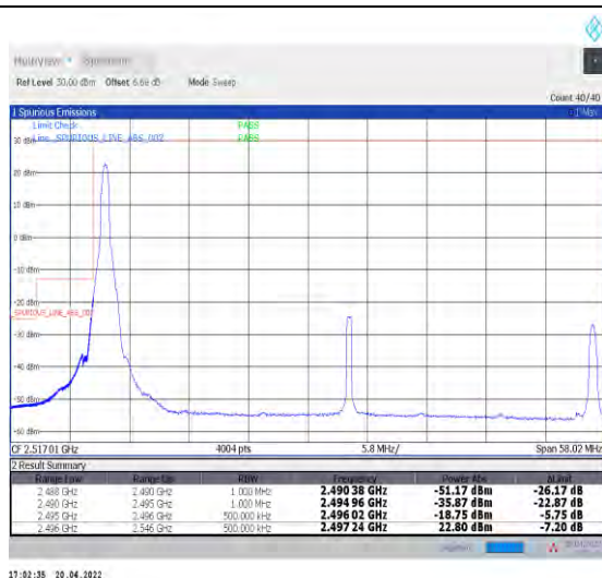
1-N41--30-50-L-1-DFT-PI2BPSK-Edge_1RB_Left-1@0-Ant1-PASS-see graph
