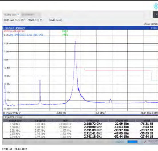
1-N41--30-50-H-2-DFT-PI2BPSK-Edge_1RB_Right-1@ 132-Ant1-PASS-see graph
