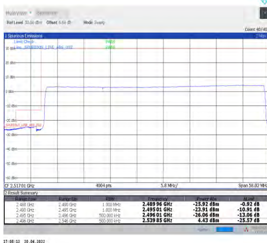
1-N41--30-50-L-6-CP-QPSK-Outer_Full-133@0-Ant1-PASS-see graph
