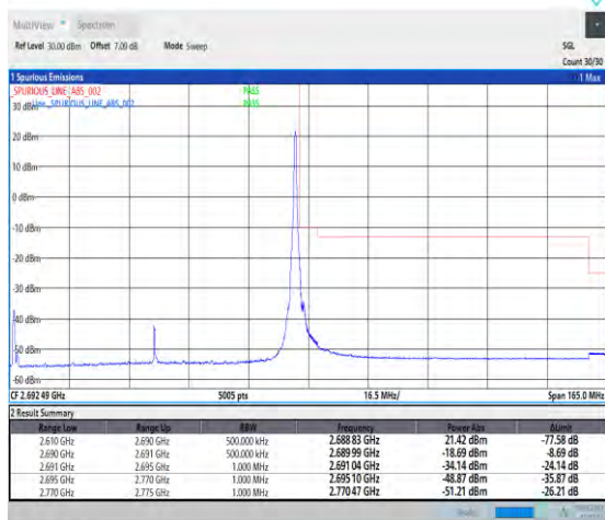
1-N41-PC1-30-80-H-2-DFT-PI2BPSK-Edge_1RB_Right-t-1@216-Ant1-1--PASS-see graph
