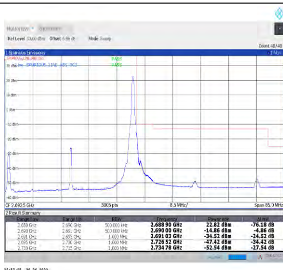
1-N41--30-40-H-2-DFT-PI2BPSK-Edge_1RB_Right-1@ 105-Ant1-PASS-see graph
