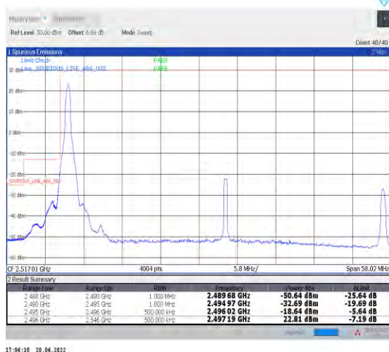
1-N41--30-50-L-4-CP-QPSK-Edge_1RB_Left-1@0-Ant1-PASS-see graph
