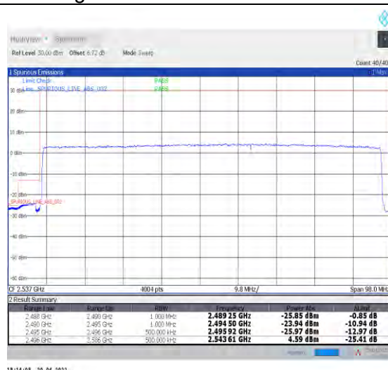
1-N41--30-90-L-3-DFT-PI2BPSK-Outer_Full-240@0-Ant1-PASS-see graph
