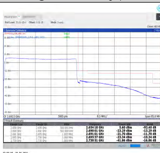
1-N41--30-40-H-6-CP-QPSK-Outer_Full-106@0-A nt1-PASS-see graph
