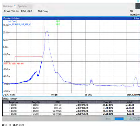
1-N41-PC1-30-20-L-1-DFT-PI2BPSK-Edge_1RB_Left-1@0-Ant1-1--PASS-see graph
