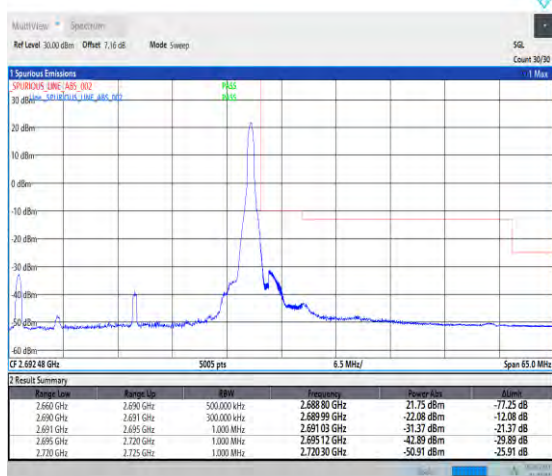
1-N41-PC1-30-30-H-5-CP-QPSK-Edge_1RB_Right-1@77-Ant1-1--PASS-see graph
