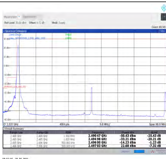
1-N41--30-90-L-1-DFT-PI2BPSK-Edge_1RB_Left-1@0-Ant1-PASS-see graph
