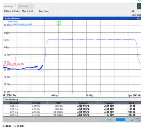
1-N41-PC1-30-20-L-3-DFT-PI2BPSK-Outer_Full-50@0-Ant1-1--PASS-see graph
