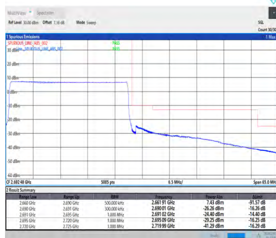
1-N41-PC1-30-30-H-6-CP-QPSK-Outer_Full-78@0-Ant1-1--PASS-see graph
