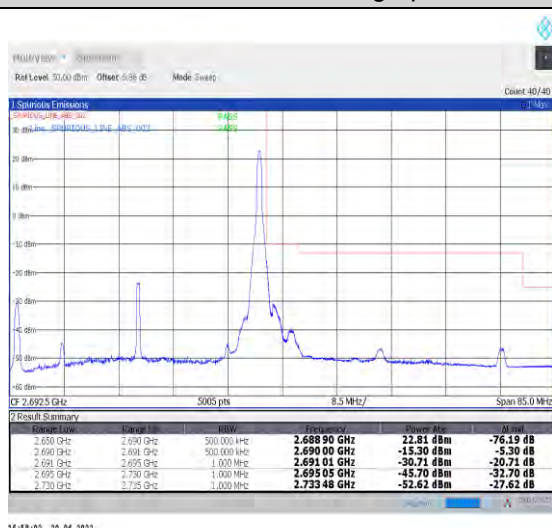
1-N41--30-40-H-5-CP-QPSK-Edge_1RB_Right-1@105 -Ant1-PASS-see graph
