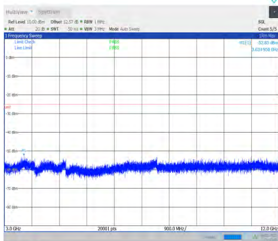
1-N41--30-100-L-1-DFT-PI2BPSK-Inner_1RB_Left-1 @1-3000-12000-Ant1--52.85--25-PASS
