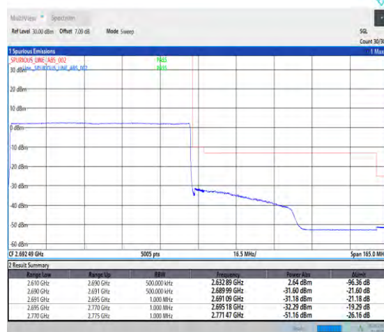
1-N41-PC1-30-80-H-6-CP-QPSK-Outer_Full-217@0-Ant1-1--PASS-see graph
