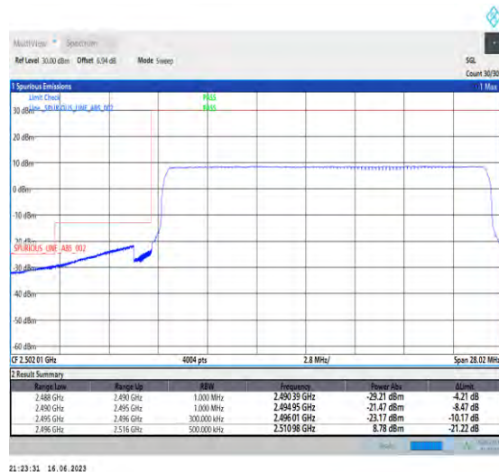
1-N41-PC1-30-20-L-6-CP-QPSK-Outer_Full-51@0-Ant1-1--PASS-see graph
