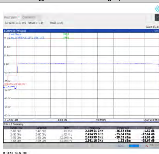
1-N41--30-90-L-6-CP-QPSK-Outer_Full-245@0-Ant1-PASS-see graph
