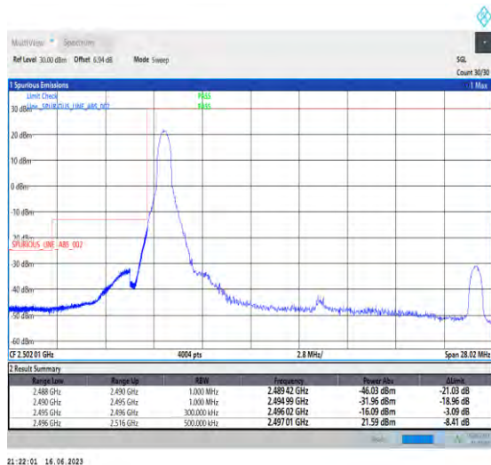
1-N41-PC1-30-20-L-4-CP-QPSK-Edge_1RB_Left-1@0-Ant1-1--PASS-see graph
