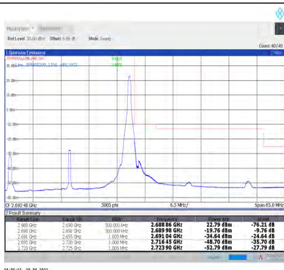
1-N41--30-30-H-2-DFT-PI2BPSK-Edge_1RB_Right-1@77-Ant1-PASS-see graph
