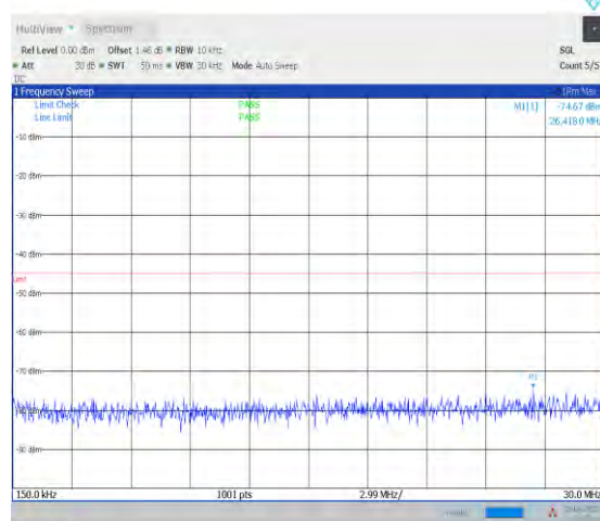
1-N41--30-100-M-1-DFT-PI2BPSK-Inner_1RB_Left-1 @1-0.15-30-Ant1--74.67--45-PASS
