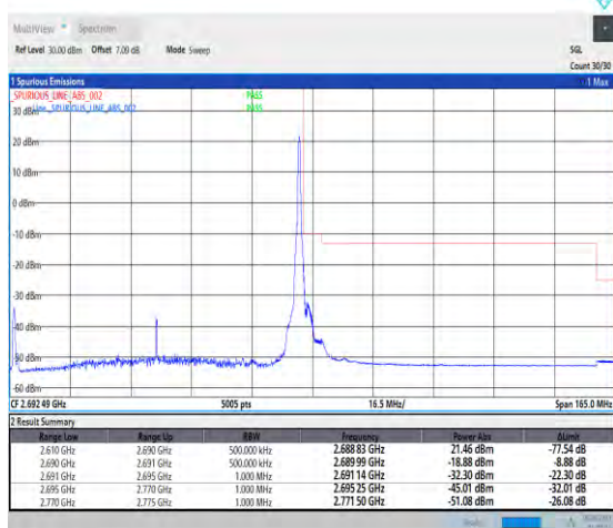
1-N41-PC1-30-80-H-5-CP-QPSK-Edge_1RB_Right-1@216-Ant1-1--PASS-see graph
