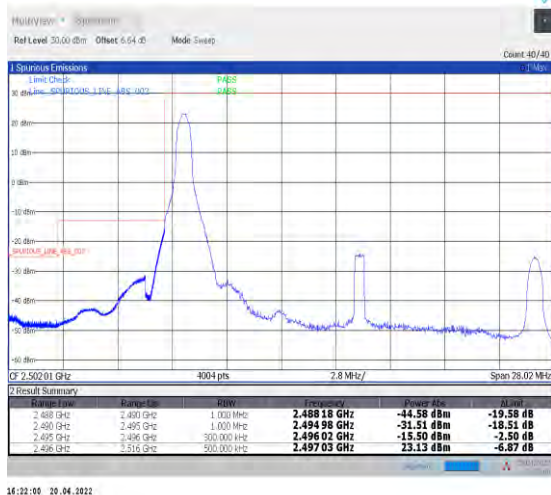
1-N41--30-20-L-4-CP-QPSK-Edge_1RB_Left-1@0-Ant1-PASS-see graph
