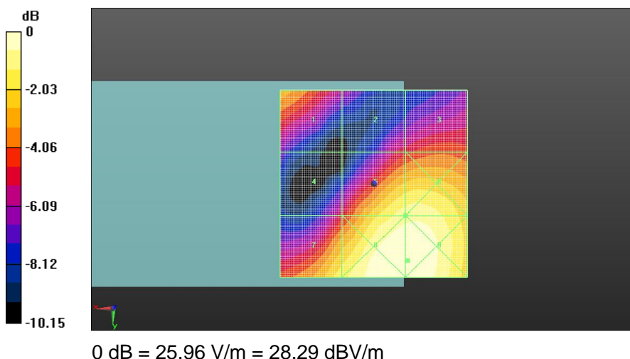
Fig A.6 HAC RF E-Field GSM 1900 Low
