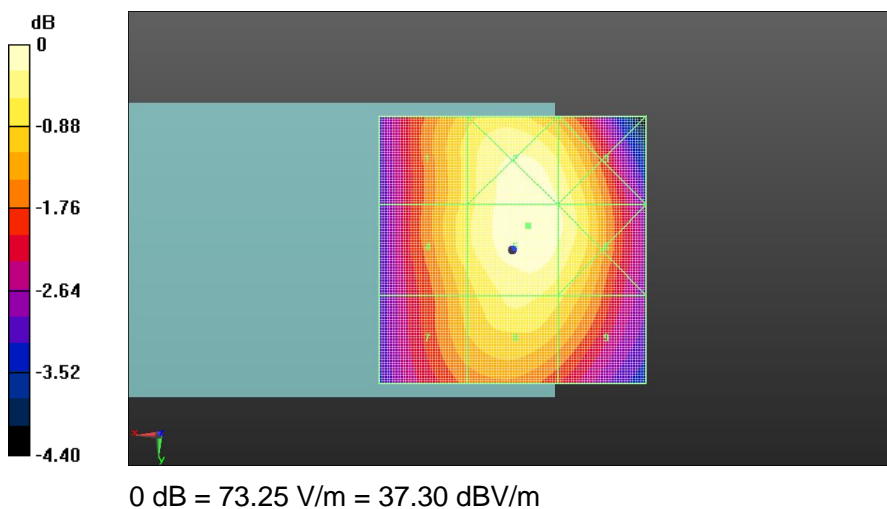
Fig A.2 HAC RF E-Field GSM 850 Middle
