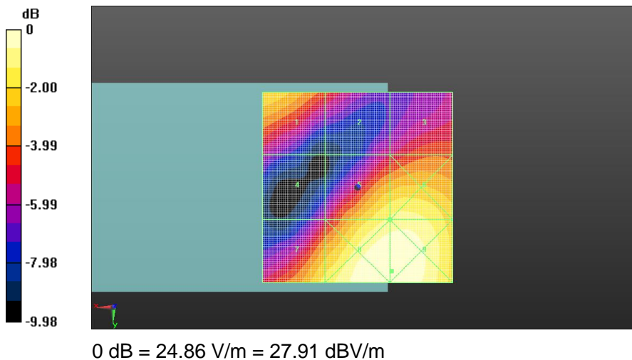
Fig A.5 HAC RF E-Field GSM 1900 Middle
