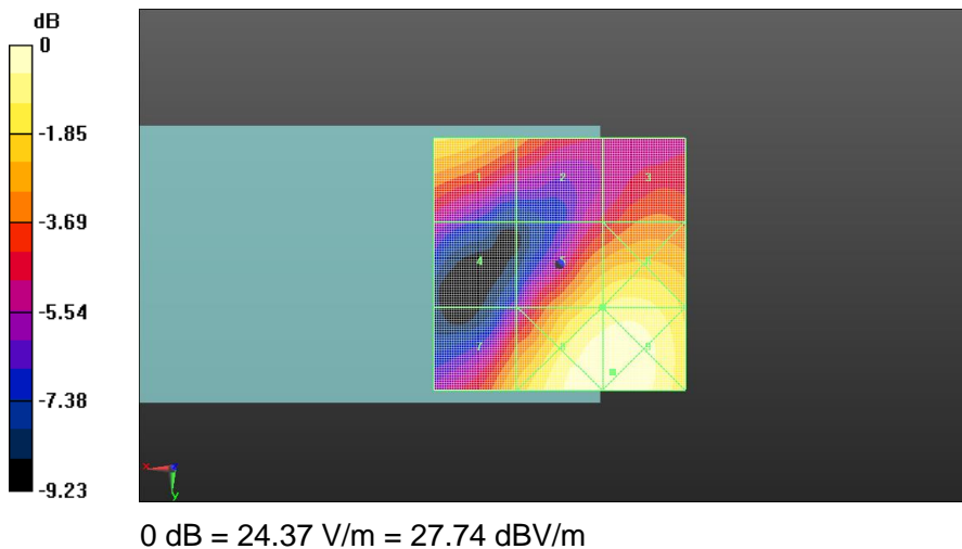
Fig A.4 HAC RF E-Field GSM 1900 High
