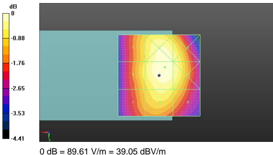
Fig A.1 HAC RF E-Field GSM 850 High
