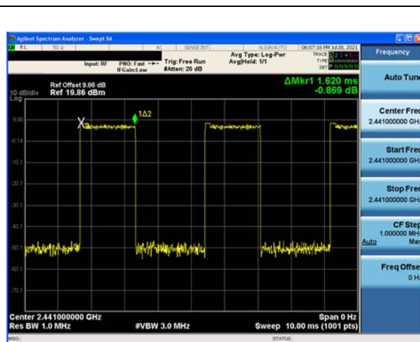
Modulation: 8DPSK 3DH3 2441
