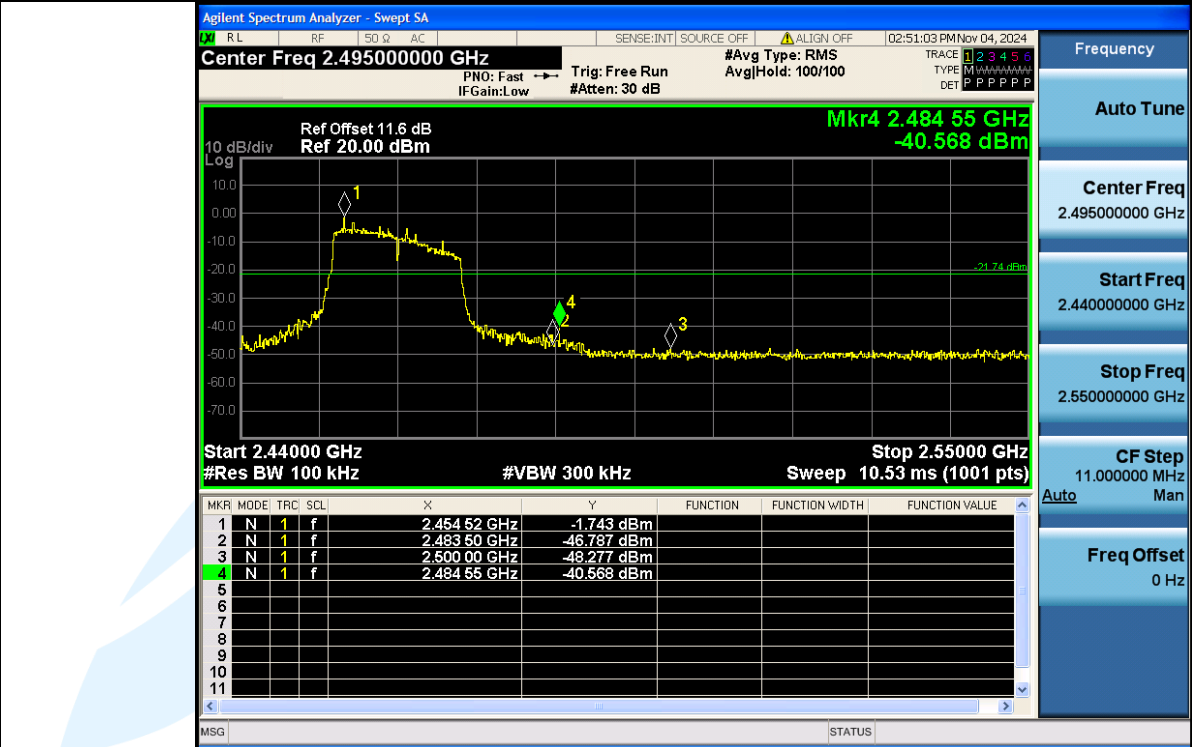
11N20SISO-Ant1-2462-PASS
