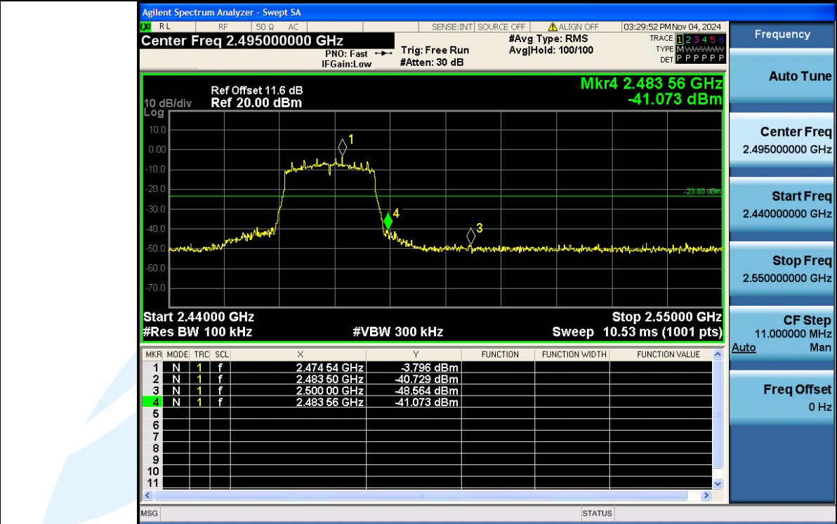
11N20SISO-Ant1-2472-PASS
