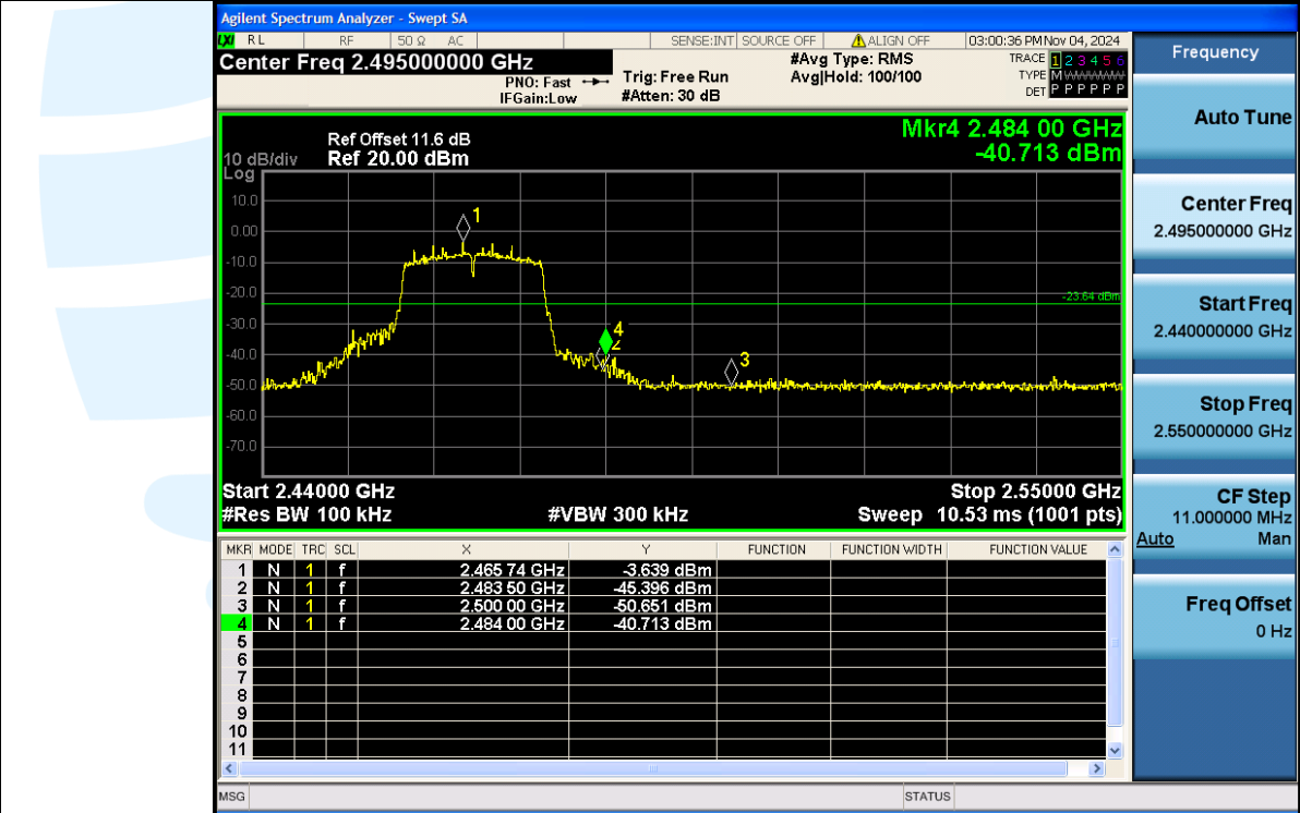
11N20SISO-Ant1-2467-PASS
