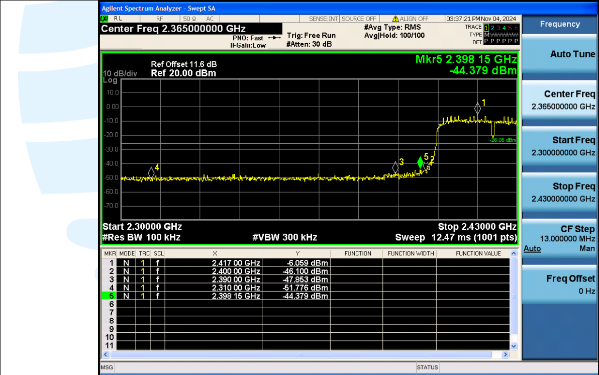
11N40SISO-Ant1-2422-PASS
